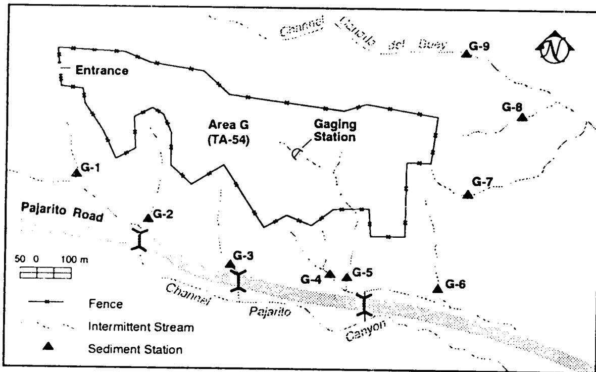
Fig. IV-10. Sediment sampling locations on and near solid waste management areas. a. Upper map shows the location of experimental areas and sediment stations at TA-49, Area AB. b. Bottom map shows the locations of alluvium sampling stations at TA-54, Area G.
