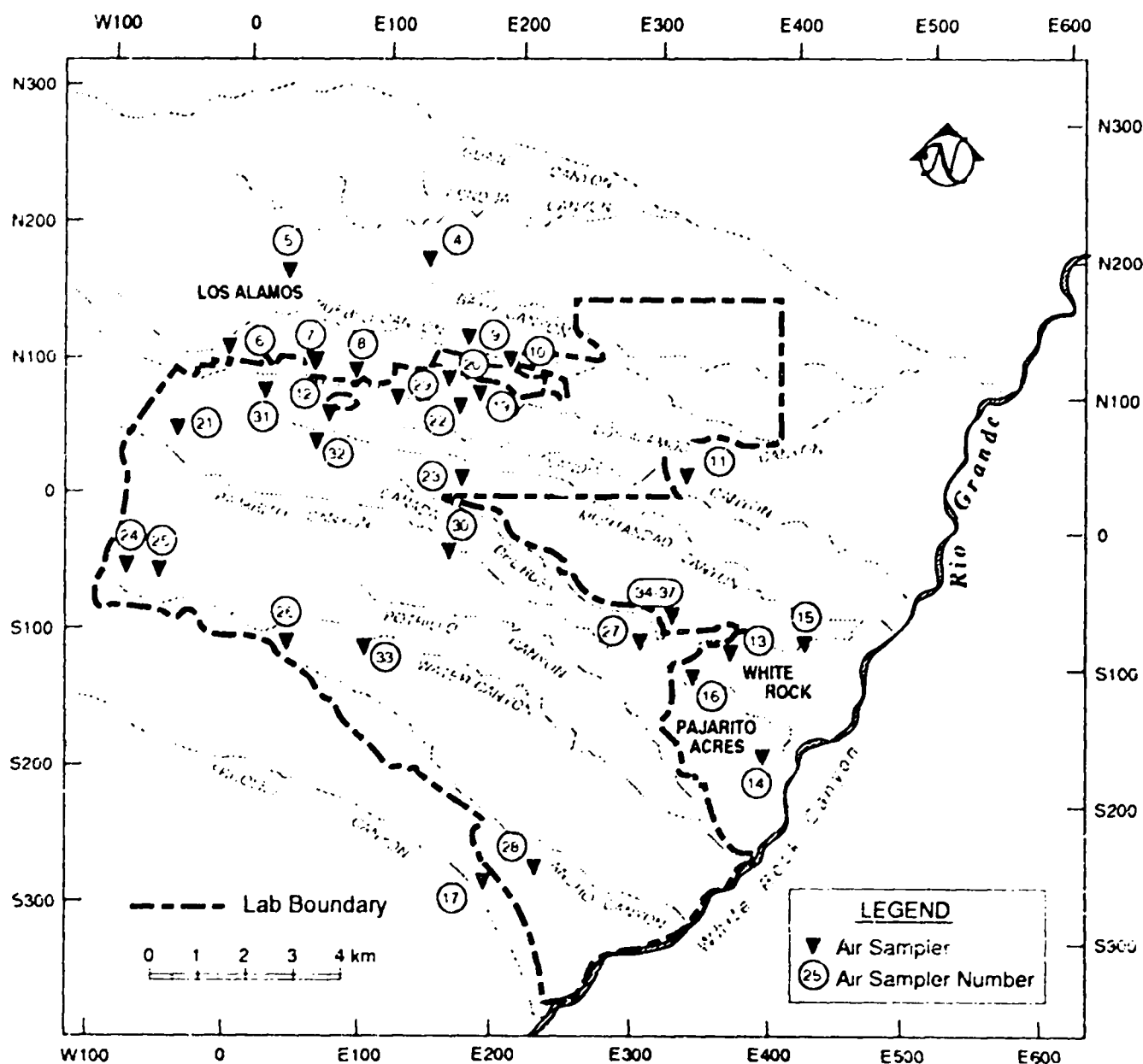
Fig. IV-4. Approximate locations on or near the Laboratory site for sampling airborne radionuclides. (Does not show Regional Stations; specific locations are presented in Table D-8.)
