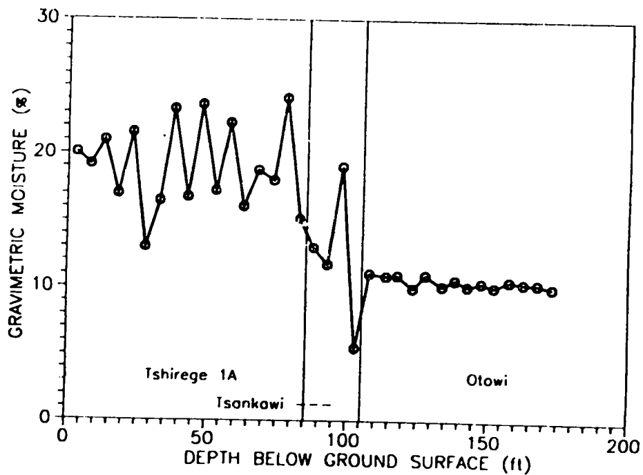
Fig. VII-6. Potrillo Canyon Core Hole No. 1 on December 12, 1991.
