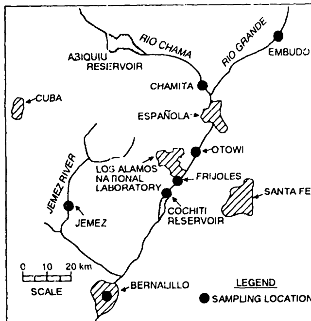
Fig. IV-5. Regional surface water, sediment, and soil sampling locations. (Map denotes general locations only; see Table D-9 for specific locations.)
