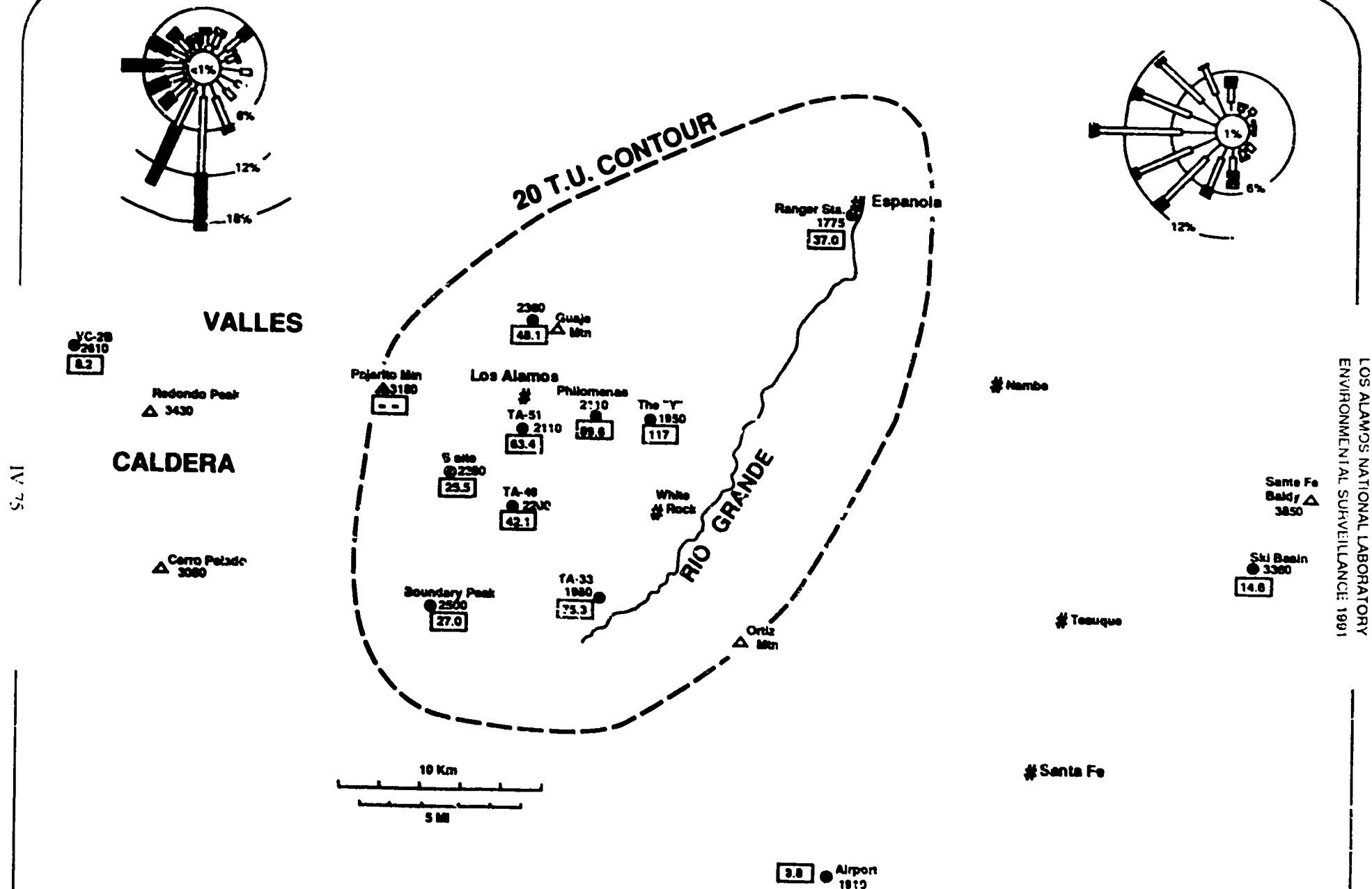
Fig. IV-16. Tritium in rainwater (collected during December 1990 - April 1991).
