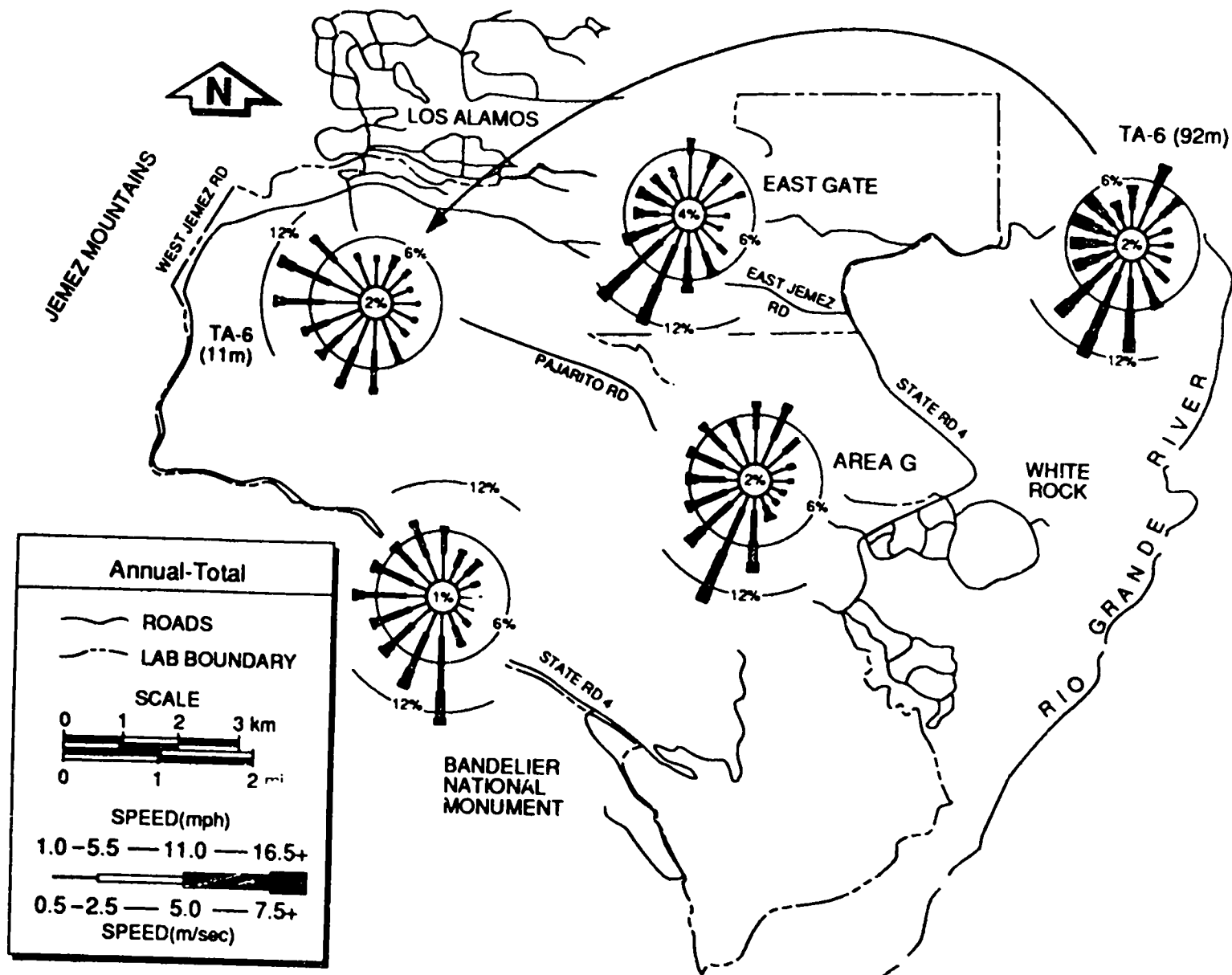
Fig. II-9. Average total wind roses at Laboratory stations. Surface winds are represented at TA-6 (upper left) clockwise to East Gate, Area G, and Band-lier. TA-6 winds at the 92 m (300 ft) level are also shown.
