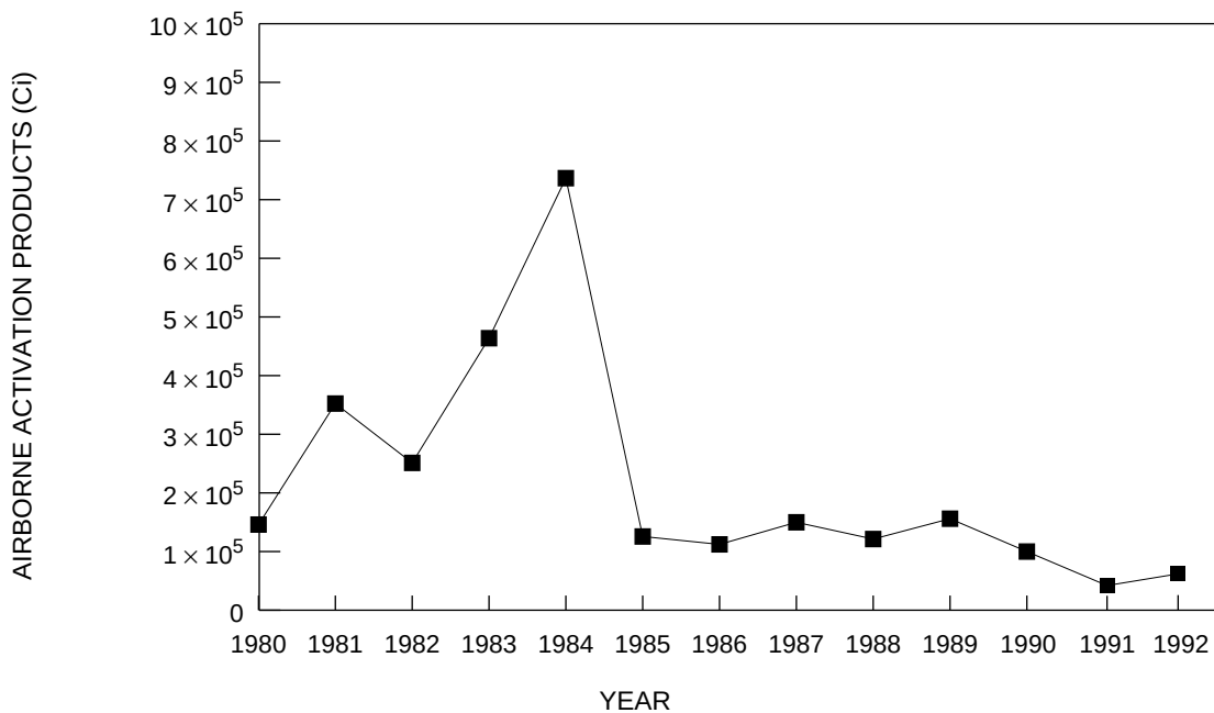
Figure V-3. Airborne activation product emissions (principally ^{10}\text{C} , ^{11}\text{C} , ^{12}\text{N} , ^{16}\text{N} , ^{14}\text{O} , ^{15}\text{O} , ^{41}\text{Ar} ) from the Los Alamos Meson Physics Facility (TA-53).
