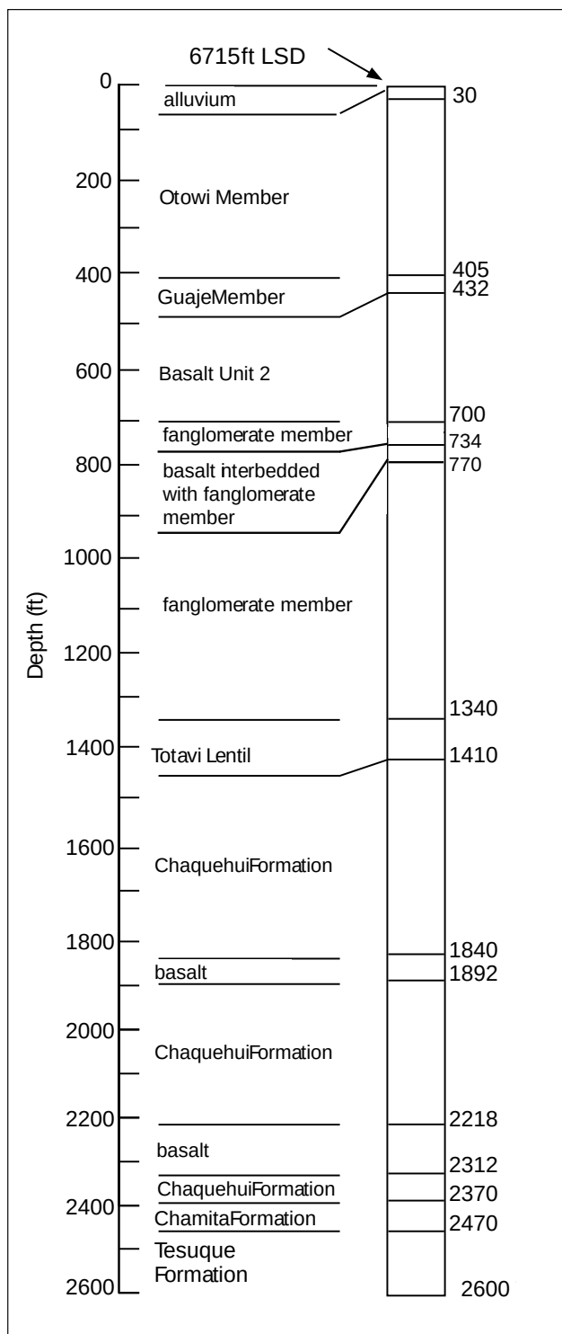
Figure E-16.1 Stratigraphy at well PM-2
