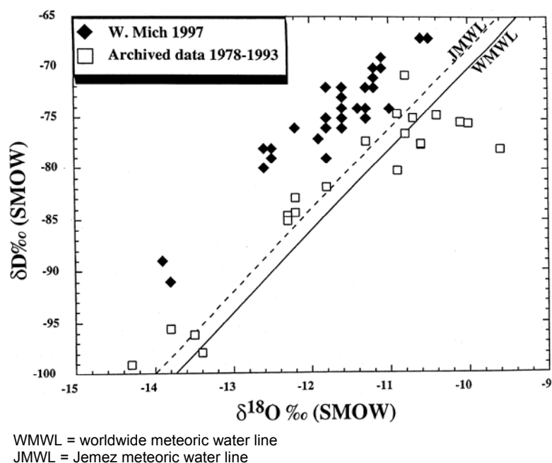
Figure F-2.3-1. Comparison of archived stable isotope data with University of Western Michigan 1997 data
