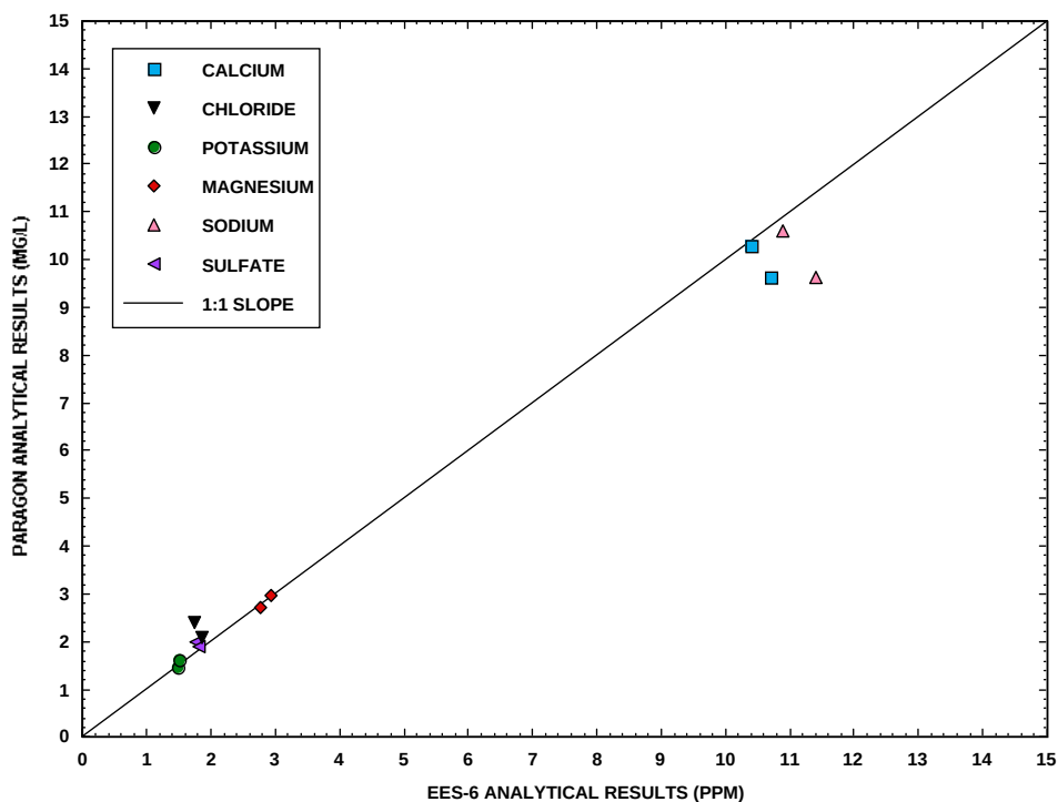
Figure F-4-4. Comparison of major ion chemistry (dissolved) reported by EES-6 and Paragon Analytics, Inc., for Doe Spring (basalt) sampled in February and September 1998
