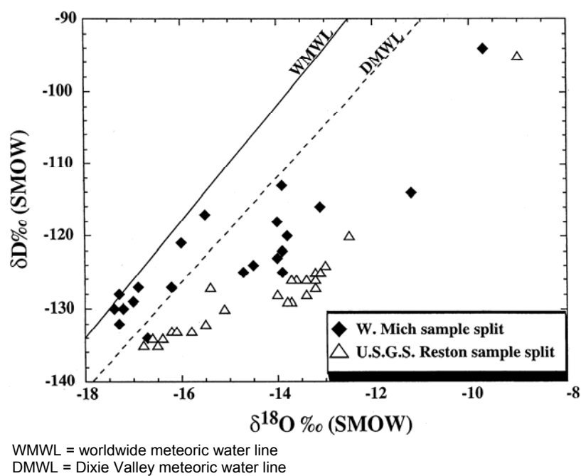
Figure F-2.3-2. Laboratory comparison of sample splits from Dixie Valley, Nevada (Goff et al. 2002, 88776)
