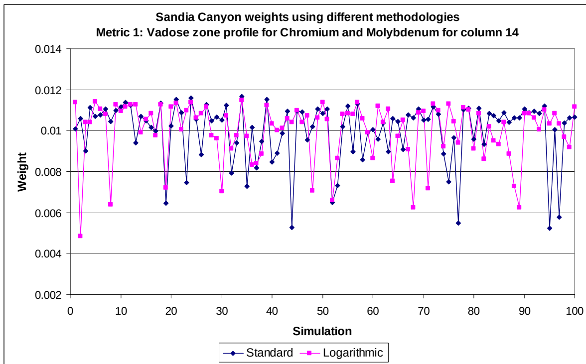
Figure G-7 Weights for the vadose zone for Cr and Mo at column 14
