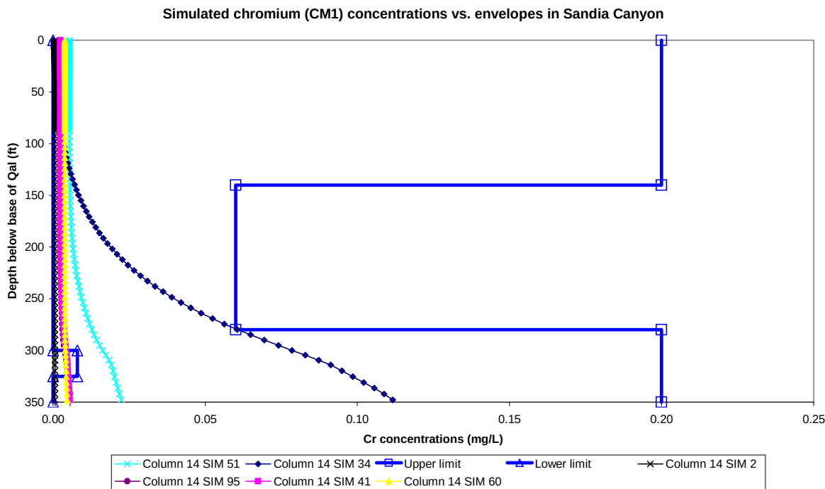
Figure G-8 Comparison between Cr concentrations and envelopes for the best (#51, #34), worst (#95, #2), and average (#60, #41) simulations
