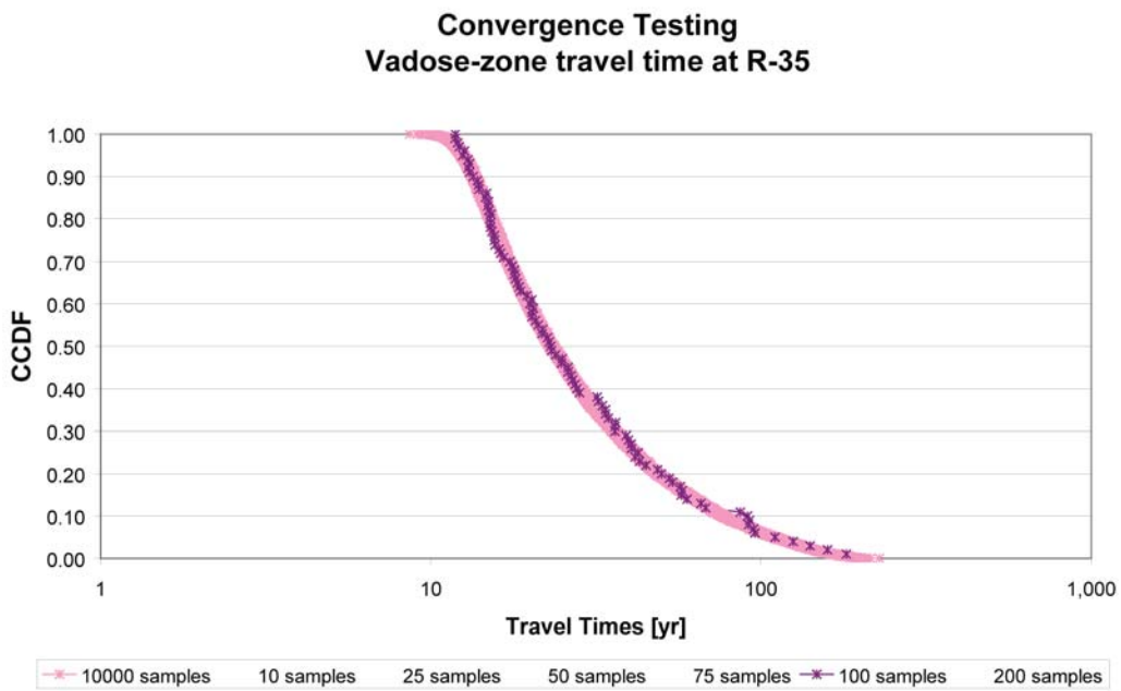
Figure F-4 Distribution of vadose-zone travel times for 100 and 10,000 realizations
