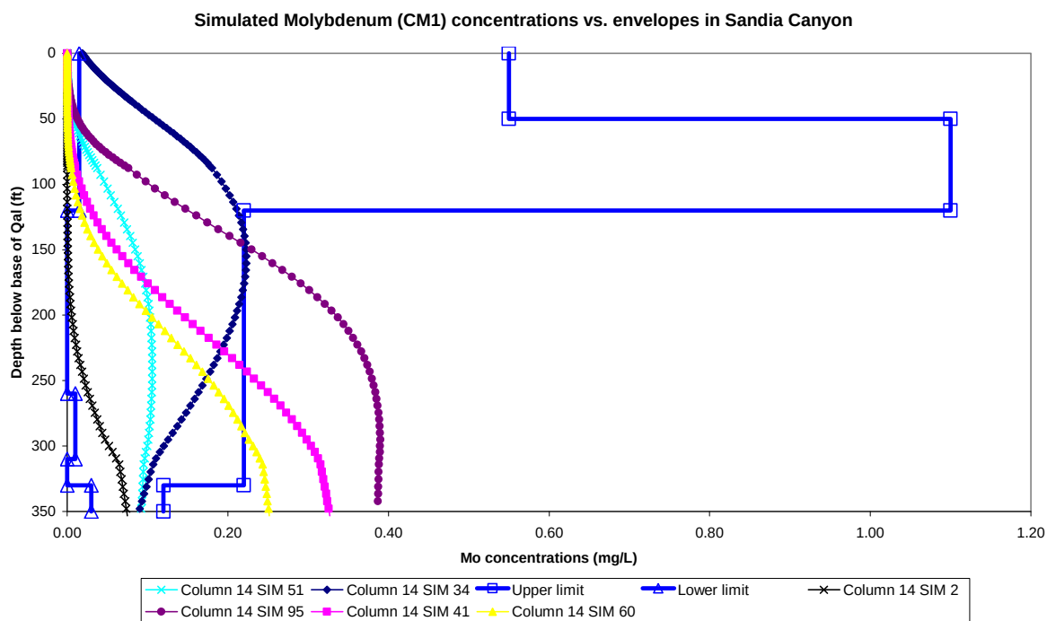
Figure G-9 Comparison of Mo concentrations with envelopes for the best (#51, #34), the worst (#95, #2), and the average (#60, #41) simulations with respect to weighting of results
