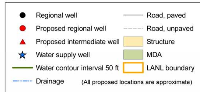
Figure 5.0-1 Location of TA-54: MDAs H, L, and G including the existing water-supply wells and regional wells; proposed locations for new wells and water-table contours
