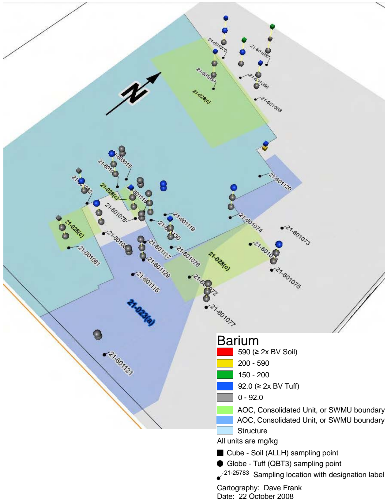
Figure C-10 Distribution of barium at AOC 21-028(c)
