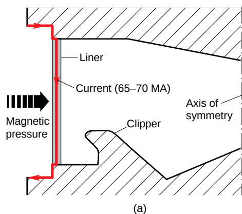
Figure 17. Generation of a Plasma Bubble
