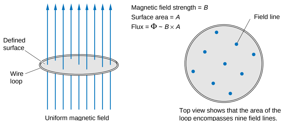
Figure 2. Magnetic Flux
