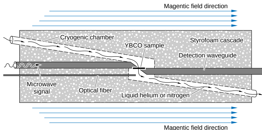
Figure 11. Schematic of the Critical-Field Experimental Setup
