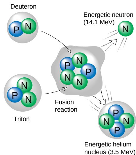
Figure 13. Thermonuclear Fusion Einstein’s famous equation, E = mc^2 , relates mass to energy. The sum of the deuteron and triton rest masses at the start of the fusion reaction is actually more than the sum of the alpha particle and neutron rest masses after the reaction has finished. As a result of fusion, some mass is converted into energy, and that energy is imparted to the reaction products. Both the alpha particle and the neutron emerge from the fusion event with a significant amount of kinetic energy.
