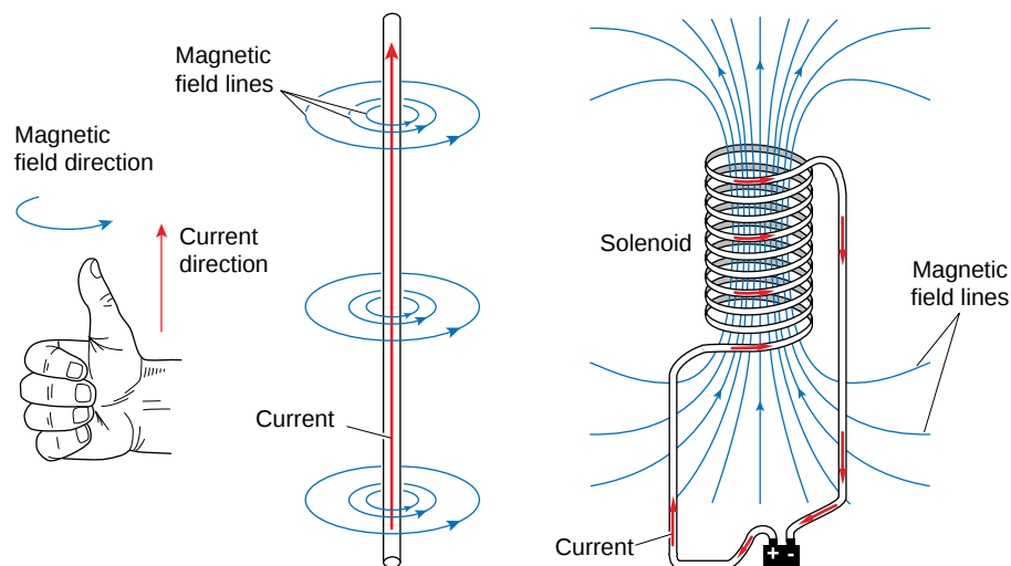
Figure 1. Magnetic Fields and Electrical Currents
