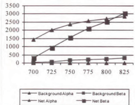
Voltage Plateau
