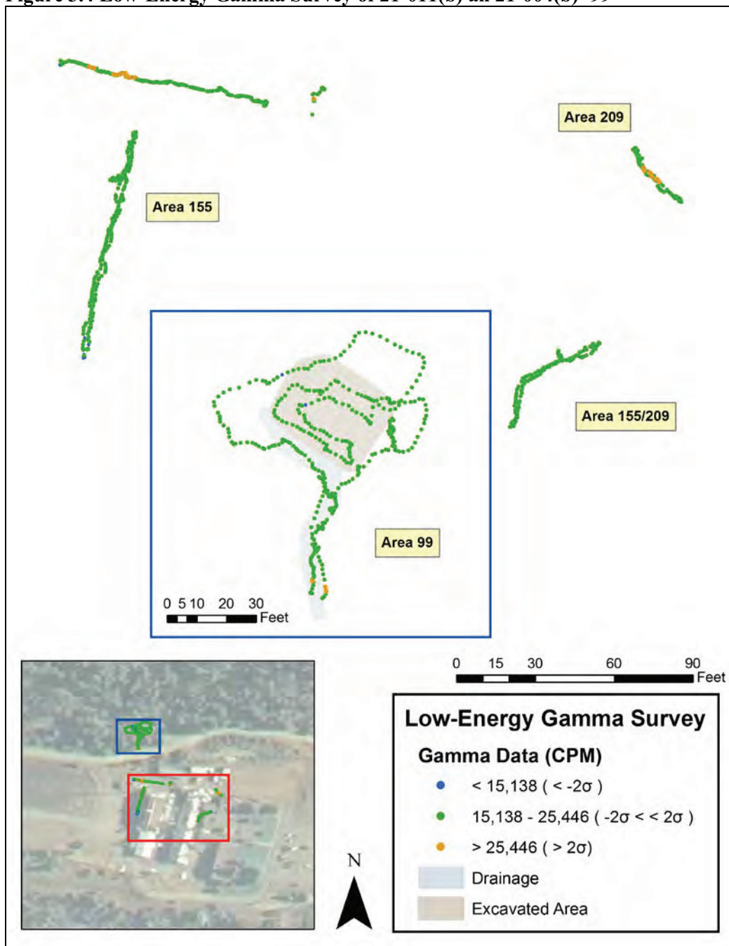
Figure 3.4 Low-Energy Gamma Survey of 21-011(b) and 21-004(b) -99
