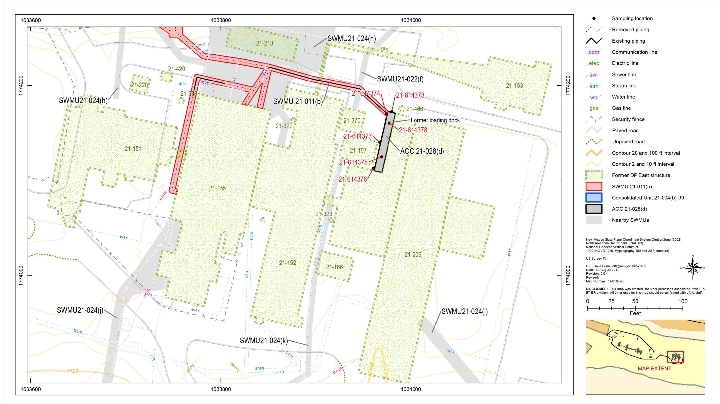
Figure 2.7-1 AOC 21-028(d) former loading dock site map with sampling locations
