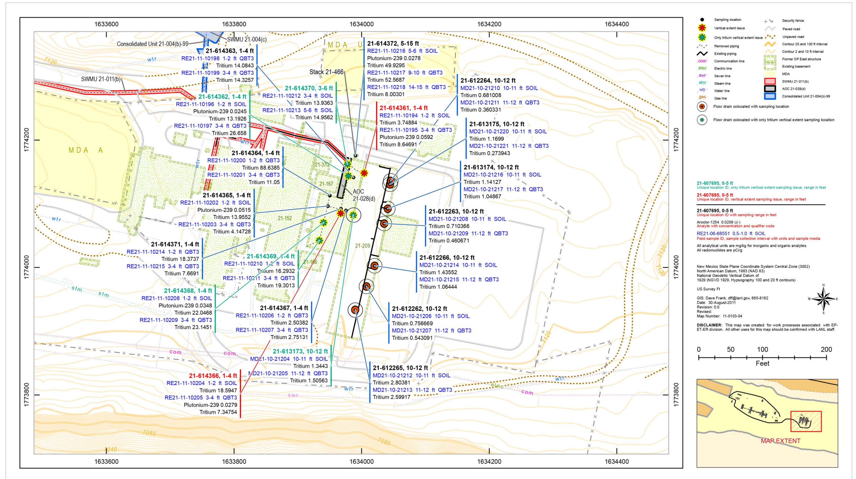
Figure 7.1-5 Radionuclides detected or detected above BVs/FVs at former building 21-209 and associated former structure 21-466 footprints
