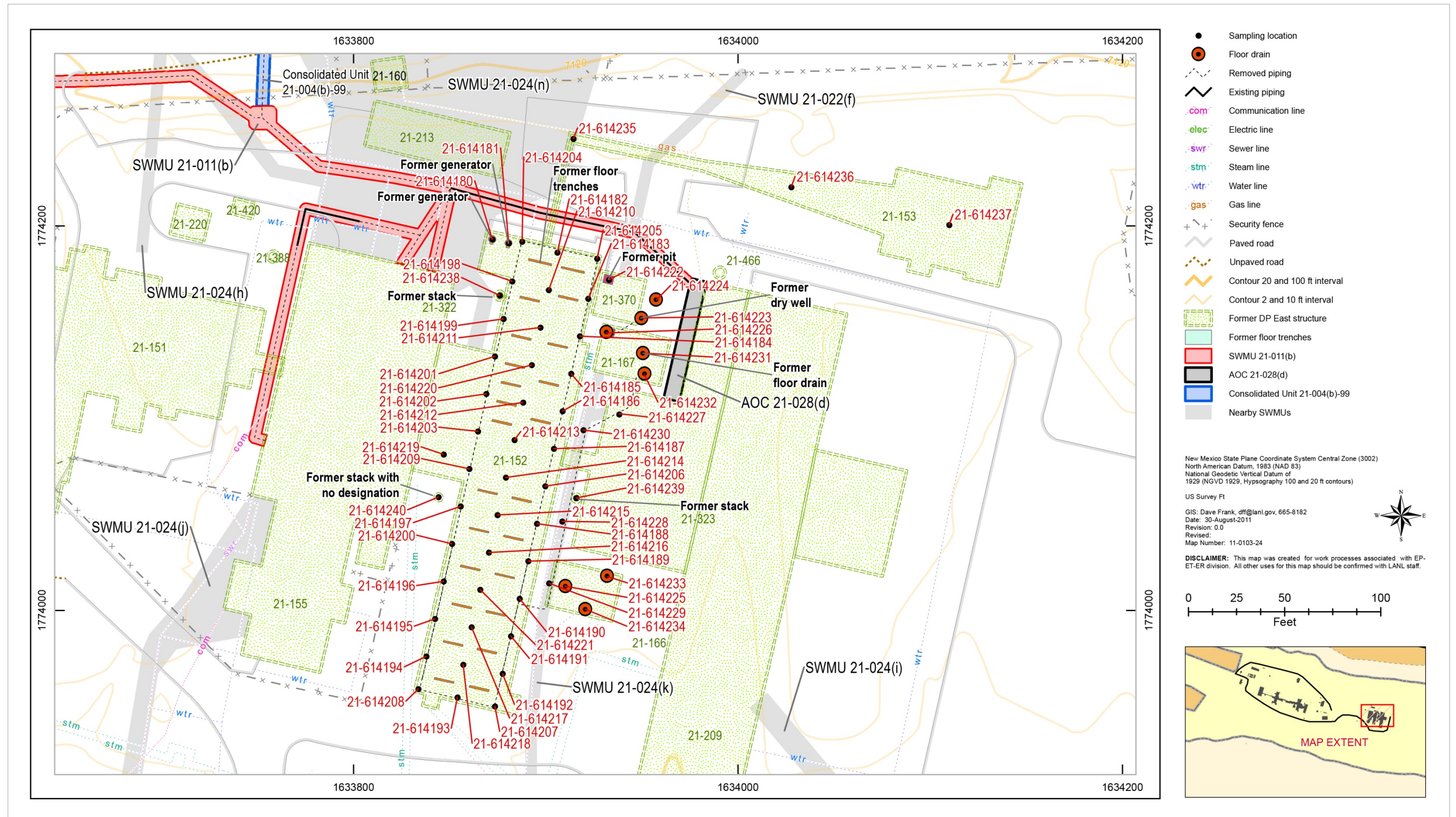
Figure 2.4-1 Former building 21-152 and associated former structures footprints site map with sampling locations
