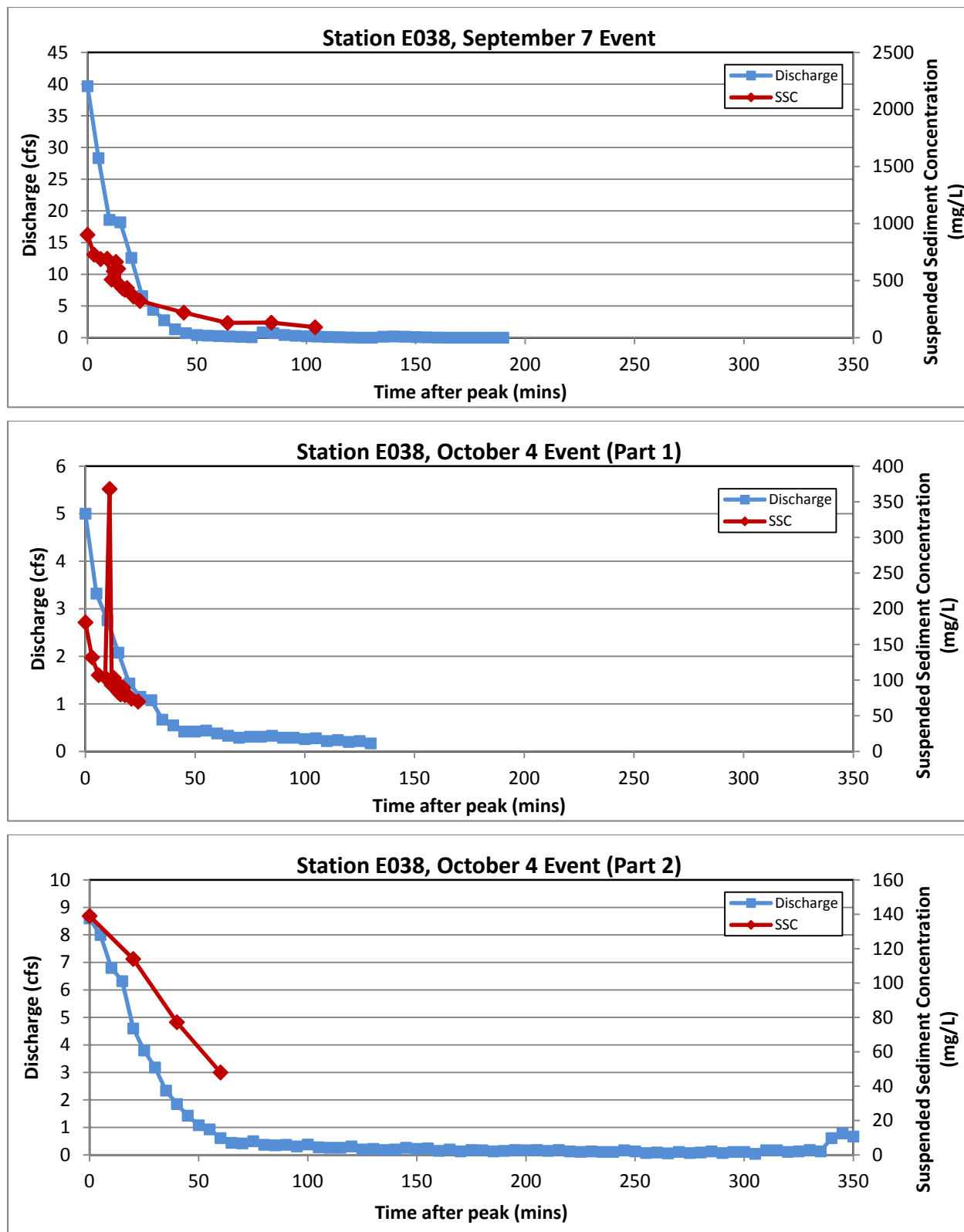
Figure 3.2-4 (continued) Discharge and SSC for sampled events at E038, E039.1, E042.1, E050.1, and E109.9
