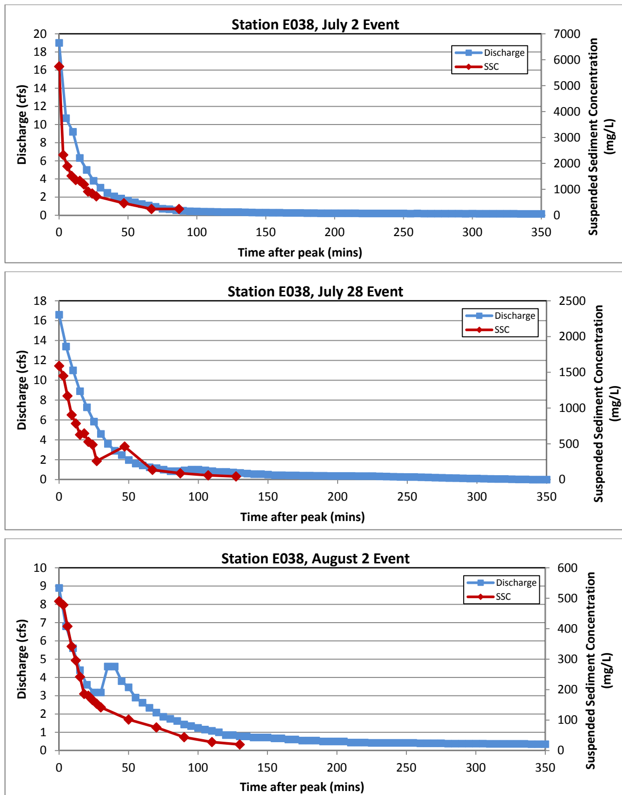
Figure 3.2-4 Discharge and SSC for sampled events at E038, E039.1, E042.1, E050.1, and E109.9
