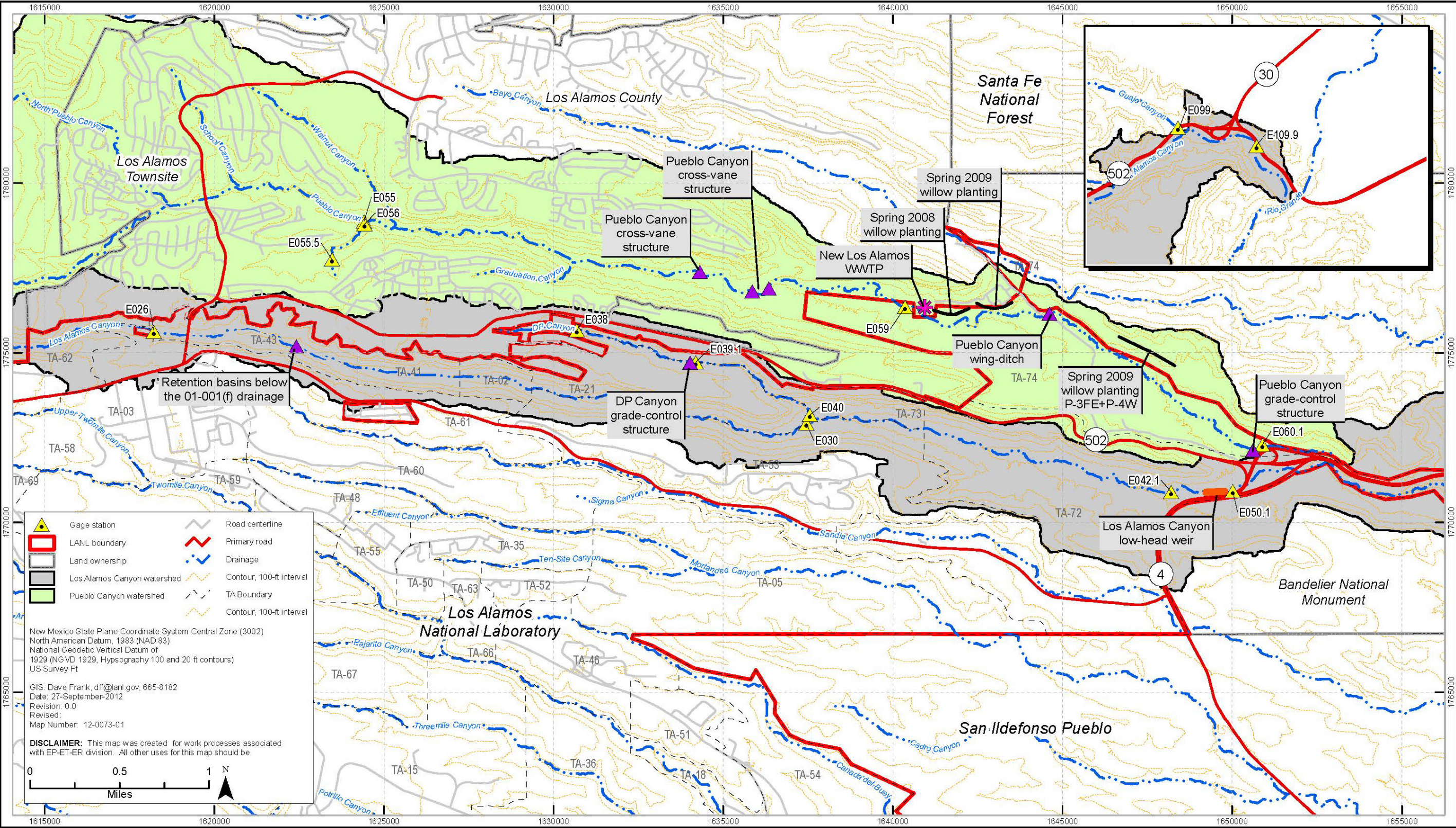
Figure 1.0-1 Los Alamos and Pueblo Canyons showing monitoring locations and sediment transport mitigation sites
