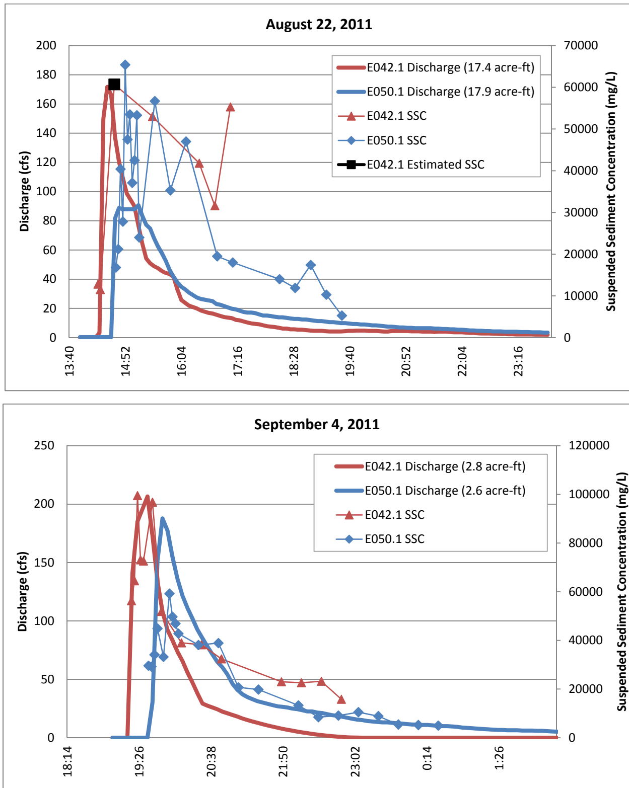
Figure 3.3-2 Discharge and SSC at E042.1 and E050.1 in upper Los Alamos Canyon on days when sampling of the same runoff event occurred
