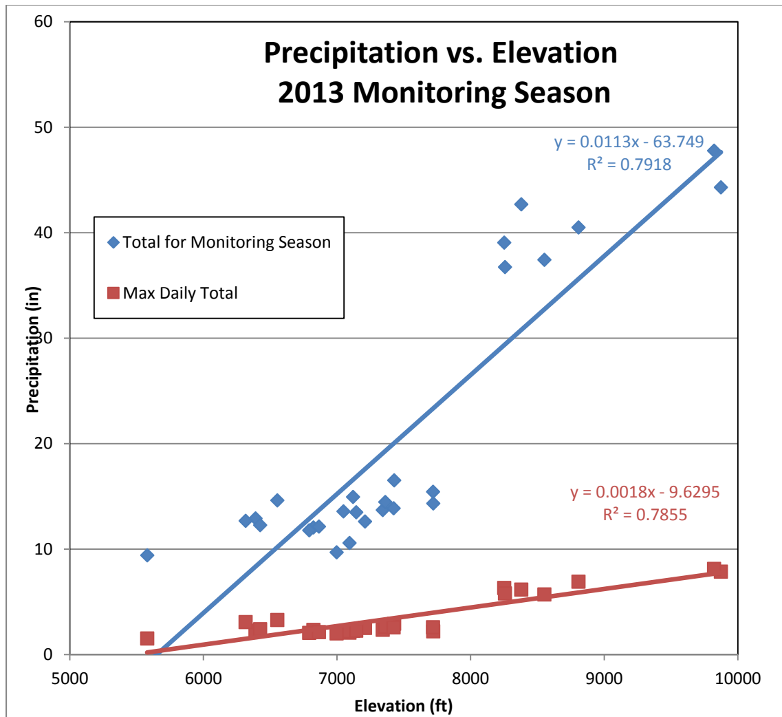
Figure 9 Total annual precipitation and maximum daily total precipitation in relation to rain gage elevation for 2013 monitoring season, May 1 to October 31, 2013
