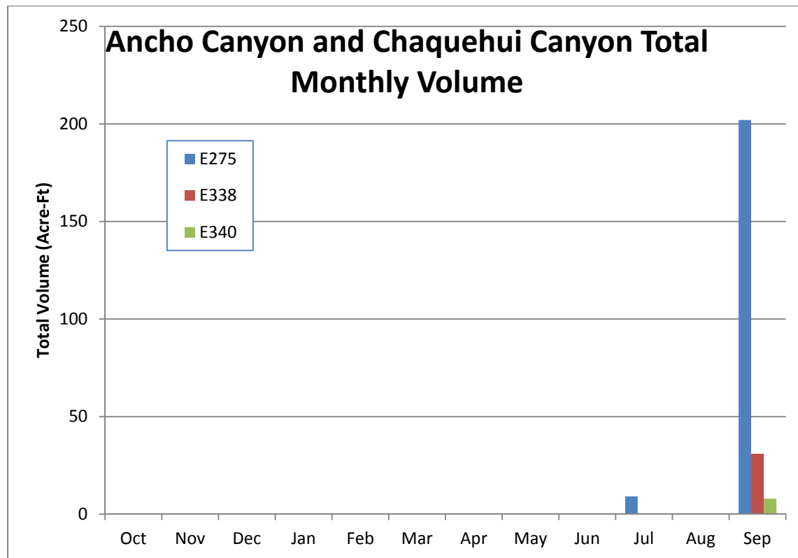
Figure 8 Total monthly volume (acre-ft) for WY2013 in Ancho Canyon and Chaquehui Canyon
