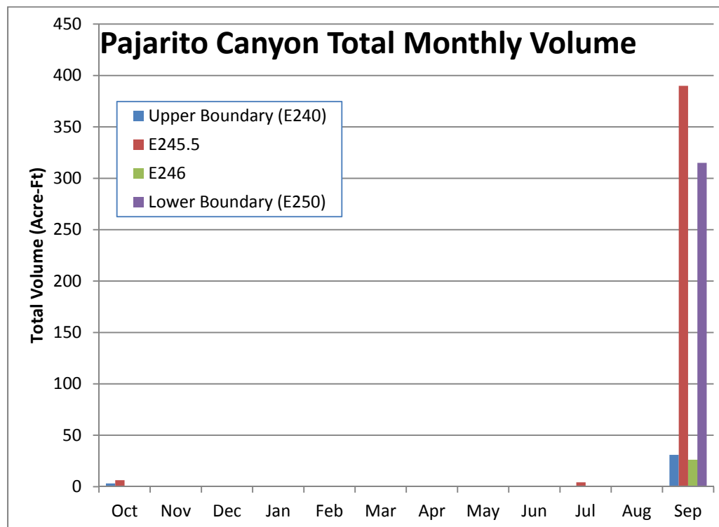
Figure 6 Total monthly volume (acre-ft) for WY2013 for Pajarito Canyon
