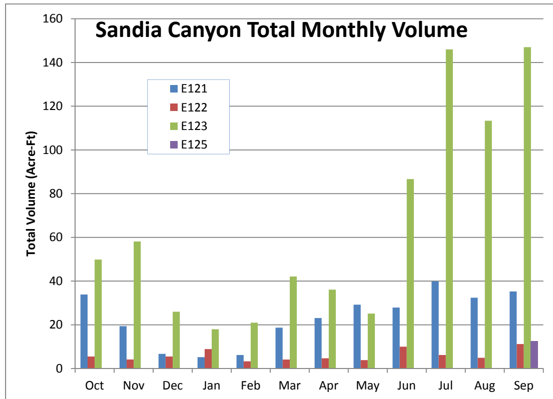
Figure 4 The total monthly volume (acre-ft) for WY2013 for Sandia Canyon
