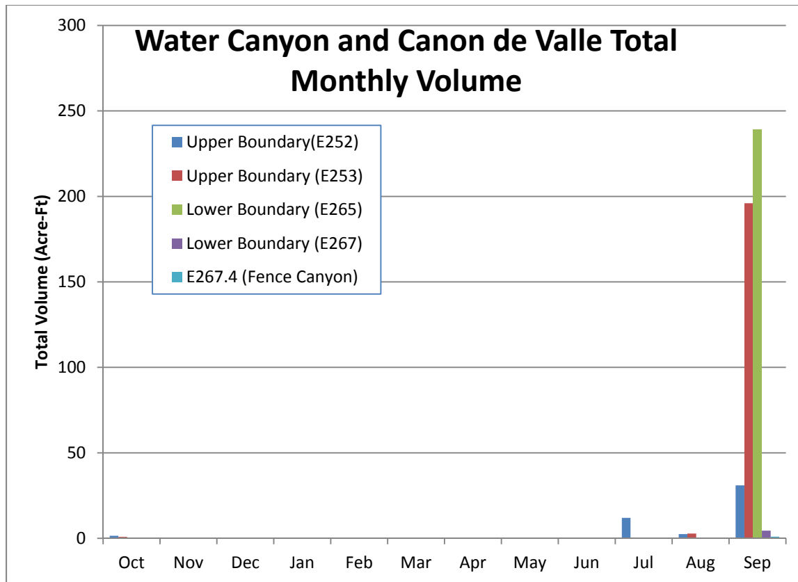
Figure 7 Total monthly volume (acre-ft) for WY2013 in Water Canyon, Cañon de Valle, and Fence Canyon
