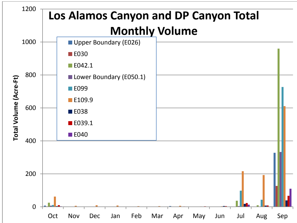
Figure 2 The total monthly volume (acre-ft) for WY2013 for Los Alamos Canyon and DP Canyon
