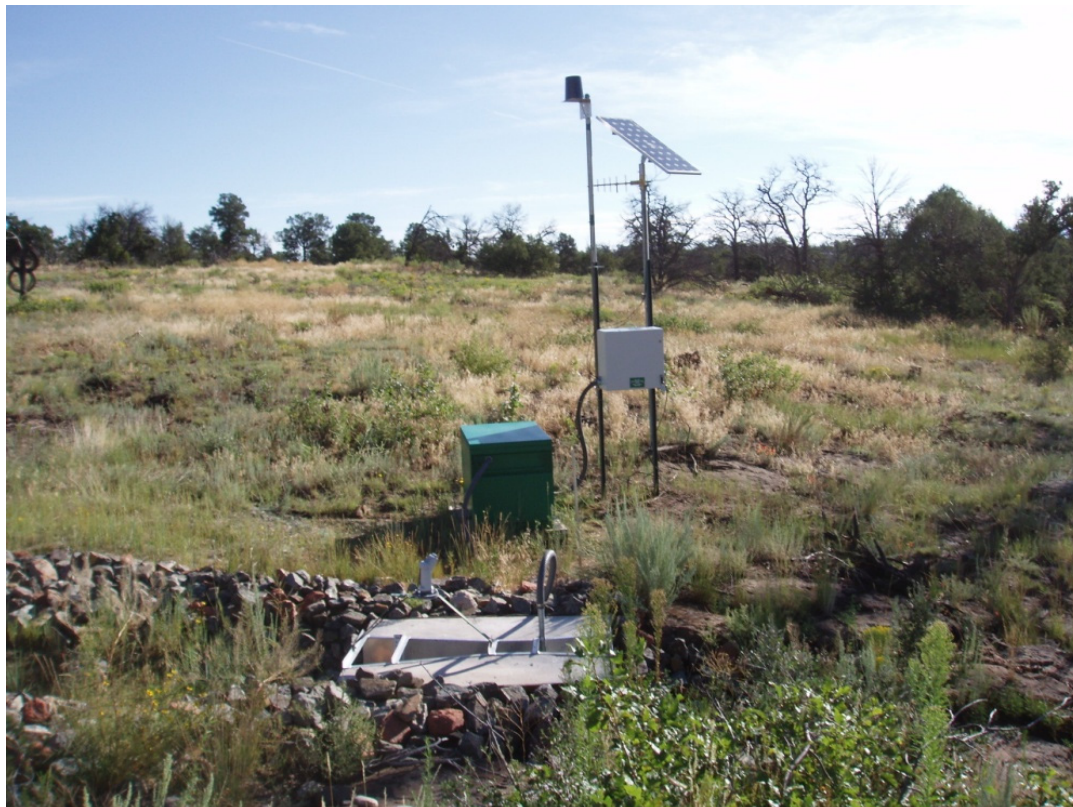
E267.4 View across stream gage, downstream to the right
