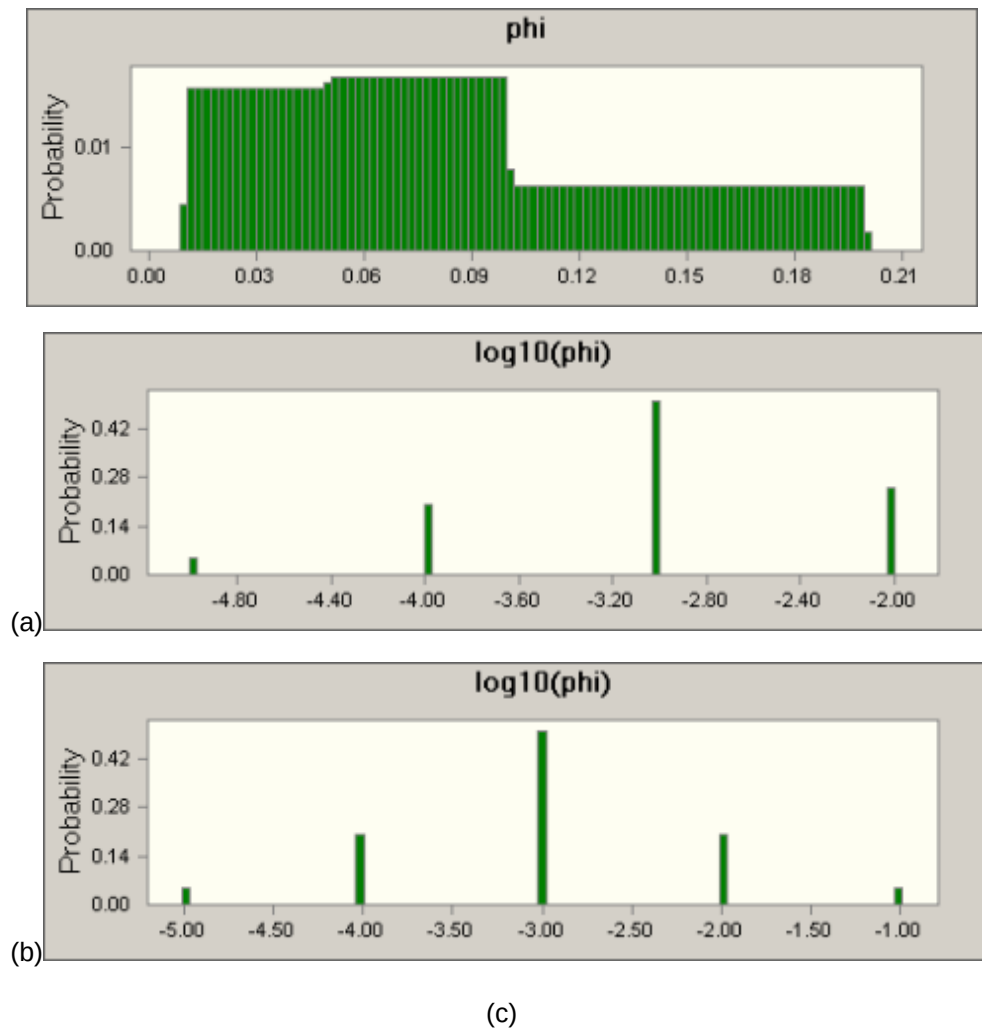
Figure C-4 Probability distributions of effective porosity for different hydrostratigraphic units: (a) Totavi Lentil, Pumiceous Puye, Puye Fanglomerate, Santa Fe Fanglomerate, Santa Fe Silt and Sands; (b) Tschicoma, Keres Group; and (c) Cerros del Rio Basalt, Bayo Canyon Basalt. The distributions are defined predominantly based on data from the literature (Freeze and Cherry 1979, 088742); the only site-specific data that are available are for the Cerros del Rio Basalt (Tb4) and Puye Fanglomerate (Tpf), and these data were considered in developing the distributions for those two units (Keating et al. 2001, 095399).
