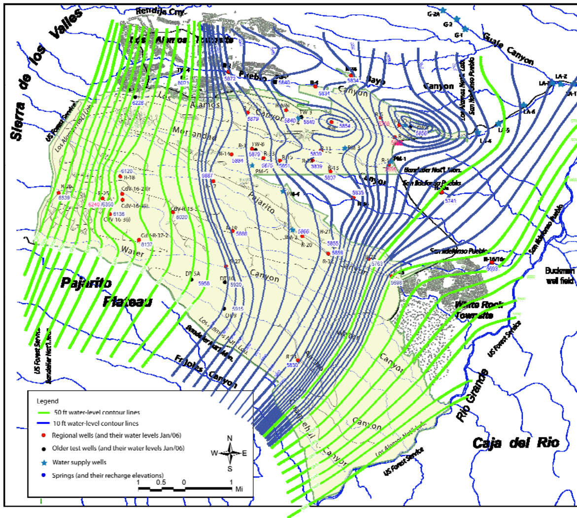
Figure C-2 Water-table map characterizing the flow direction in the phreatic zone of the regional aquifer
