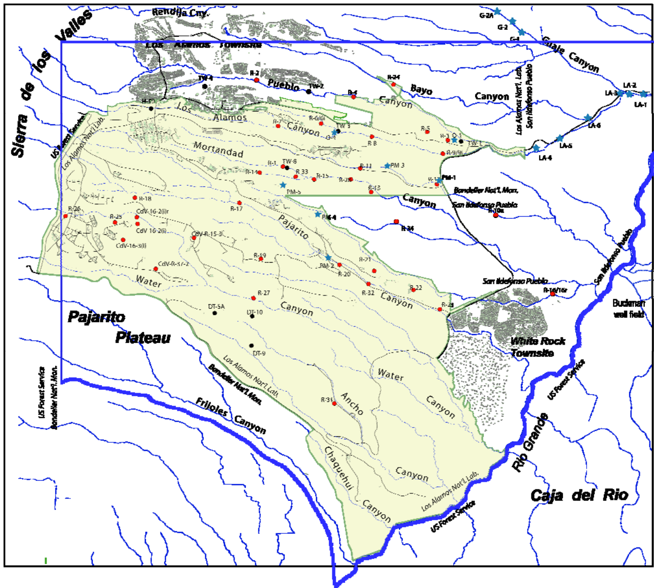
Figure C-1 Domain of the regional-aquifer numerical model used for the wells assessments
