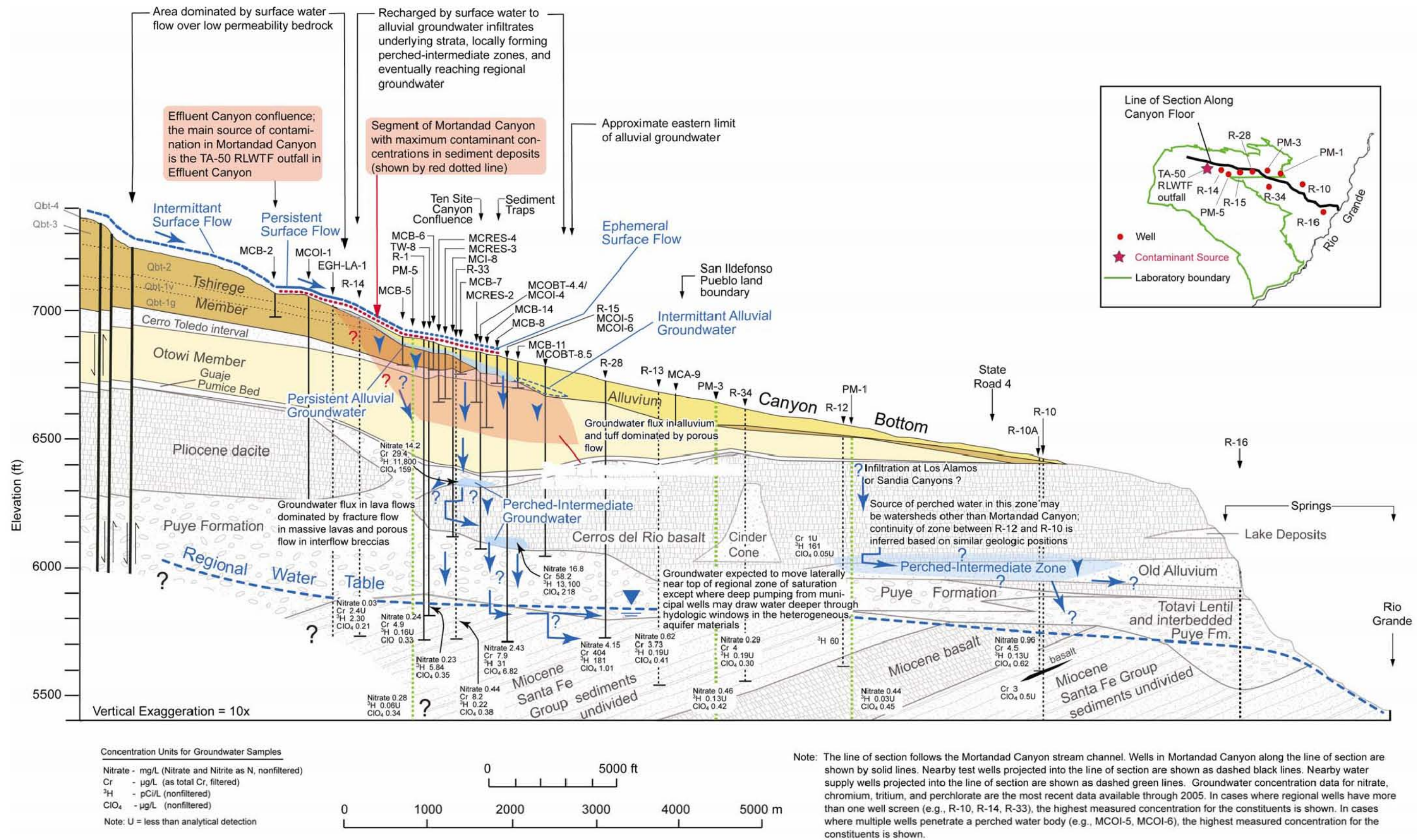
Figure 2-2 Conceptual hydrogeologic cross section showing potential contaminant transport pathways
