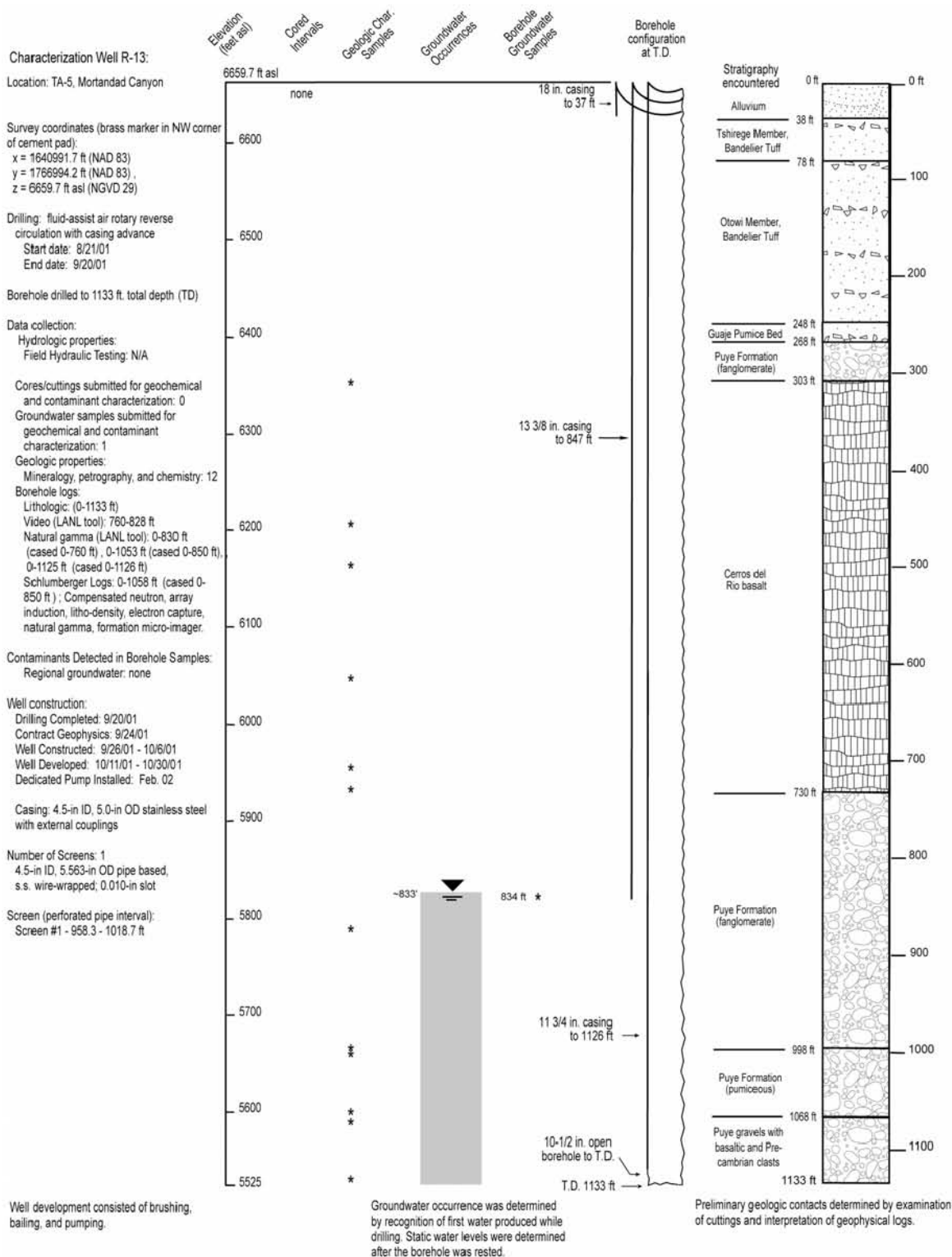
Drilling, stratigraphic, and hydrologic information for characterization well R-13 Rev. 0 (2/25/02)
