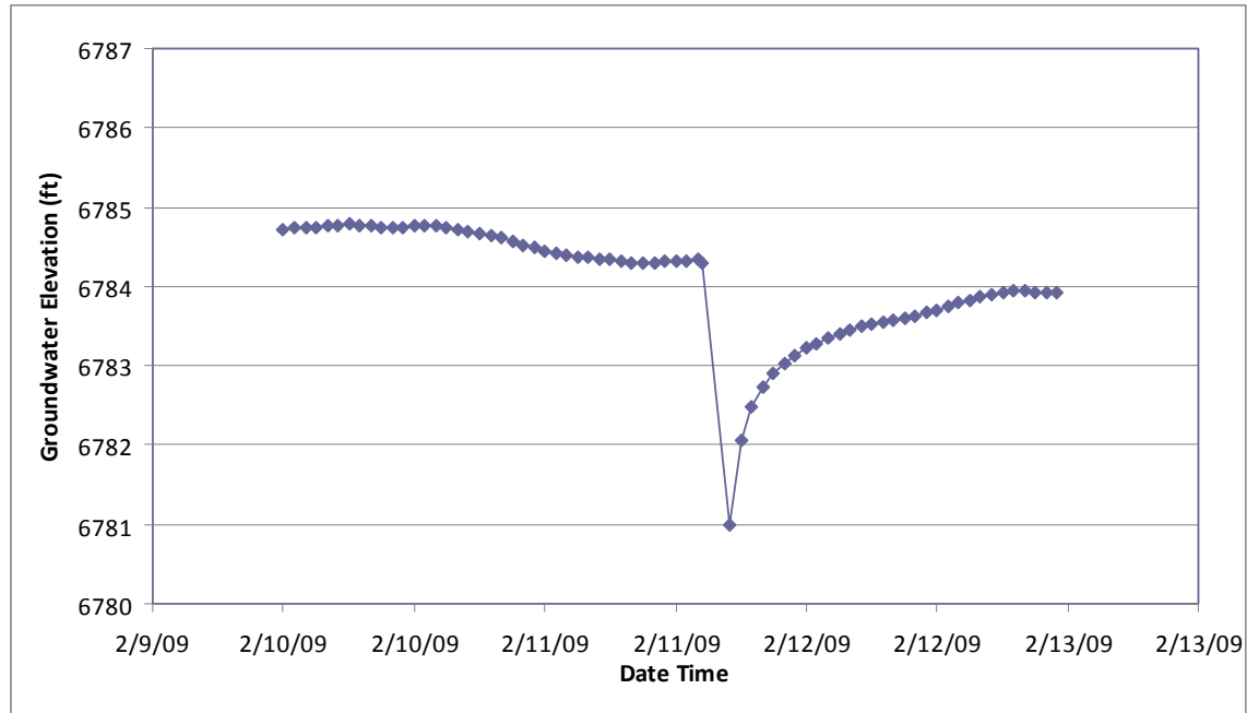
Figure B-2.0-1 Water-level data for CDBO-6 directly before and after the 2/11/09 sampling event
