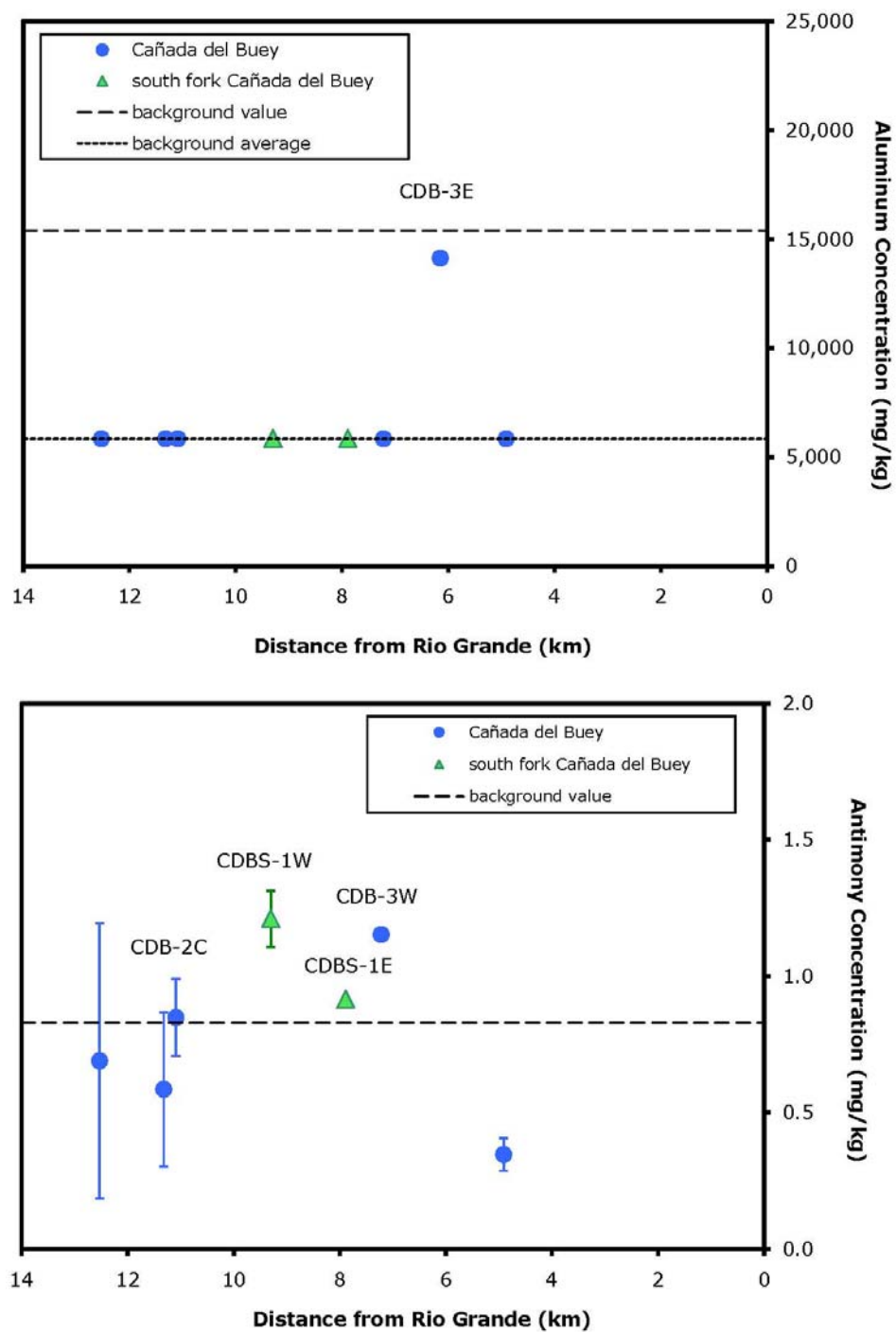
Figure 7.1-1 Estimated average concentrations of select inorganic chemicals in fine facies sediment in Cañada del Buey
