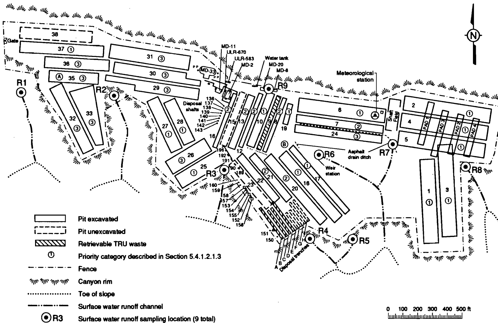
Figure 5.4-6 Surface water runoff sampling locations at MDA G.
