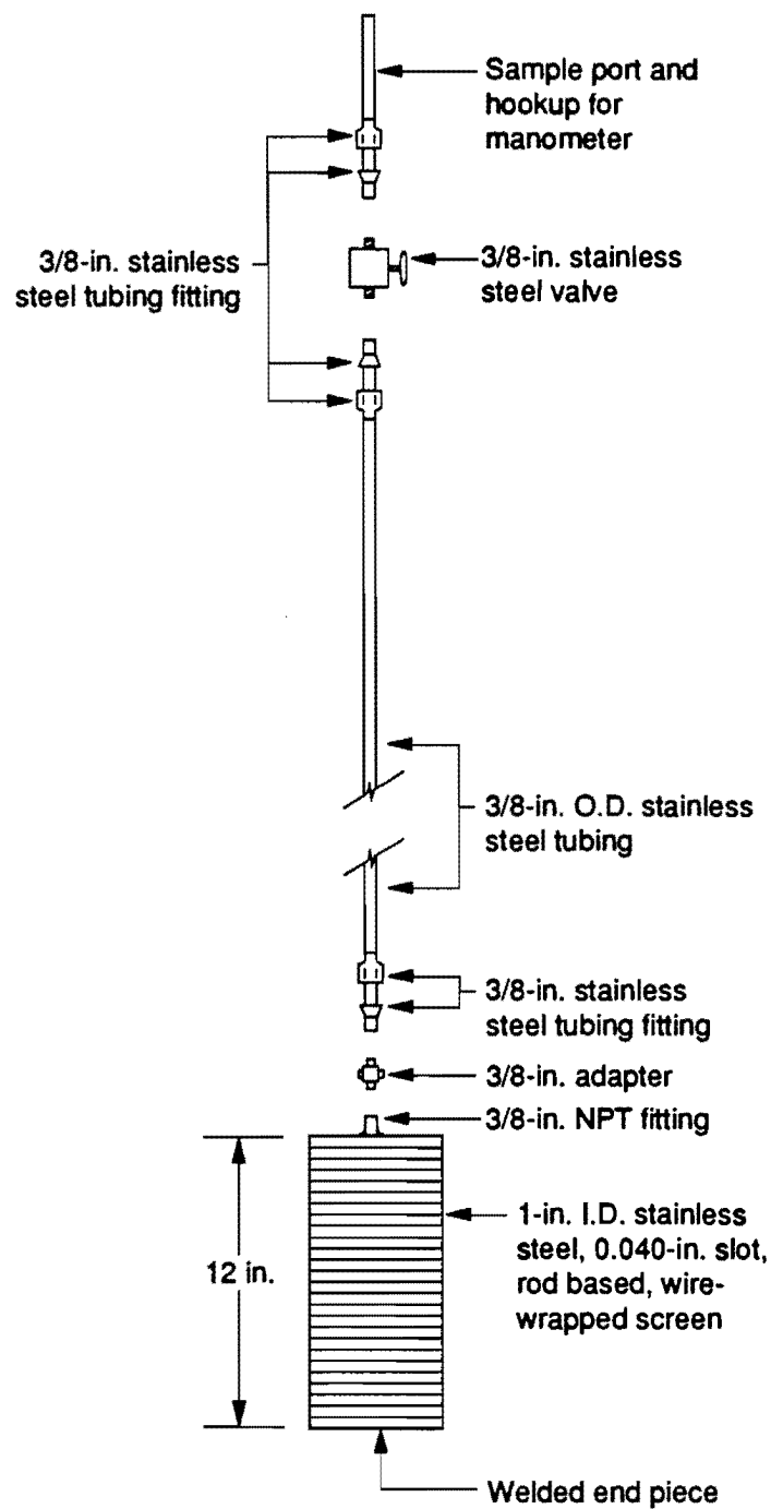
Figure A-14B Vapor monitoring probe construction (not to scale).
