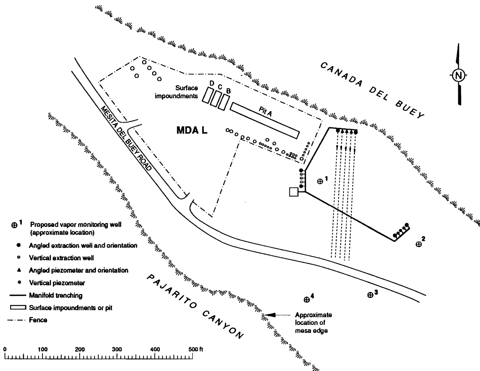
Figure A-12 Locations for extraction wells and piezometers with trench and blower/treatment system. (Base map modified from IT Corp. 1987 and 1991.)
