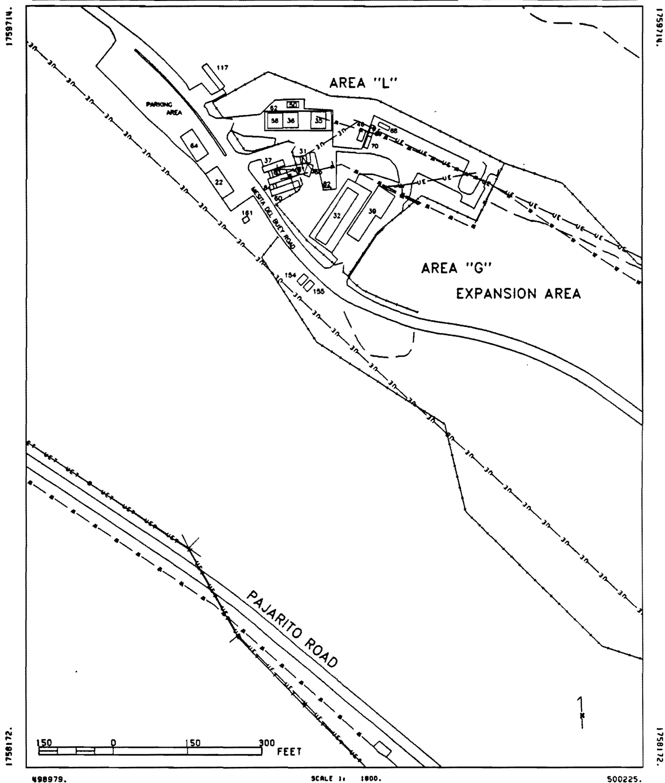
Figure III-2 Utilities Servicing MDA I.
