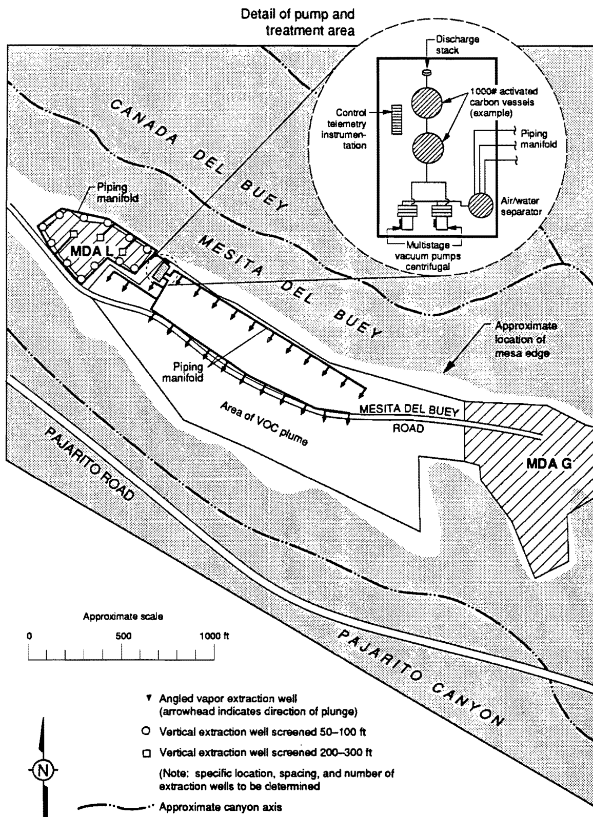
Figure A-11 Conceptual configuration of vapor extraction system.
