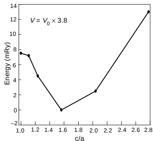
Figure 10. Calculated Total Energy of Aluminum as a Function of Orthorhombic Shear
