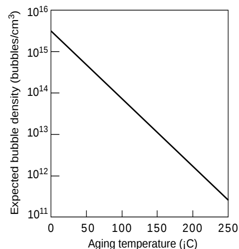
Figure 4. Estimate of the Helium Bubble Density
