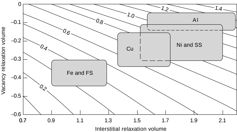
Figure 8. Net Bias for Radiation-Induced Void Swelling Dislocations attract and absorb self-interstitials slightly more than vacancies. The different rate of absorption is known as the net bias, \Delta B , and is the fundamental driving force for void swelling. The contour lines are lines of constant net bias value as indicated. The boxes circumscribe the range of predicted values for the net bias using measured relaxation volumes and their uncertainties. The materials are aluminum (Al), nickel and austenitic stainless steels (Ni and SS), copper and copper-nickel alloys (Cu), and body-centered-cubic iron and ferritic steels (Fe and FS).
