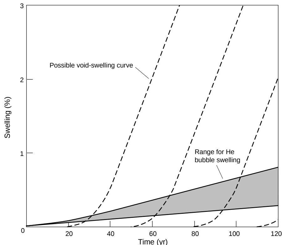
Figure 9. Predictions for Radiation-Induced Damage in Plutonium
