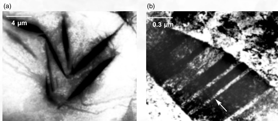
Figure 1. Direct Observation of Martensites in Pu-Ga Alloy (a) A TEM image shows \alpha' -plates (dark phase) inside the \delta -phase of a Pu-3.4 at. % Ga alloy. The sample was cooled to low temperature to transform martensitically to the monoclinic \alpha' -phase. Note the crystallographically distinct orientations of the martensite plates. (b) At higher magnification, twin boundaries (one perpendicular to arrow) can be seen within an individual plate. (This figure was reproduced courtesy of Acta Metall. Mater. )
