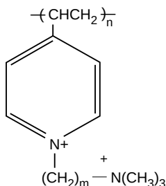
(c) Trimethylammonium
