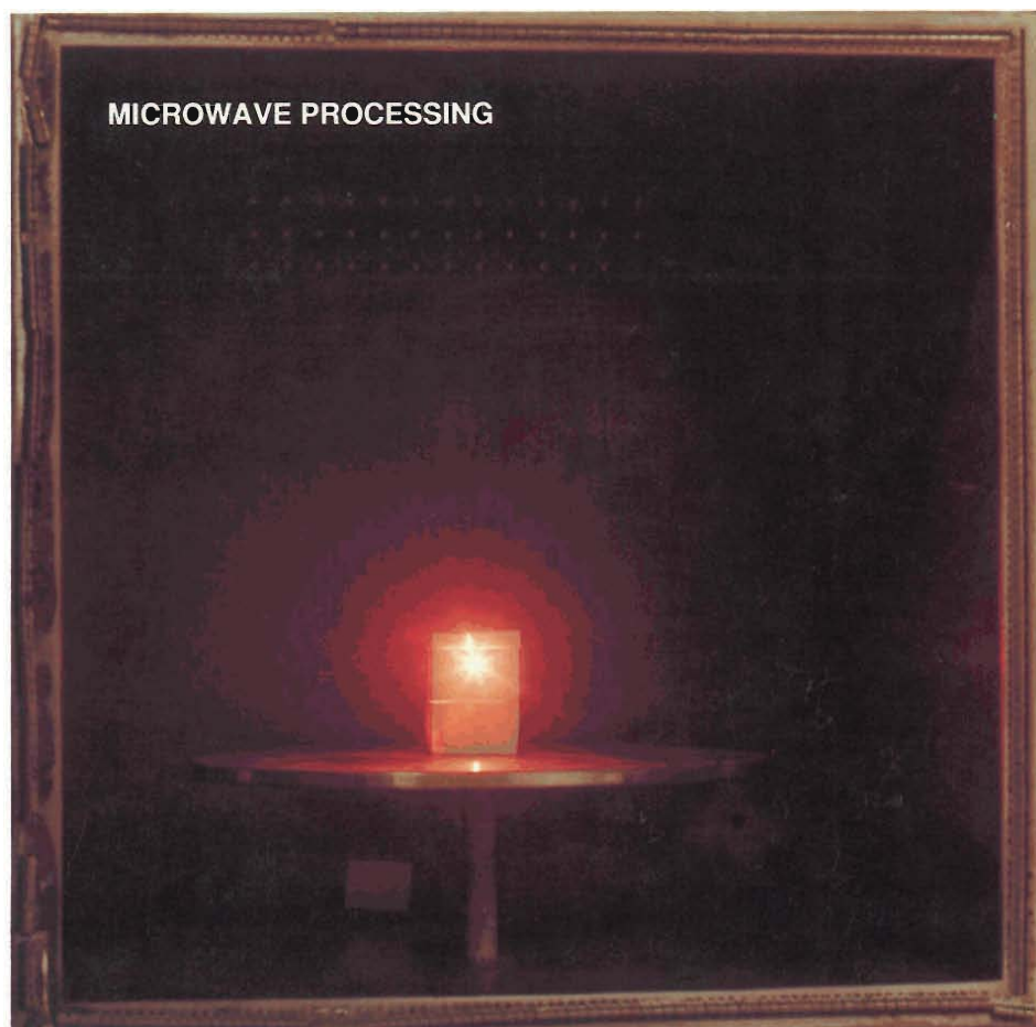
Fig. 11. A sample of boron carbide is rapidly sintered in a microwave oven to produce a fine-grained ceramic with a density that is close to the theoretical maximum.
