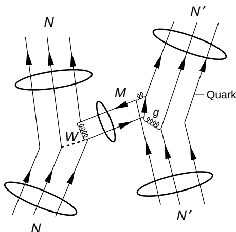
Figure 8. The Nucleon-Nucleon Weak Interaction at the Quark Level
