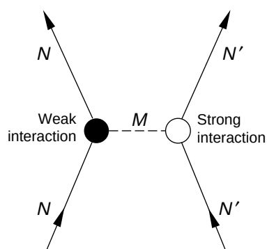
(a) Nucleon-Nucleon Weak Interaction Showing Meson ( M ) Exchange.
