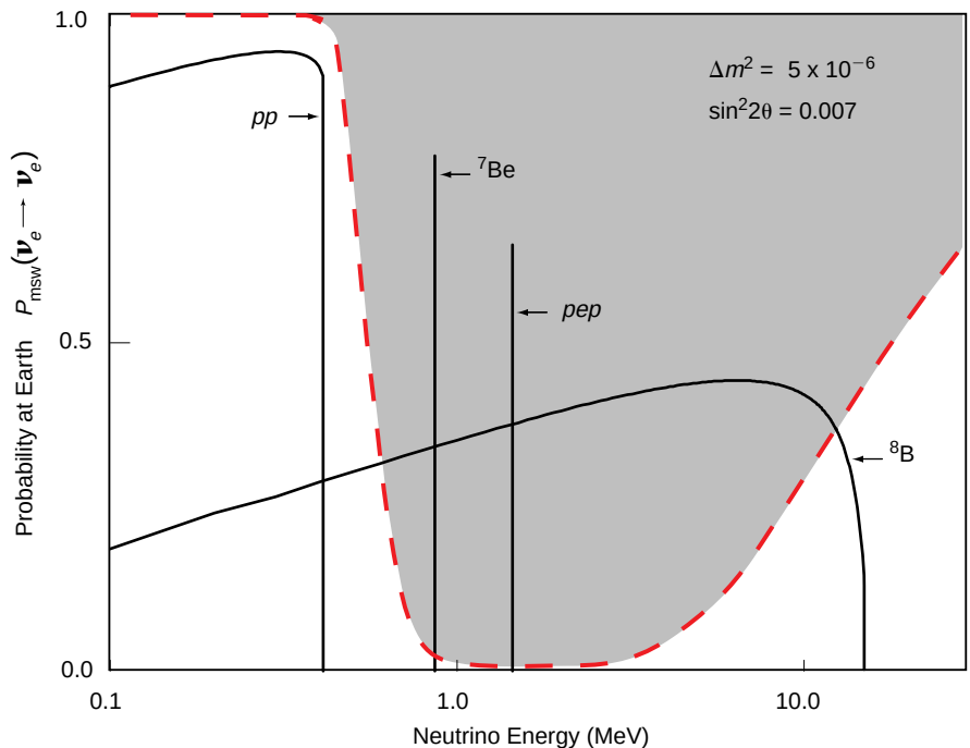
Figure 3. MSW Solution to the Solar-Neutrino Problem The MSW survival probability P_{\text{MSW}}(\nu_e \rightarrow \nu_e) (red dashed line) has been plotted as a function of neutrino energy and superimposed over a simplified picture of the solar-neutrino spectrum. Solar neutrinos with energies that fall within the gray-shaded region (those from the {}^7\text{Be} , pep , and {}^8\text{B} reactions) have a low survival probability, and thus have a high probability of oscillating into muon and/or tau neutrinos as they flee the solar core. If the MSW effect occurs in the Sun, experiments that detect only electron neutrinos would measure a reduced flux from those reactions. An experiment such as the one planned at the Sudbury Neutrino Observatory, which is sensitive to electron, muon, and tau flavors, should detect the full flux.
