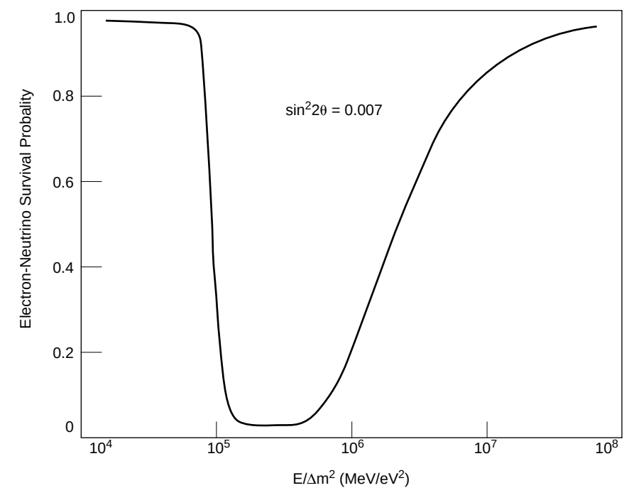
Figure 2. The MSW Survival-Probability Curve for the Sun The probability that an electron neutrino born in the core of the Sun will emerge from the Sun as an electron neutrino is called the survival probability P_s(\nu_e \rightarrow \nu_e) . (The survival probability is equal to 1 - P(\nu_e \rightarrow \nu_\mu) .) It is plotted as a function of E_\nu/\Delta m^2 , which is essentially the in vacuo oscillation length \lambda . The mixing angle was chosen such that \sin^2 2\theta = 0.007 , and calculation of the curve takes into account the density profile of the Sun. For a range of oscillation length values between 10^5 and 10^6 MeV/eV 2 , the probability that an electron neutrino remains an electron neutrino is very small. In our two-state model, the neutrino would oscillate into a muon neutrino.
