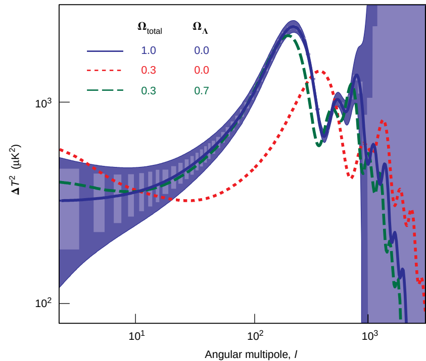
Figure 6. MAP and the Future Temperature fluctuation squared is plotted to show how the MAP mission can distinguish between different theoretical models, here cold dark matter (dark blue curve), an open model with \Omega = 0.3 (dashed red curve), and a model with a nonzero cosmological constant \Omega_\Lambda (dashed green curve). The rectangles that follow the blue curve are projected error bars, while the solid-blue envelope represents the so-called “cosmic variance,” a finite sampling effect due to the fact that the observation is restricted to only a fraction of the Universe. Thus MAP will provide useful information for multipoles up to l \sim 1000 and is dominated by cosmic variance up to l \sim 600 . If this figure corresponded to real data, only the cold dark matter model would be viable.
