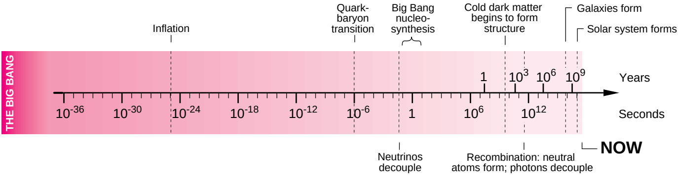
Figure 1. The Universe’s Time Line The Big Bang model allows cosmologists to order events in the evolution of the Universe. This figure plots time on a logarithmic scale. Although cold dark matter begins to form structures within the first 100 years or so of the Universe’s history, those structures do not evolve into galaxies (or clusters of galaxies) until many millions of years later.
