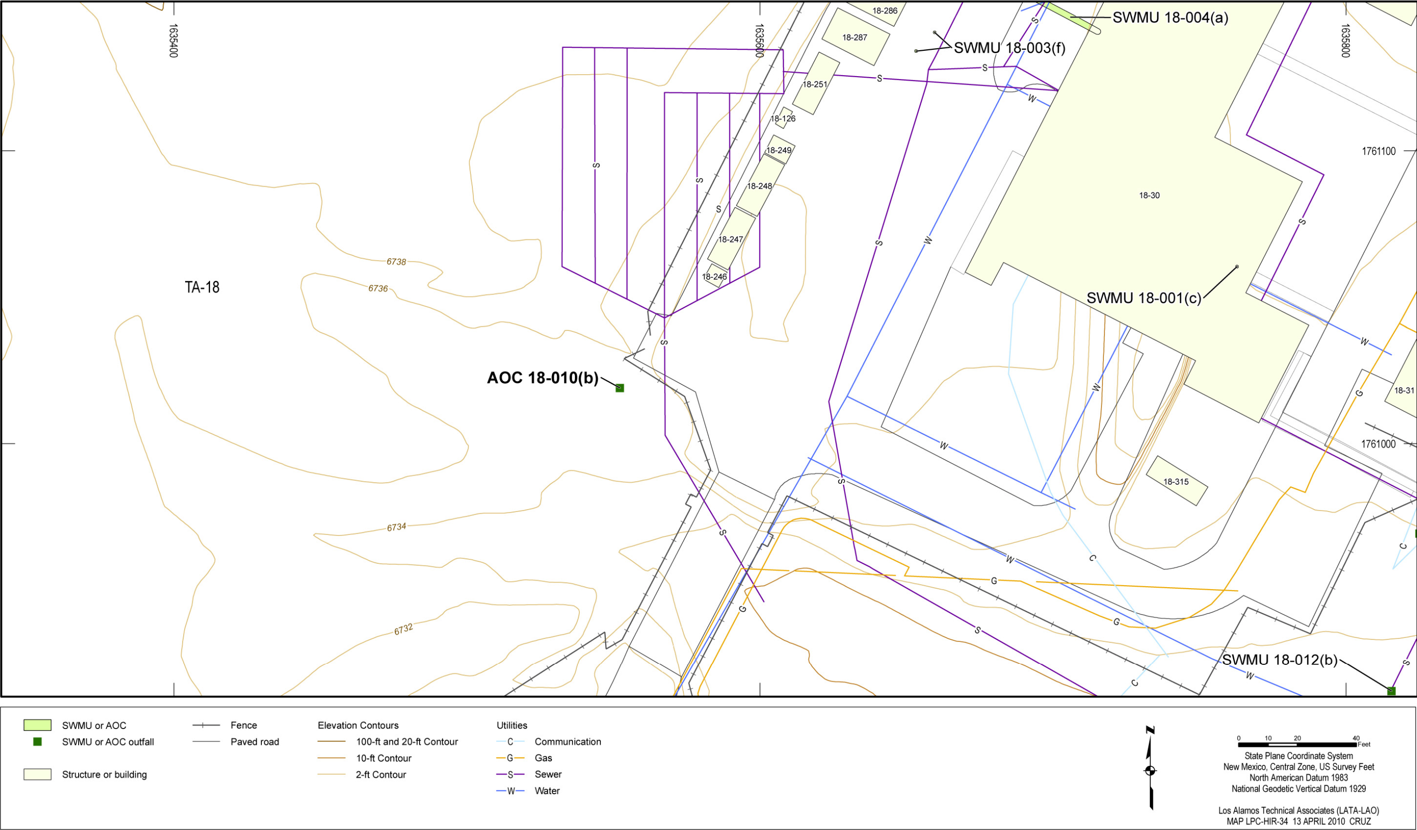
Figure 4.17-1 Site features of AOC 18-010(b)
