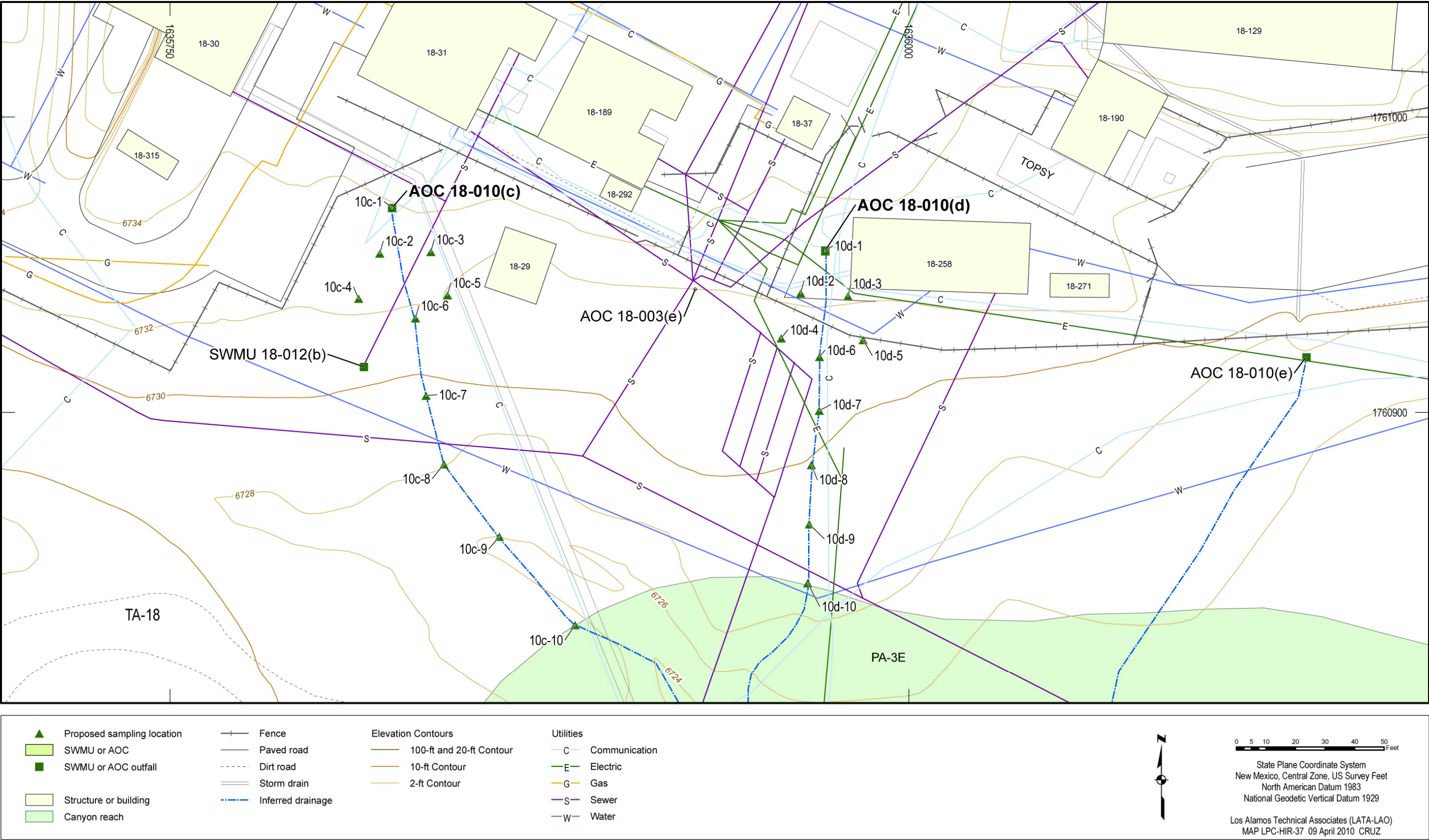
Figure 4.18-2 Proposed sampling locations for AOCs 18-010(c) and 18-010(d)
