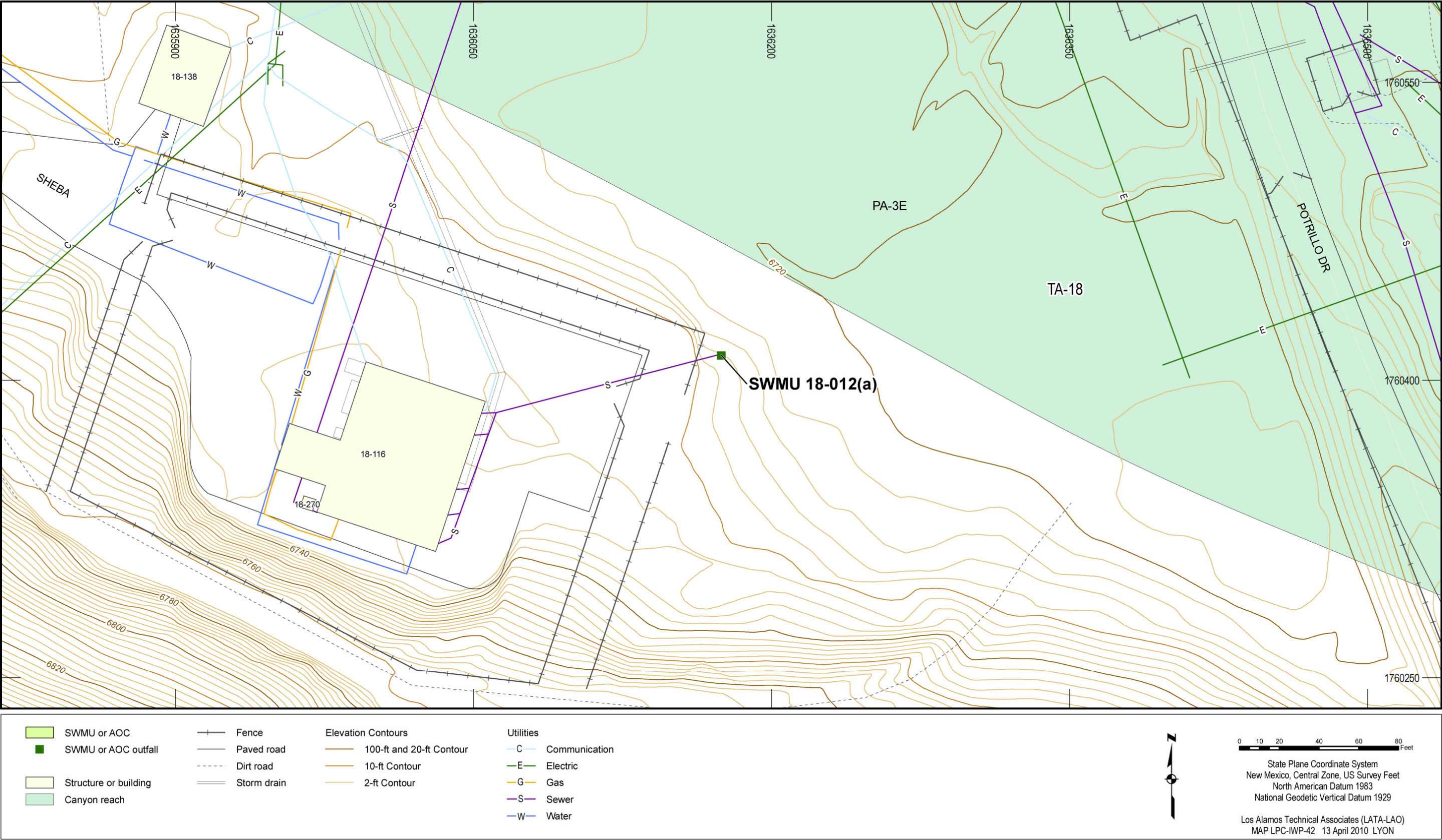
Figure 4.23-1 Site features of SWMU 18-012(a)
