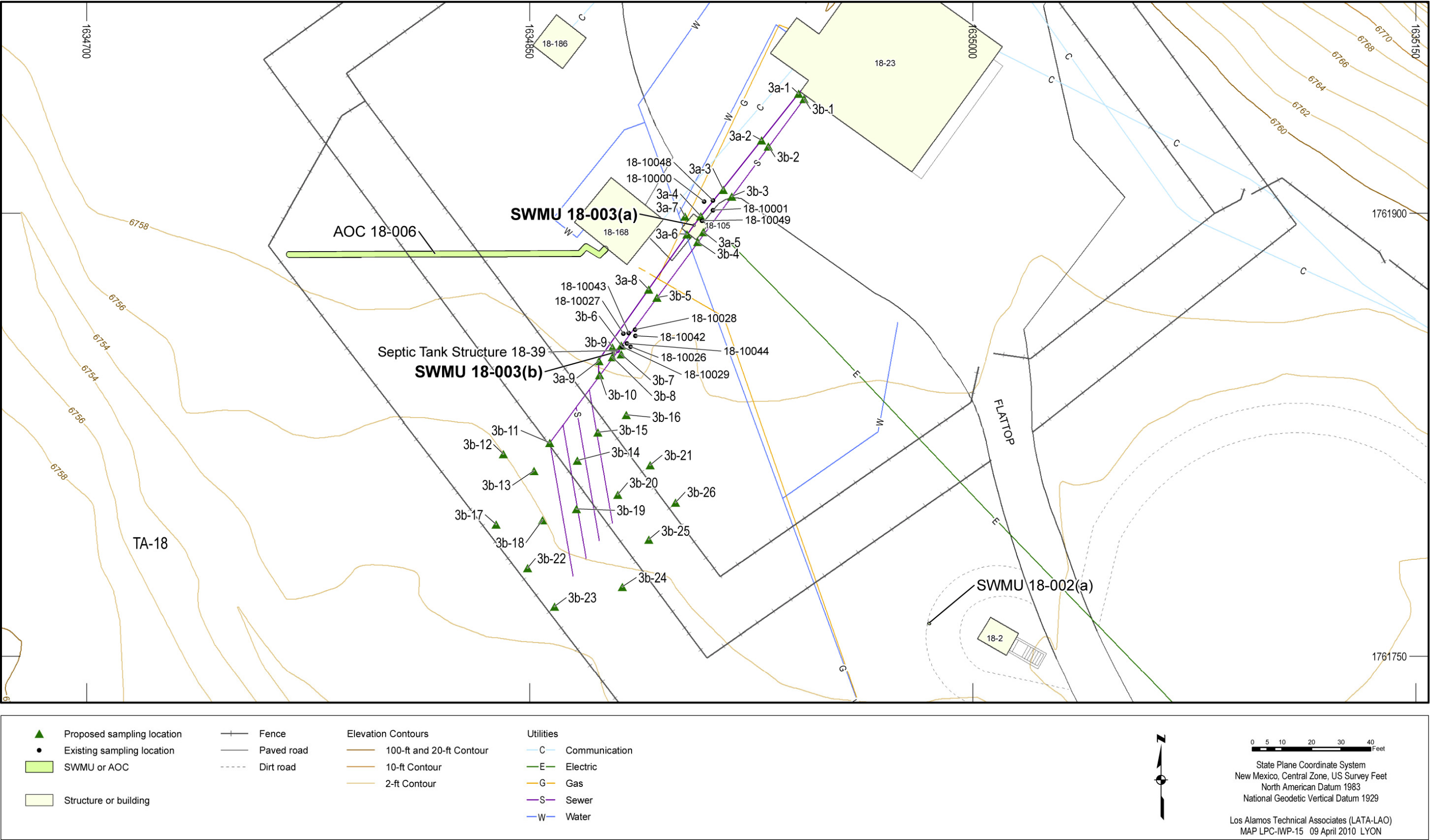
Figure 4.6-5 Proposed sampling locations for Consolidated Unit 18-003(a)-00 [SWMU 18-003(a) and SWMU 18-003(b)]
