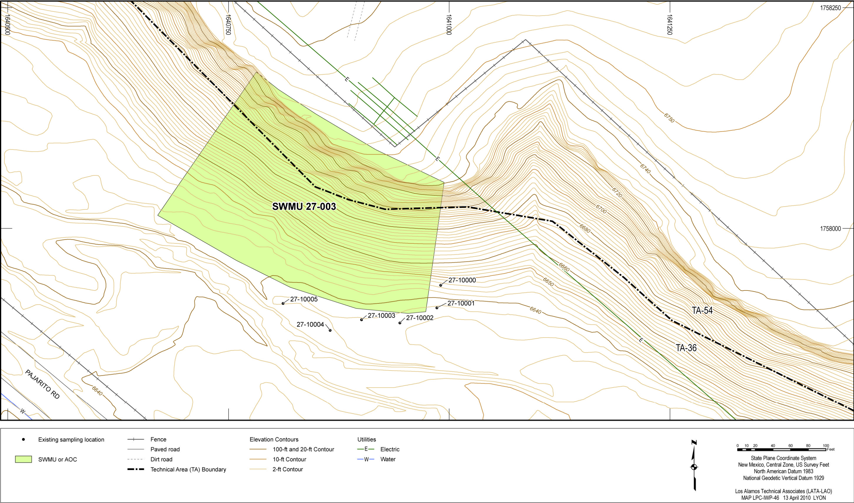
Figure 5.2-1 Site features of SWMU 27-003
