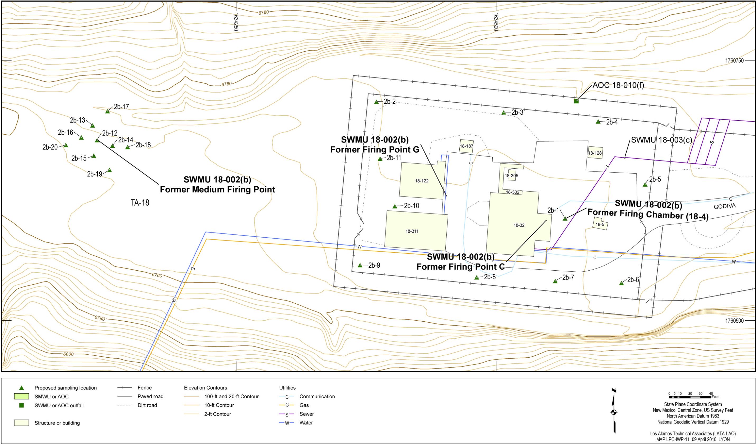
Figure 4.4-2 Proposed sampling locations for SWMU 18-002(b)
