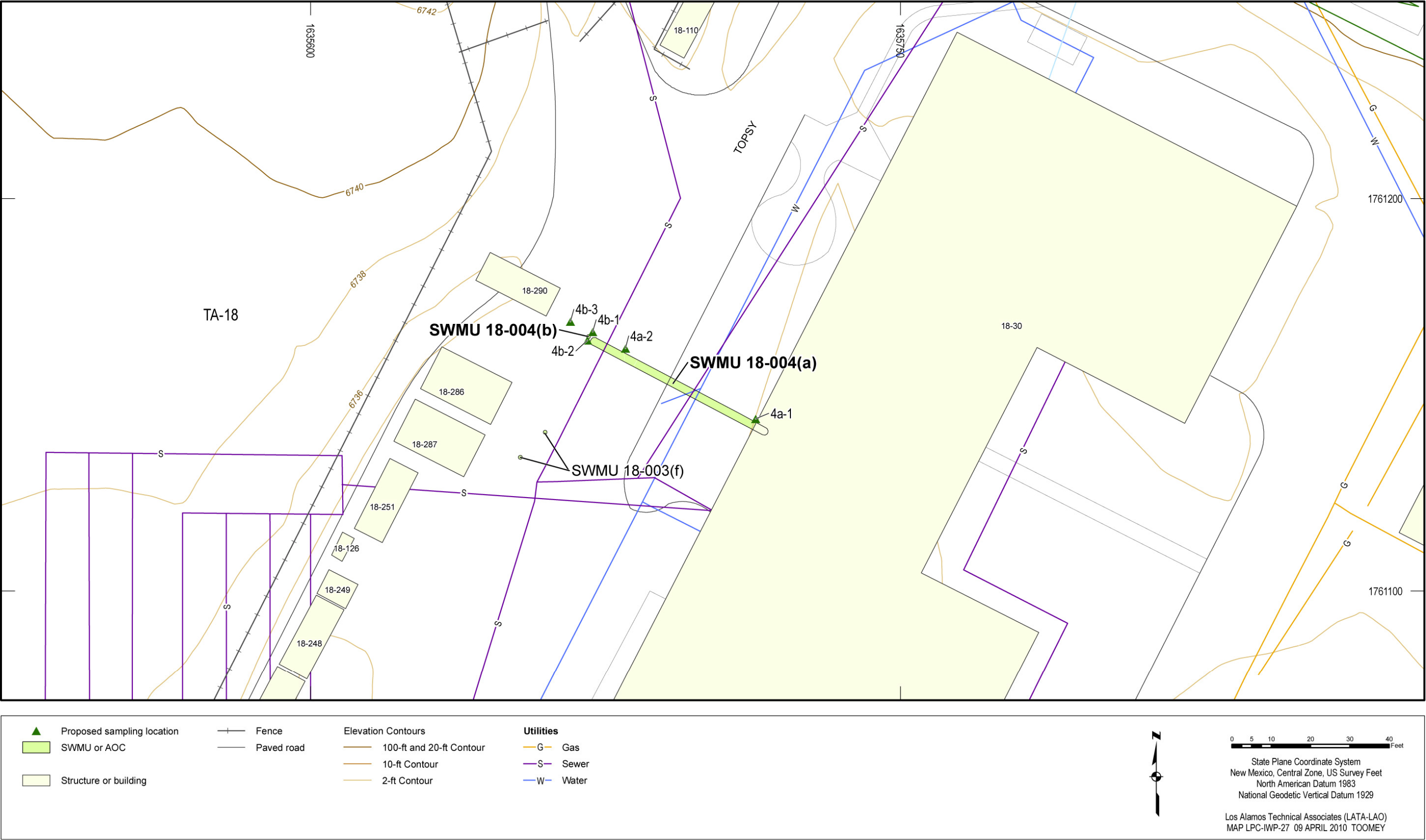
Figure 4.13-2 Proposed sampling locations for Consolidated Unit 18-004(a)-00 [SWMUs 18-004(a) and 18-004(b)]
