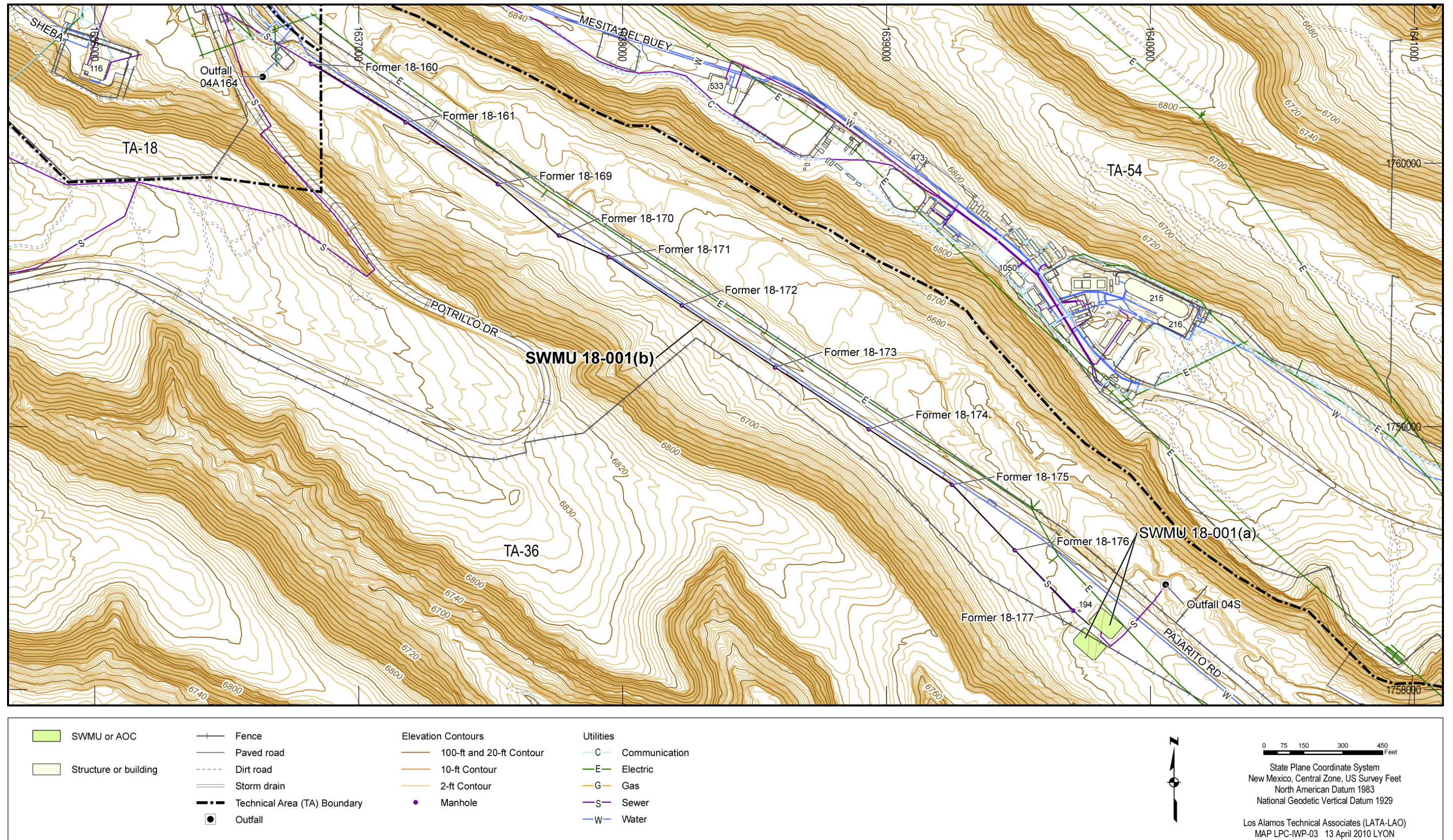
Figure 4.1-2 Site features of Consolidated Unit 18-001(a)-00 [SWMU 18-001(b)]
