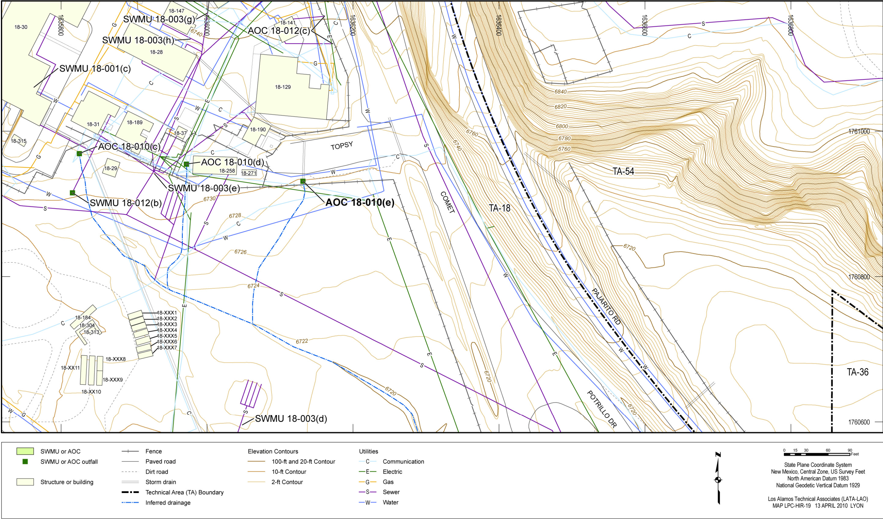
Figure 4.20-1 Site features of AOC 18-010(e)
