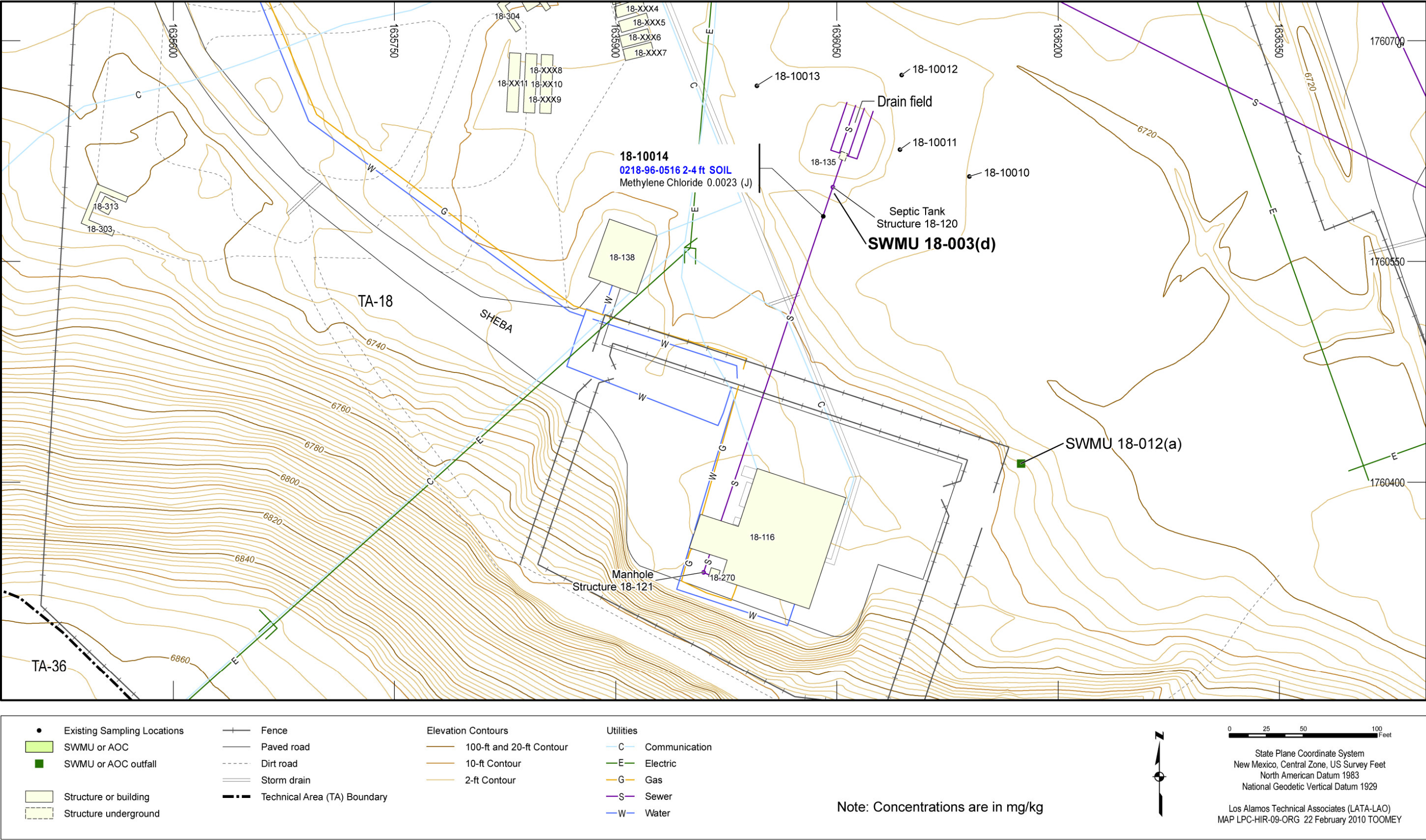
Figure 4.8-3 Organic chemicals detected at SWMU 18-003(d)
