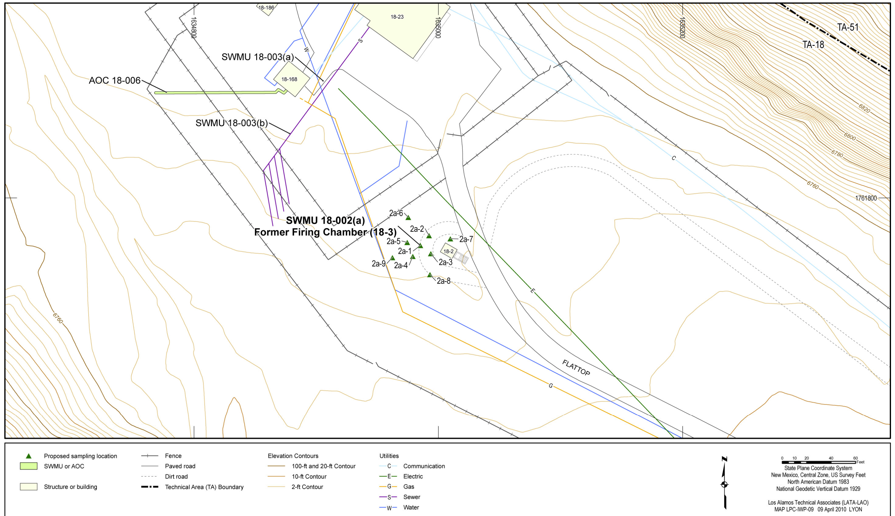
Figure 4.3-2 Proposed sampling locations for SWMU 18-002(a)
