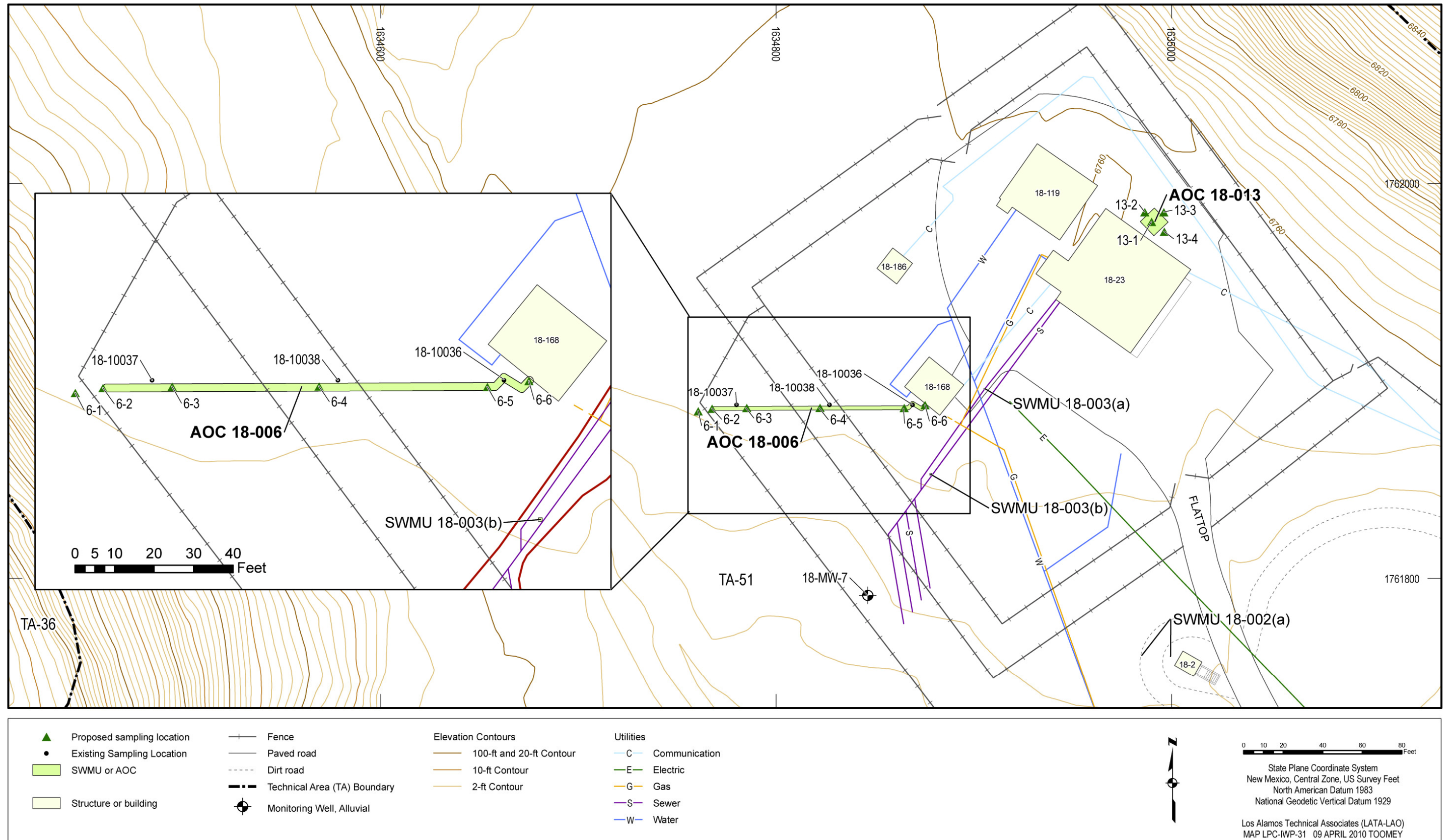
Figure 4.15-4 Proposed sampling locations for AOCs 18-006 and 18-013
