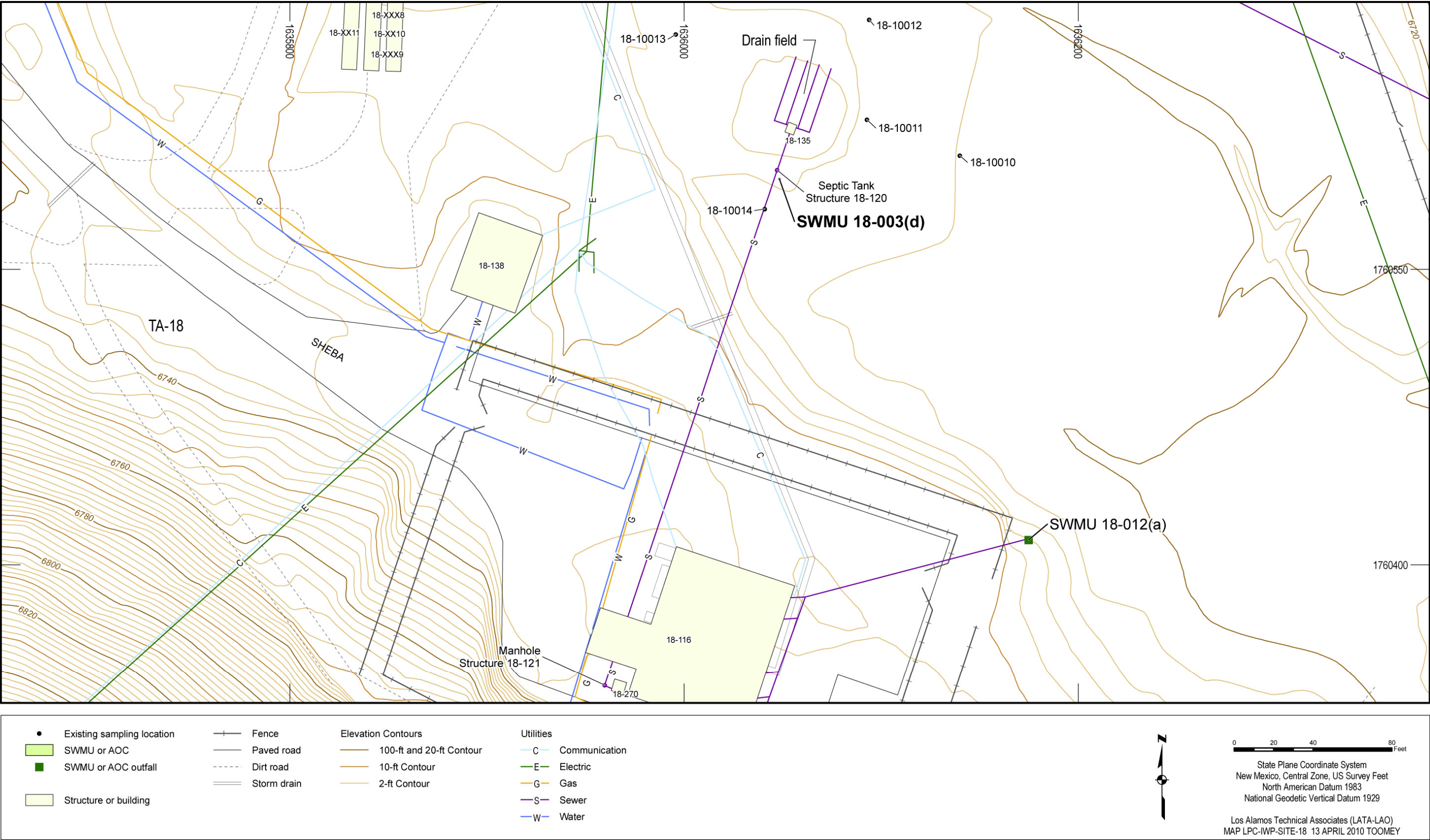
Figure 4.8-1 Site features of SWMU 18-003(d)
