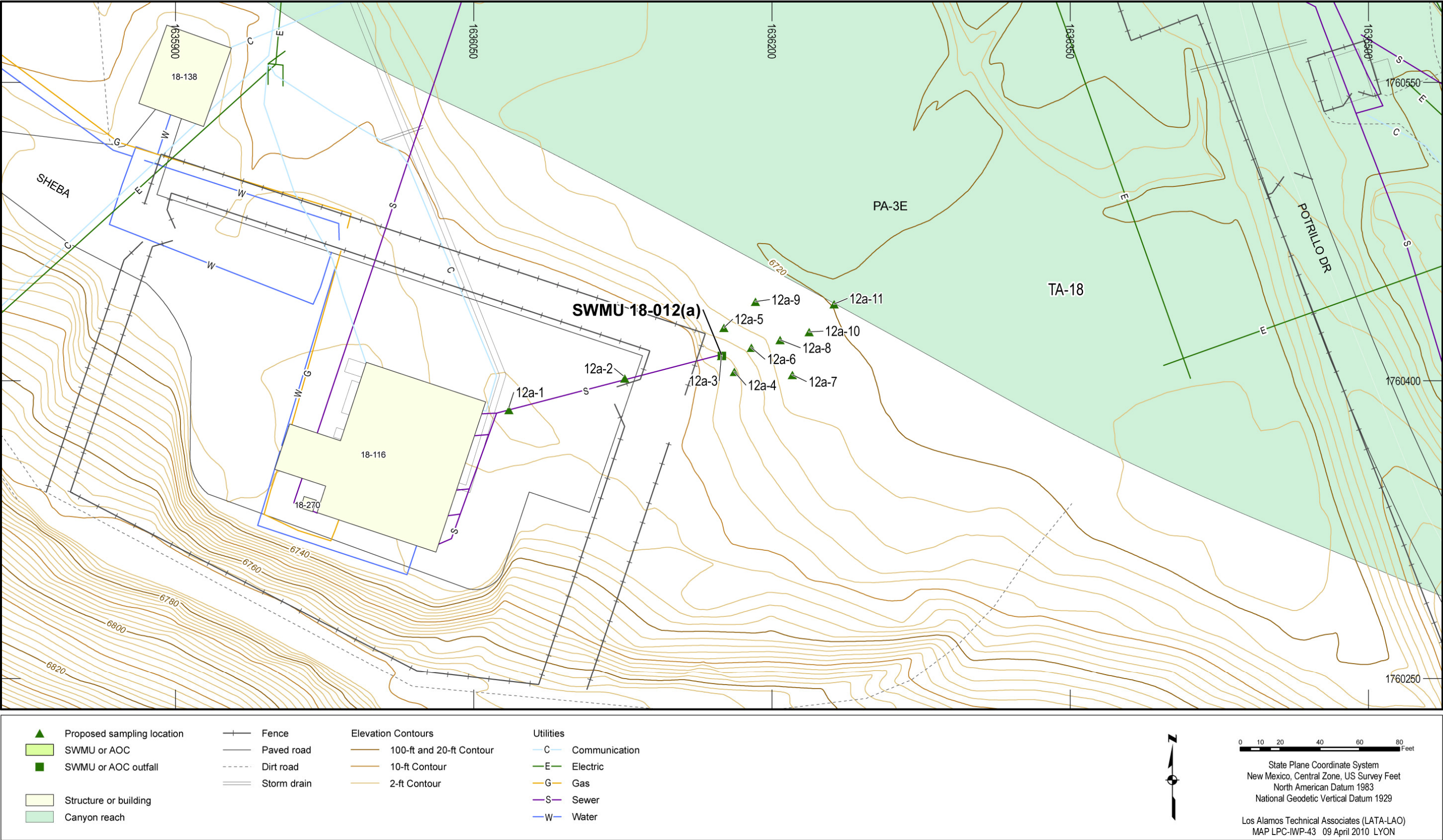
Figure 4.23-2 Proposed sampling locations for SWMU 18-012(a)
