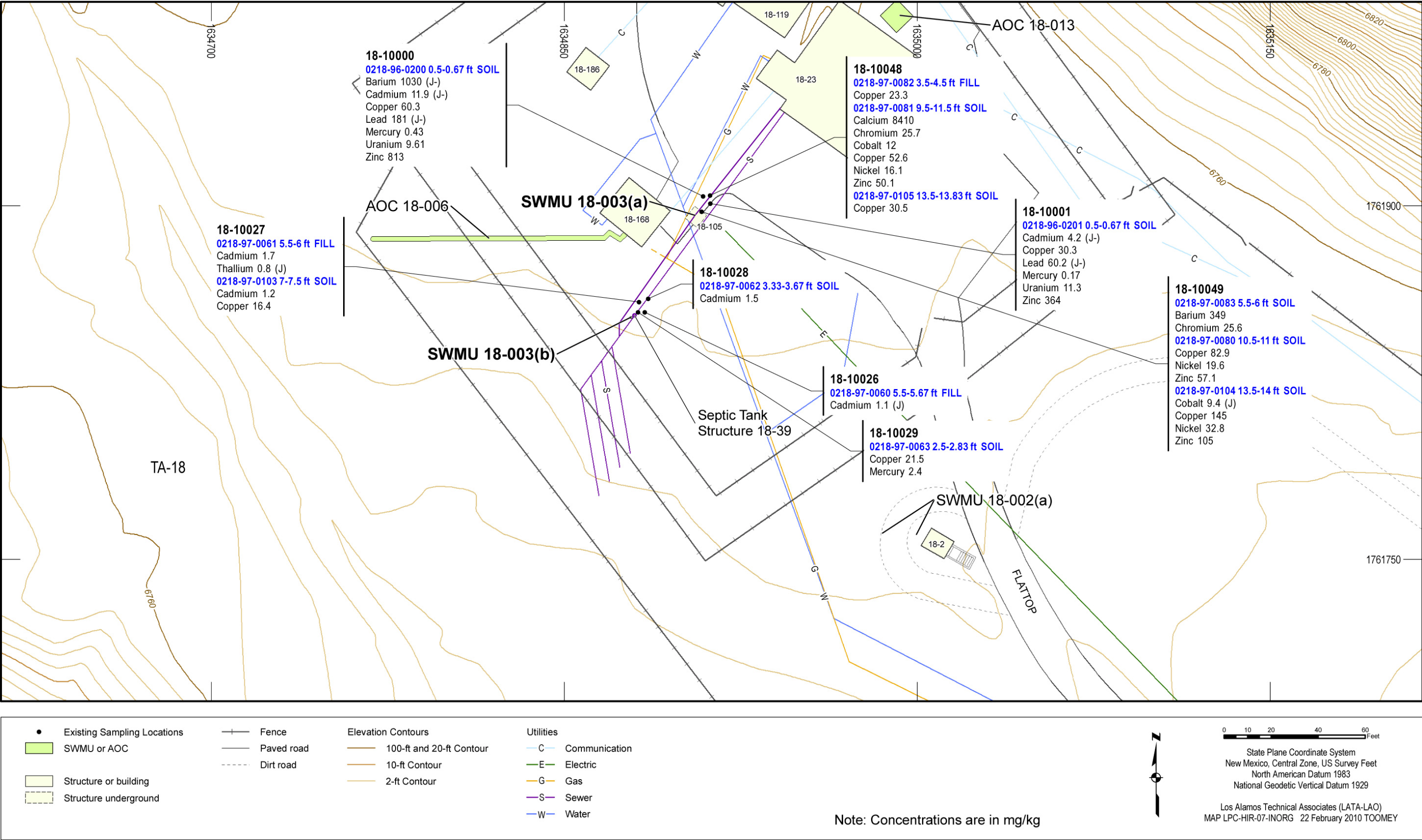
Figure 4.6-2 Inorganic chemicals detected above BVs at Consolidated Unit 18-003(a)-00 [SWMUs 18-003(a) and 18-003(b)]
