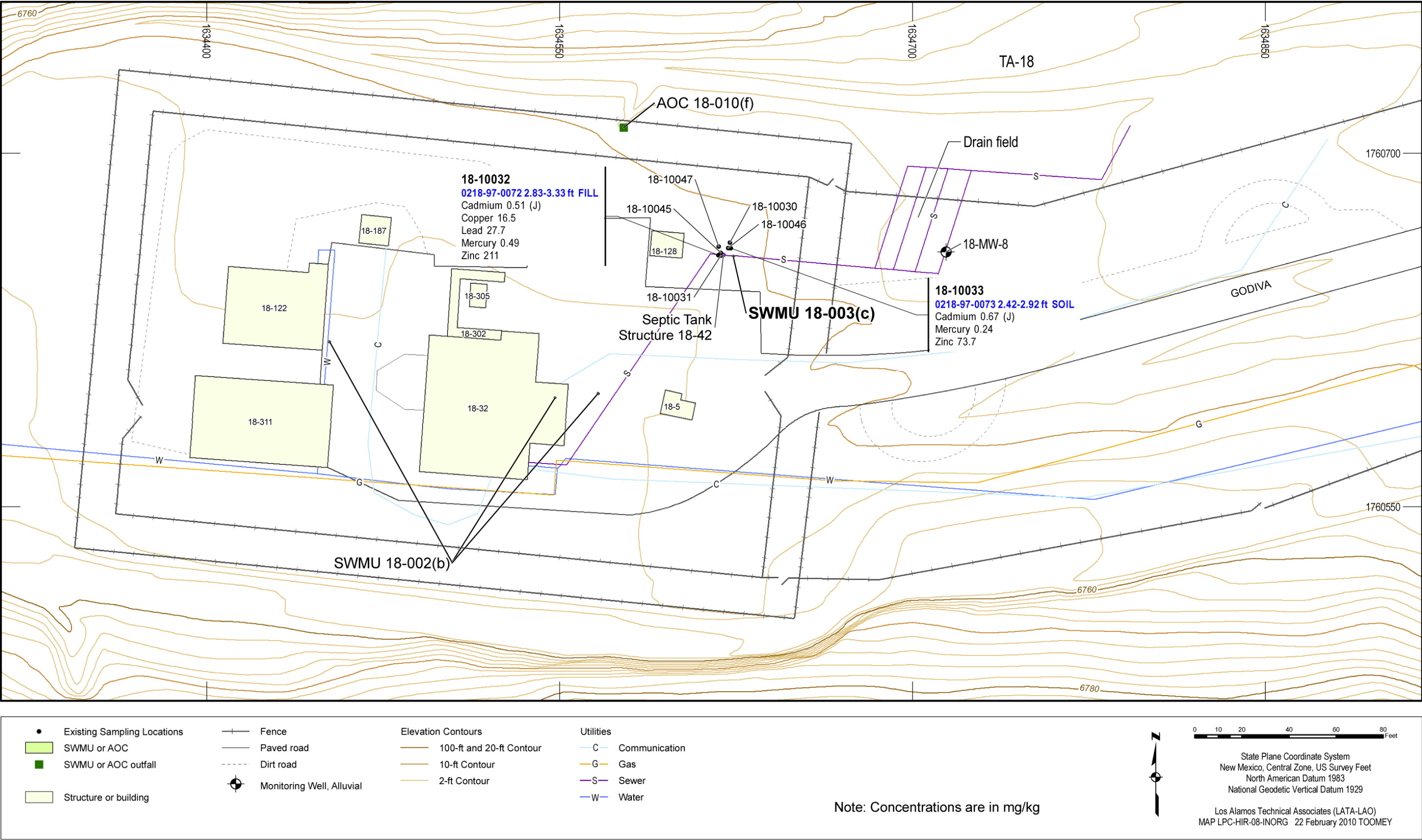
Figure 4.7-2 Inorganic chemicals detected above BVs at SWMU 18-003(c)
