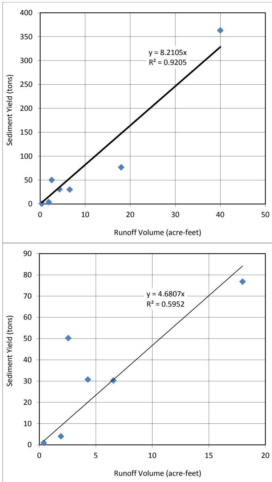
Figure 3.2-4 Relationship between sediment yield and runoff volume with (top) and without (bottom) August 15 storm at E109.9
