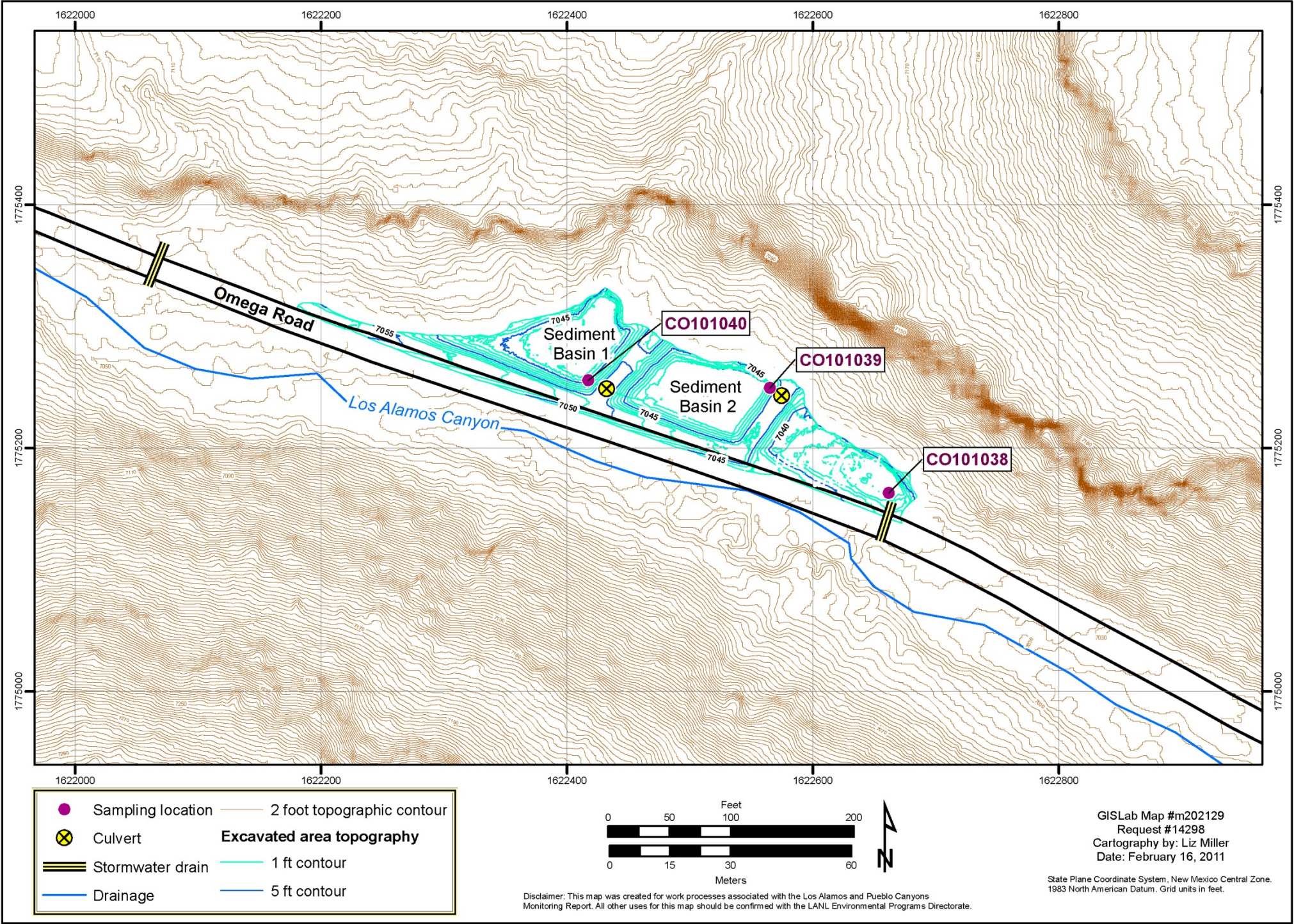
Figure 2.1-1 Watershed mitigations and sampling locations at the retention basins and wetland below the SWMU 01-001(f) drainage
