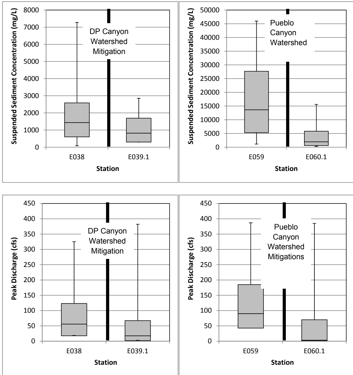
Figure 3.3-2 Box and whisker plot of suspended sediment concentrations (top) and peak discharge (bottom) upstream and downstream of the DP Canyon Watershed Mitigation (left) and Pueblo Canyon Watershed Mitigations (right)
