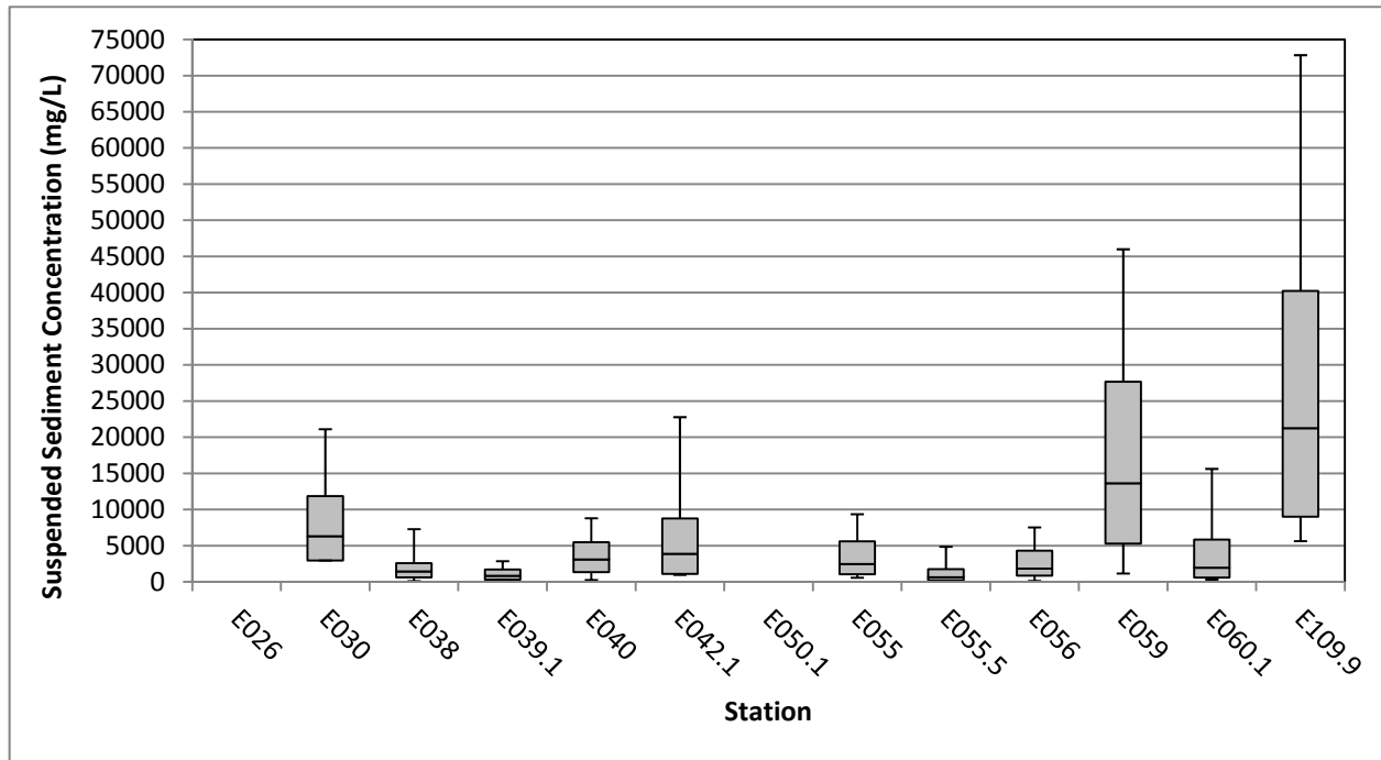
Figure 3.1-1 Box and whisker plot of suspended sediment concentrations for each station (no suspended sediment samples were collected at E026 or E050.1)
