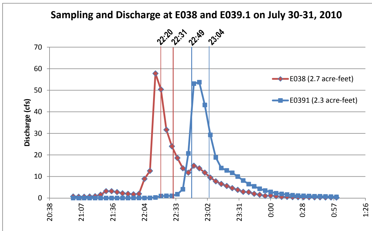
Figure 3.3-1 Discharge at E038 and E039.1 in DP Canyon on July 9 and July 30-31
