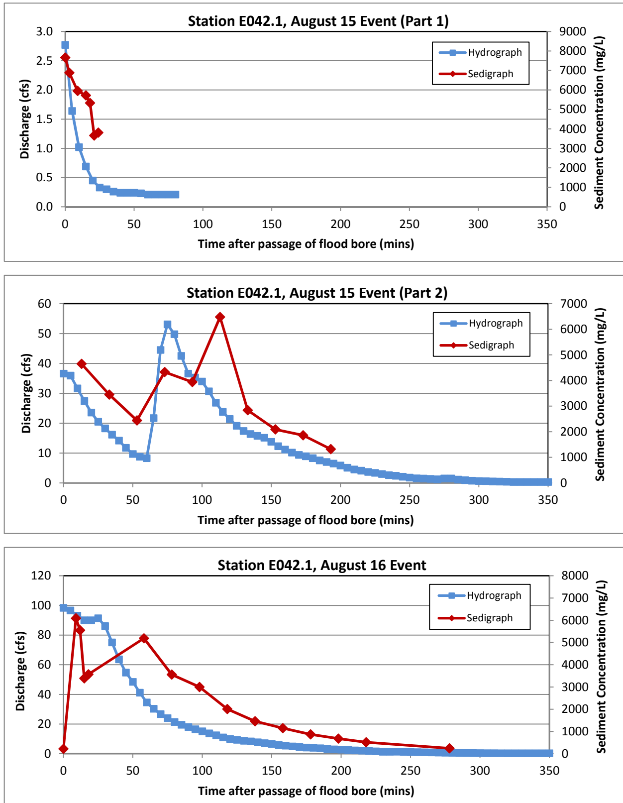
Figure 3.2-3 (continued) Discharge and suspended sediment concentration for each station sampled throughout the storm event
