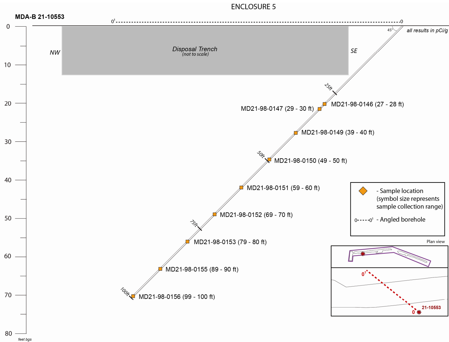
Figure 3.3-4 Schematic profile of MDA B location ID 21-10553
