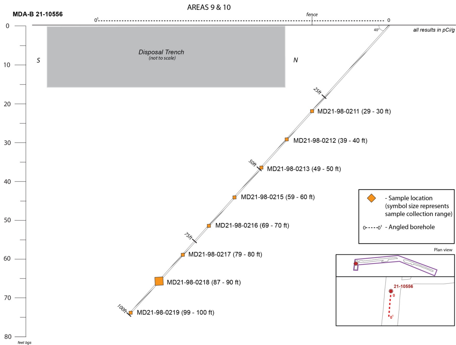
Figure 3.3-7 Schematic profile of MDA B location ID 21-10556
