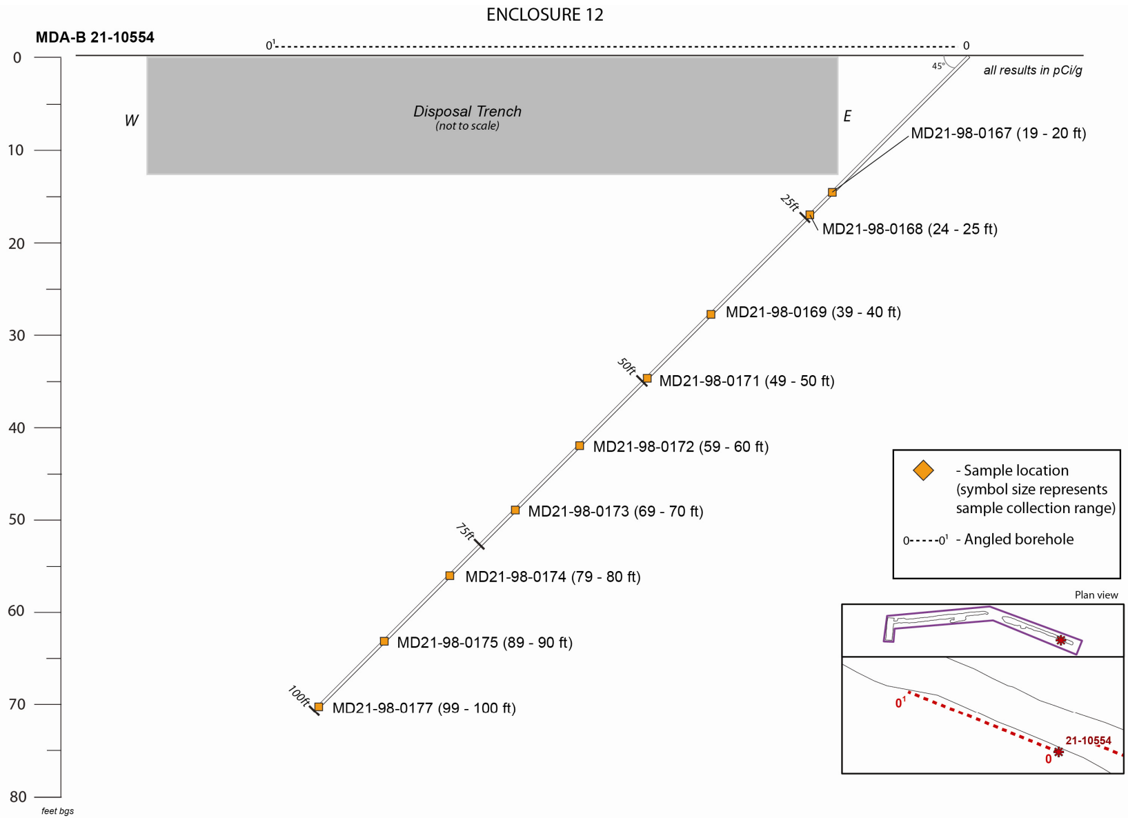
Figure 3.3-5 Schematic profile of MDA B location ID 21-10554
