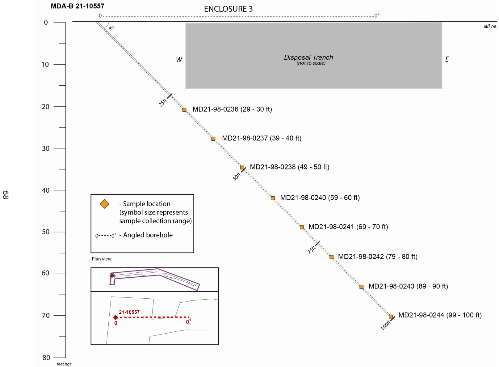
Figure 3.3-8 Schematic profile of MDA B location ID 21-10557
