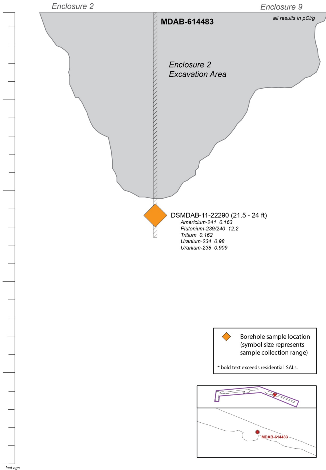
Figure 6.3-3 Schematic of MDAB-614483
