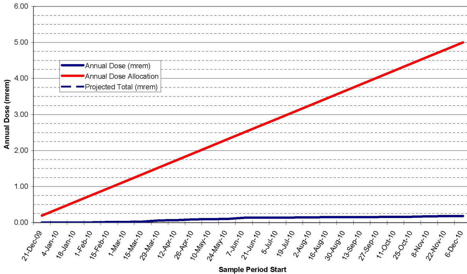
Figure G-2 AIRNET Site ID 317 from 2010
