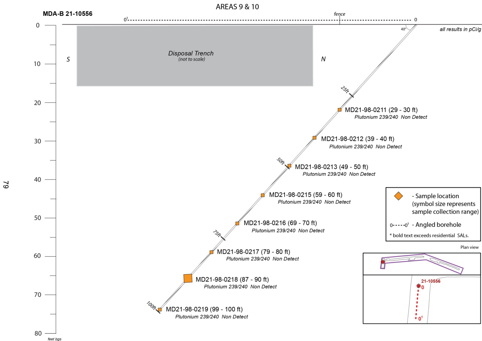
Figure 7.4-6 Borehole diagram of 21-10556
