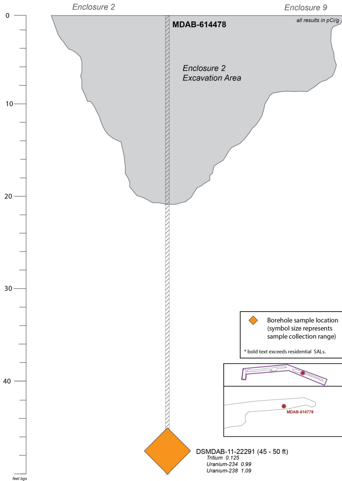
Figure 6.3-2 Schematic of MDAB-614478
