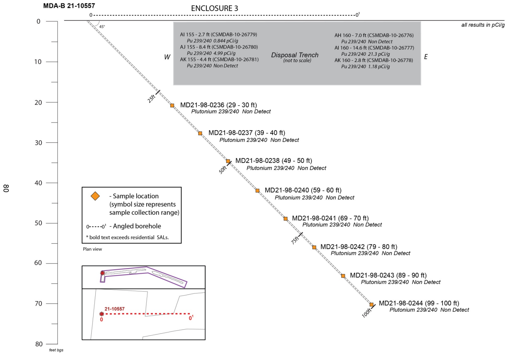
Figure 7.4-7 Borehole diagram of 21-10557
