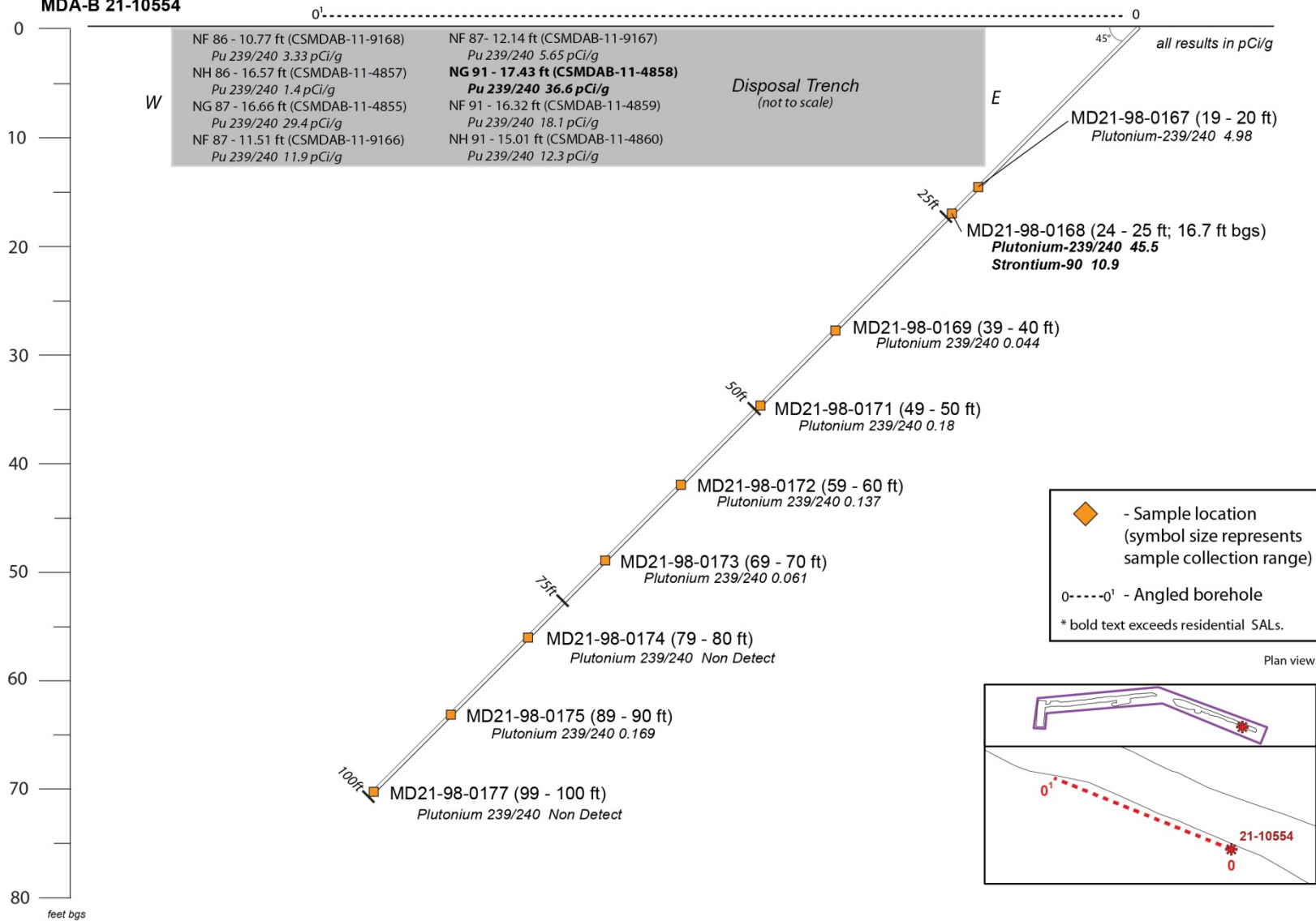
Figure 7.4-4 Borehole diagram of 21-10554
