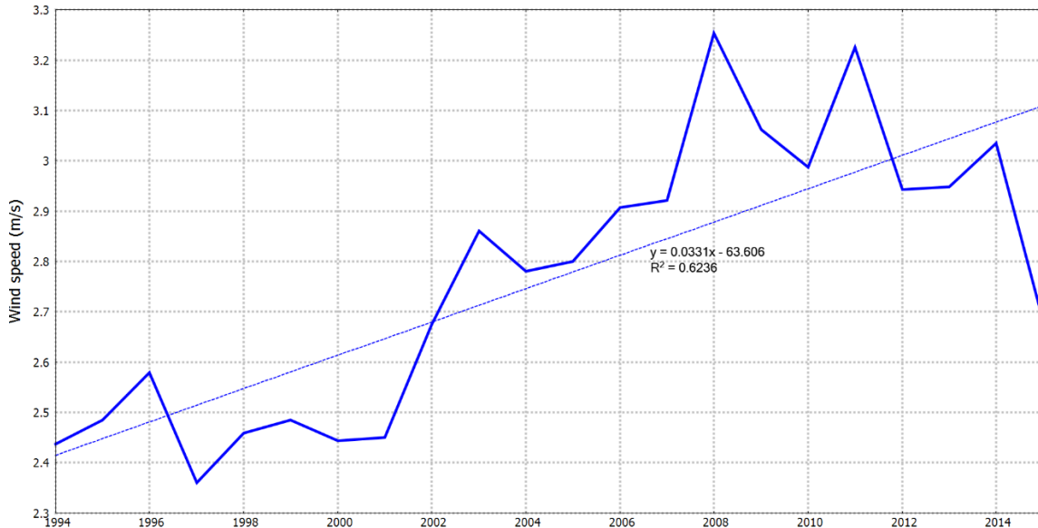
Figure 10-11: Annual average wind speed at 12 meters AGL at TA-6 (1994–2015).
