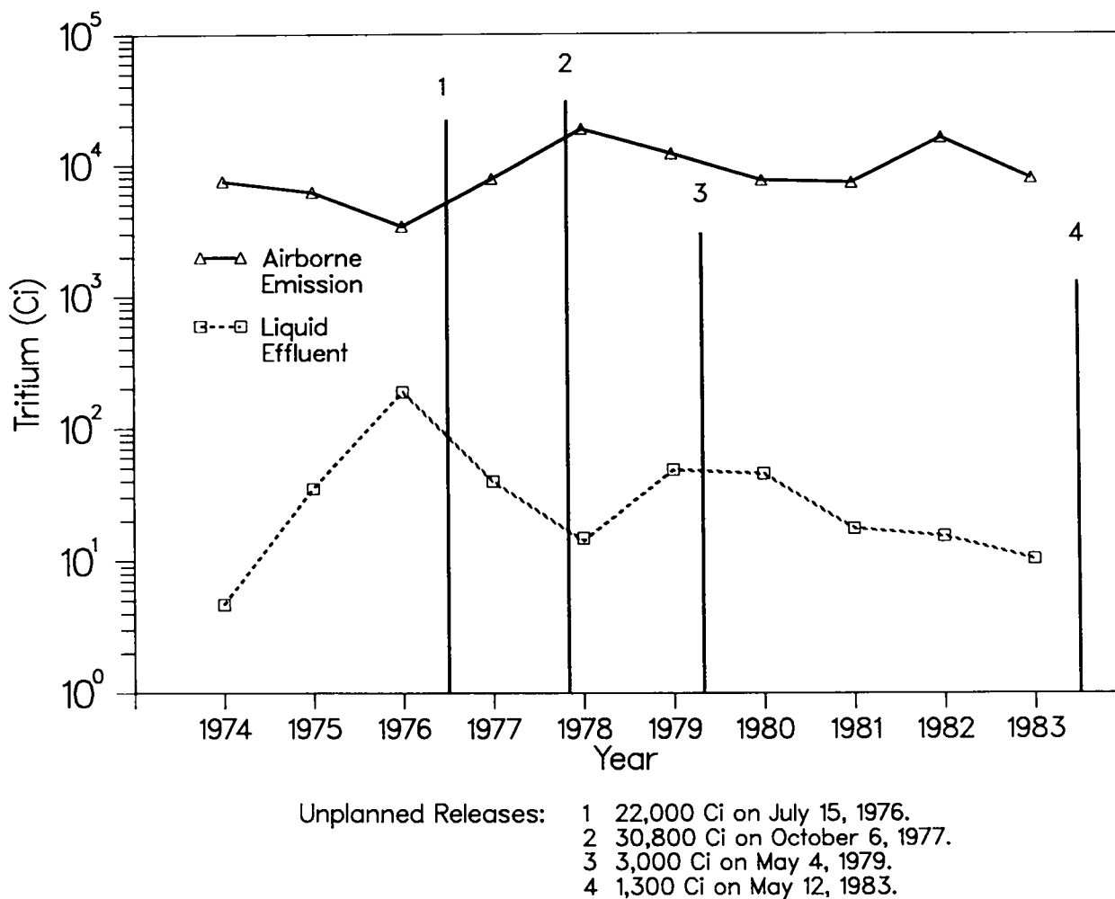
Fig. 21. Summary of tritium releases (airborne emissions and liquid effluents).
