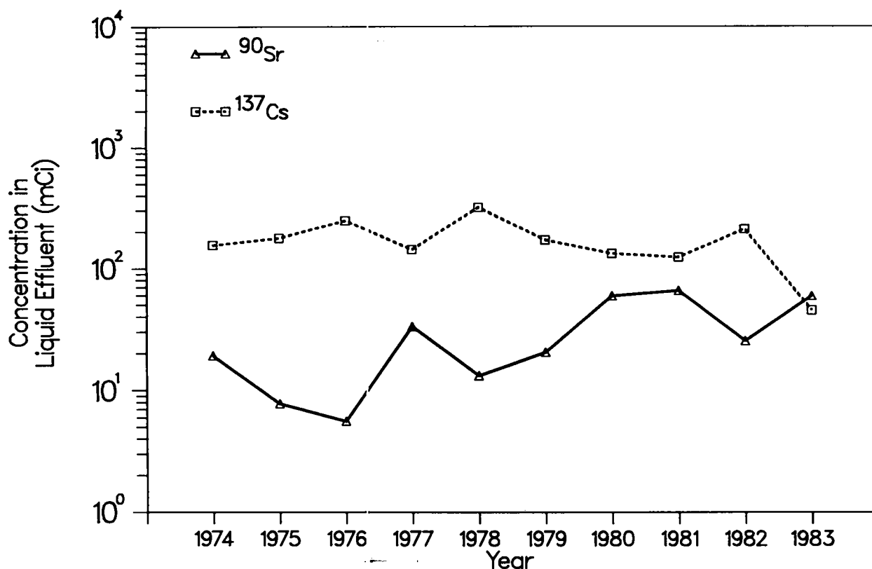
Fig. 24. Summary of strontium and cesium liquid effluent releases.
