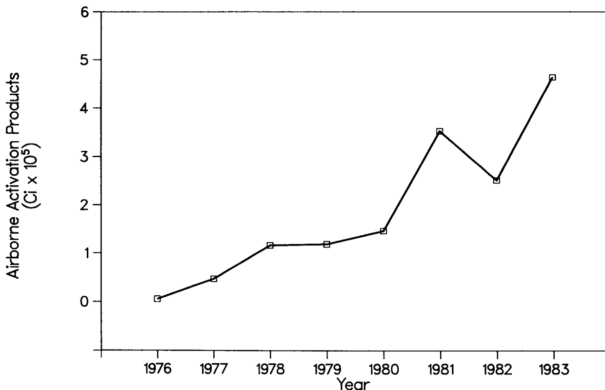
Fig. 23. Airborne activation product releases ( ^{11}\text{C} , ^{13}\text{N} , ^{14}\text{O} , ^{15}\text{O} , ^{41}\text{Ar} , ^{192}\text{Au} , ^{195}\text{Hg} ) from the Los Alamos Meson Physics Facility (TA-53).
