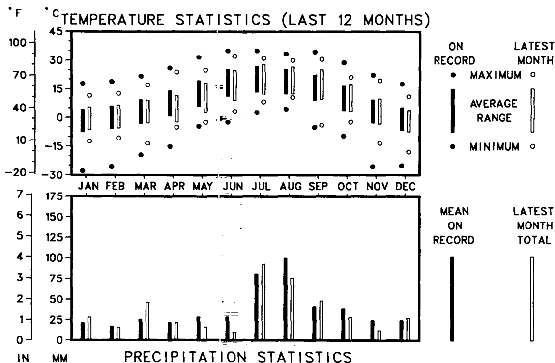
Fig. 26. Summary of 1983 weather in Los Alamos (data from Occupational Health Laboratory, OHL, TA-59).
