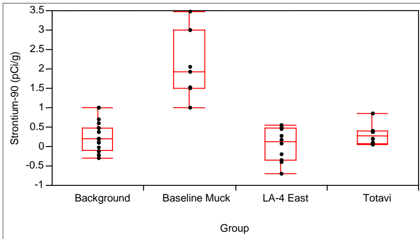
Figure A-5. Box plot for strontium-90
