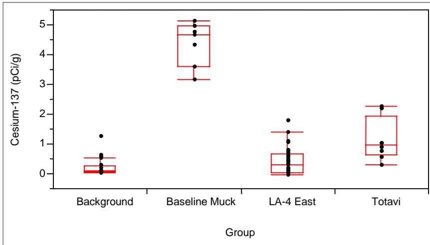
Figure A-2. Box plot for cesium-137
