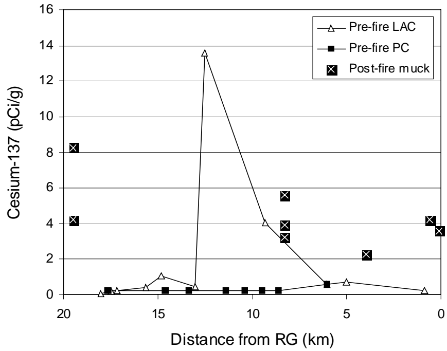
Figure 8. Cesium-137 spatial plot for Los Alamos and Pueblo Canyons sediment concentrations. Pre-fire data from Reneau et al. (1998 a, b, and c). LAC = Los Alamos Canyon, PC = Pueblo Canyon.
