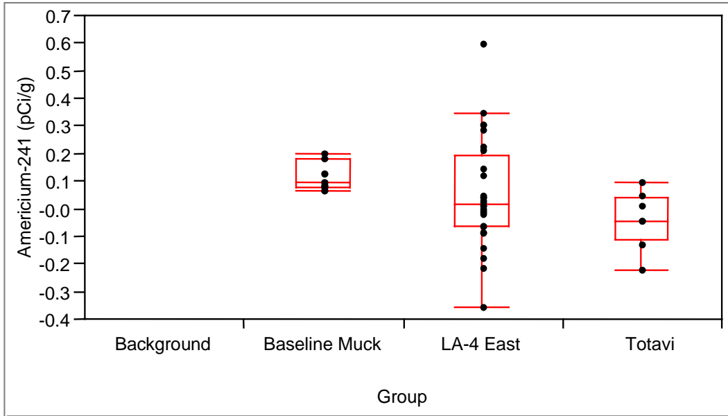
Figure A-1. Box plot for americium-241 (note - there are no background data for americium-241 by gamma spectroscopy - the analytical method used for other data groups)
