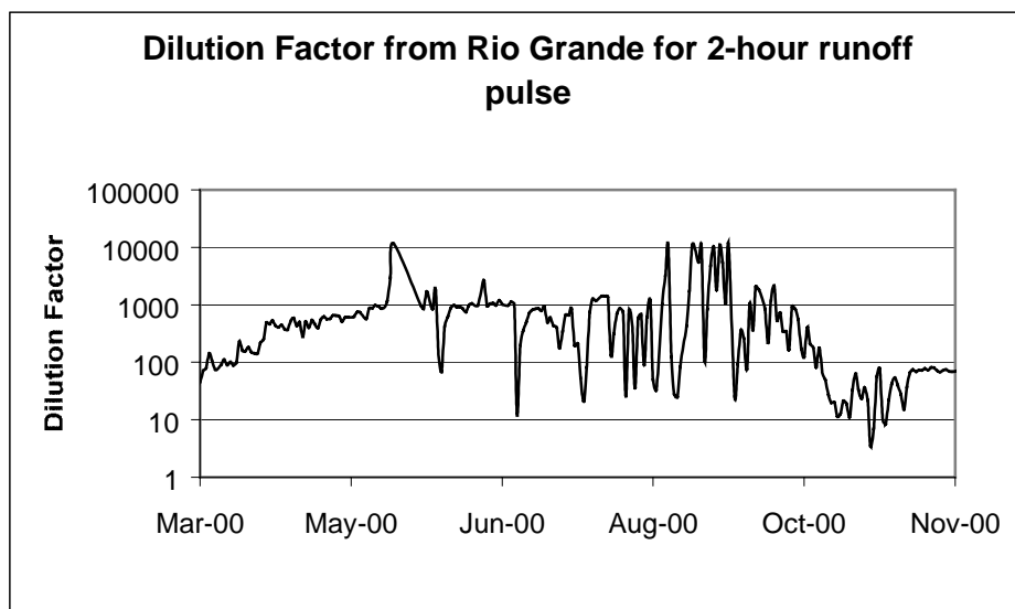
Figure 4. Dilution factors resulting from LANL-canyon runoff mixing with Rio Grande flows over a 2-hour period during year 2000. Minimum dilution occurs on October 23.
