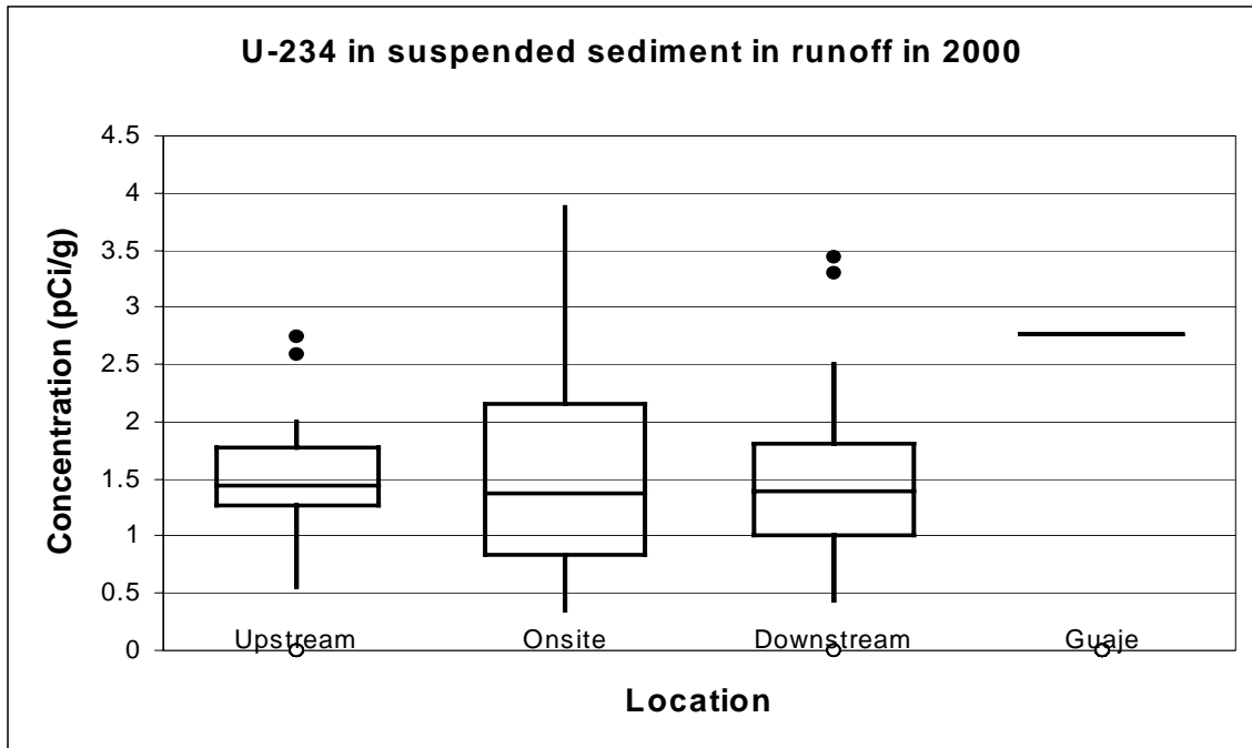
Figure 5. Concentrations of uranium isotopes in suspended sediment carried by runoff in LANL canyons and in Guaje Canyon. These box plots are useful for evaluating differences among groups of data. We use the plots to summarize the distribution of concentrations in sediments in locations upstream (of LANL), LANL on-site, downstream, and at Guaje Canyon for reference. The horizontal line in the middle of the box represents the median concentration. The upper and lower ends of the box delimit the spread of the data by including the middle 50% of the values. Possible statistical outliers are shown with circles.
