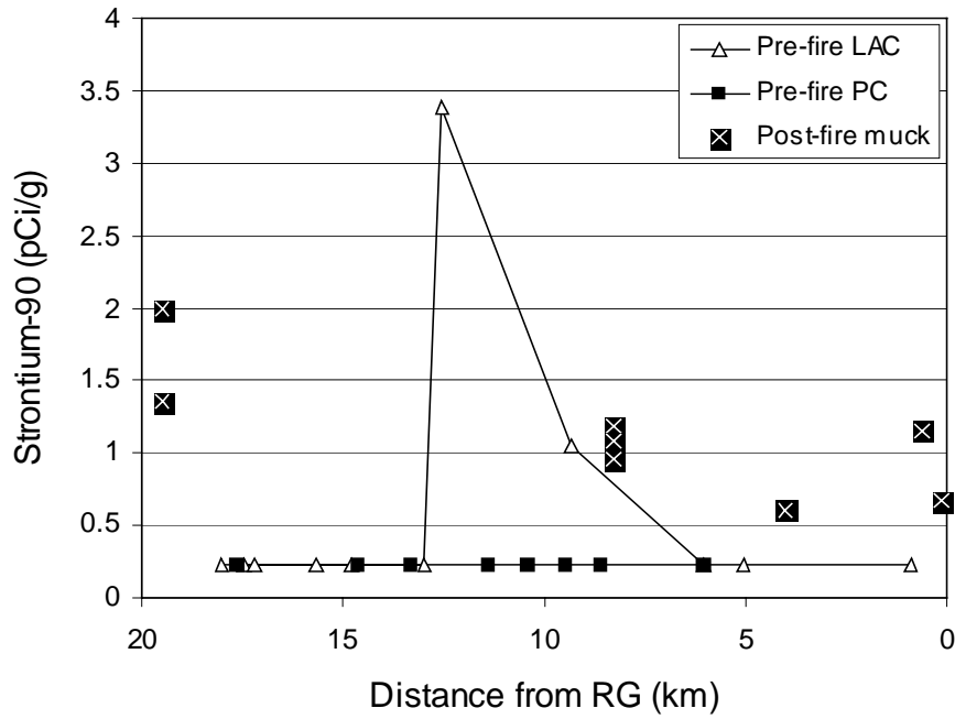
Figure 9. Strontium-90 spatial plot for Los Alamos and Pueblo Canyon sediment concentrations. Pre-fire data from Reneau et al. (1998 a, b, and c). LAC = Los Alamos Canyon, PC = Pueblo Canyon.
