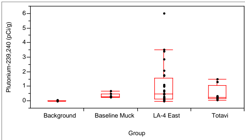
Figure A-4. Box plot for plutonium-239,240
