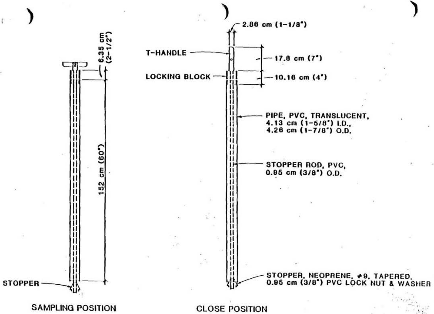
FIGURE E-3.3 COMPOSITE LIQUID WASTE SAMPLER (COLIWASA)
