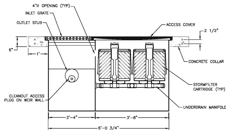
A CATCH BASIN FILTER-SECTION VIEW SCALE: NONE
