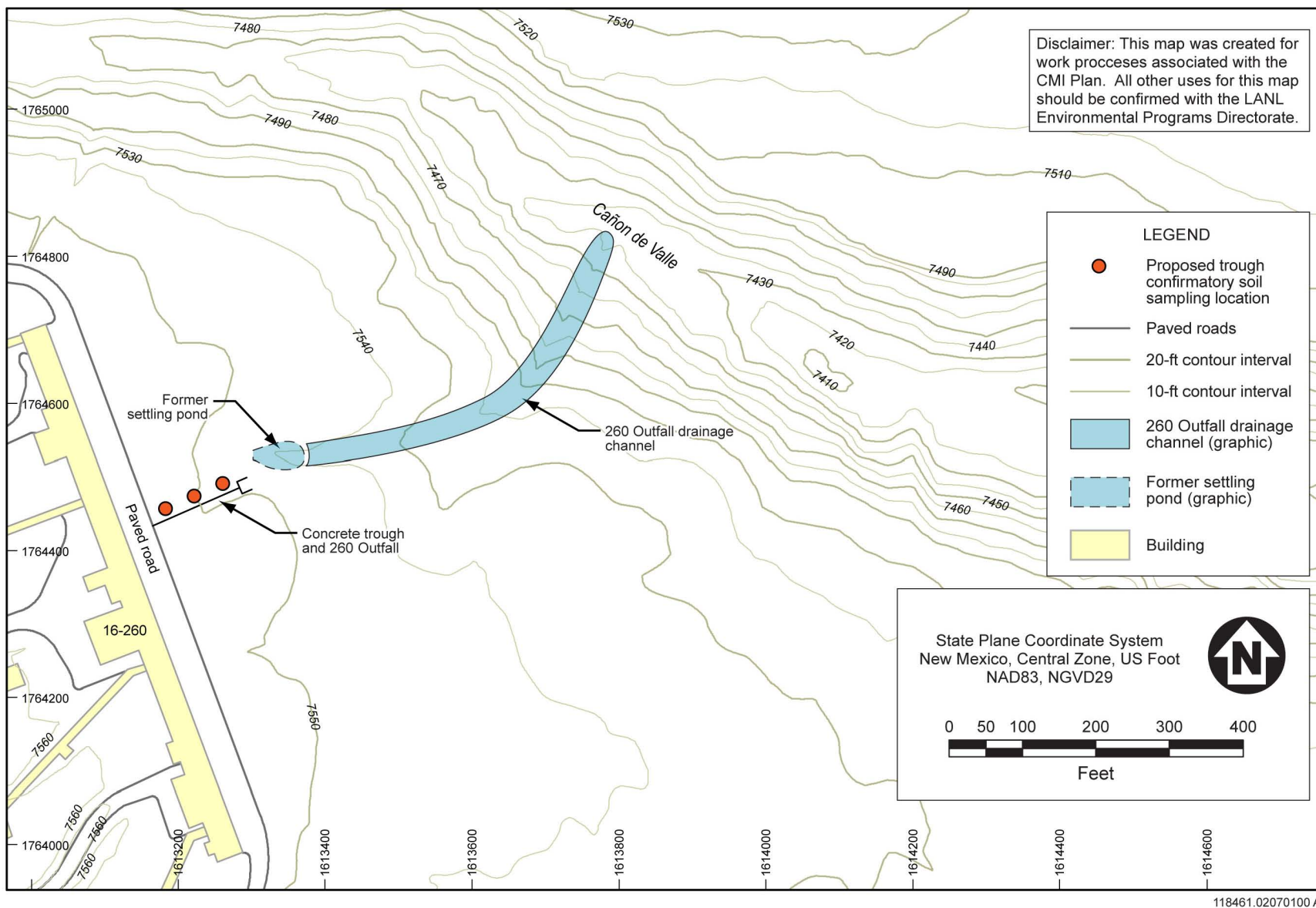
Figure 3.1-1 260 Outfall drainage channel and associated structures
