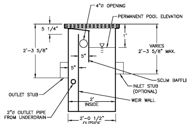
B CATCH BASIN FILTER-SECTION VIEW SCALE: NONE
