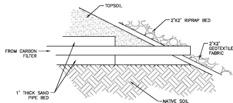
D SECTION SURFACE DISCHARGE SCALE: NONE
