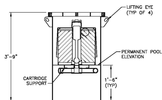
C CATCH BASIN FILTER-SECTION VIEW SCALE: NONE
