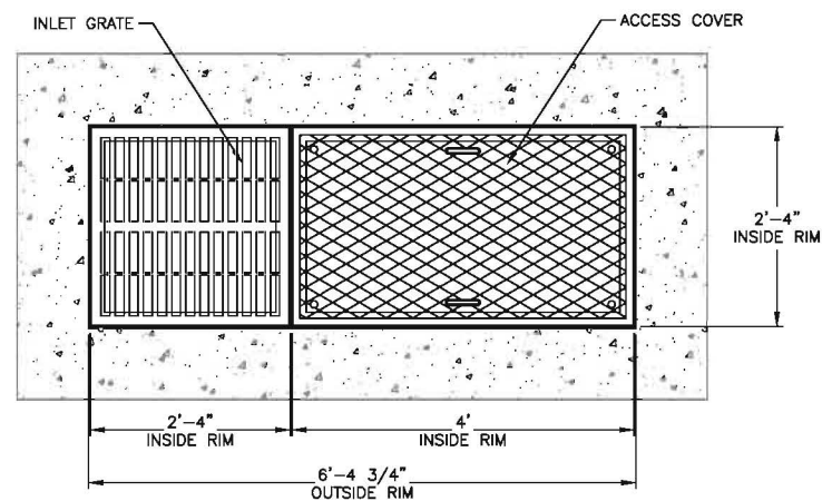
2 DETAIL CATCH BASIN FILTER-TOP VIEW SCALE: NONE
