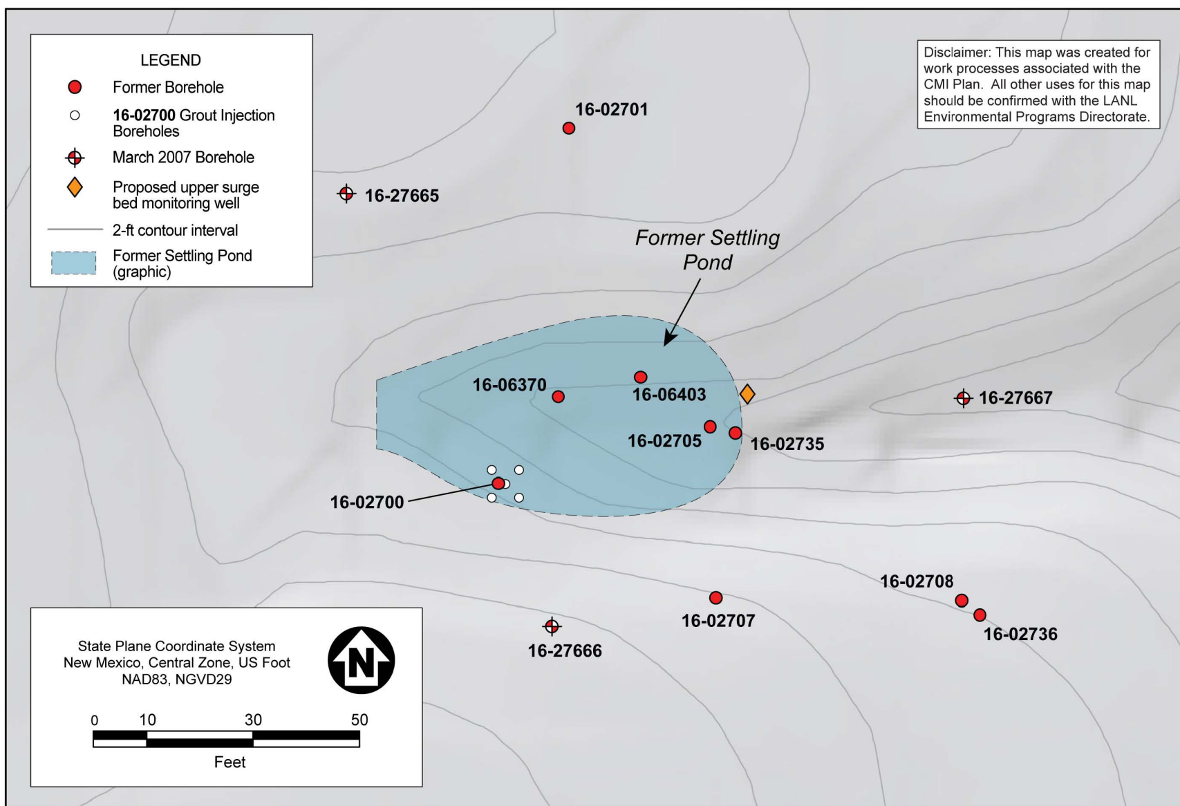
Figure 5.3-1 Former settling pond grouting injection boreholes near BH 16-02700
