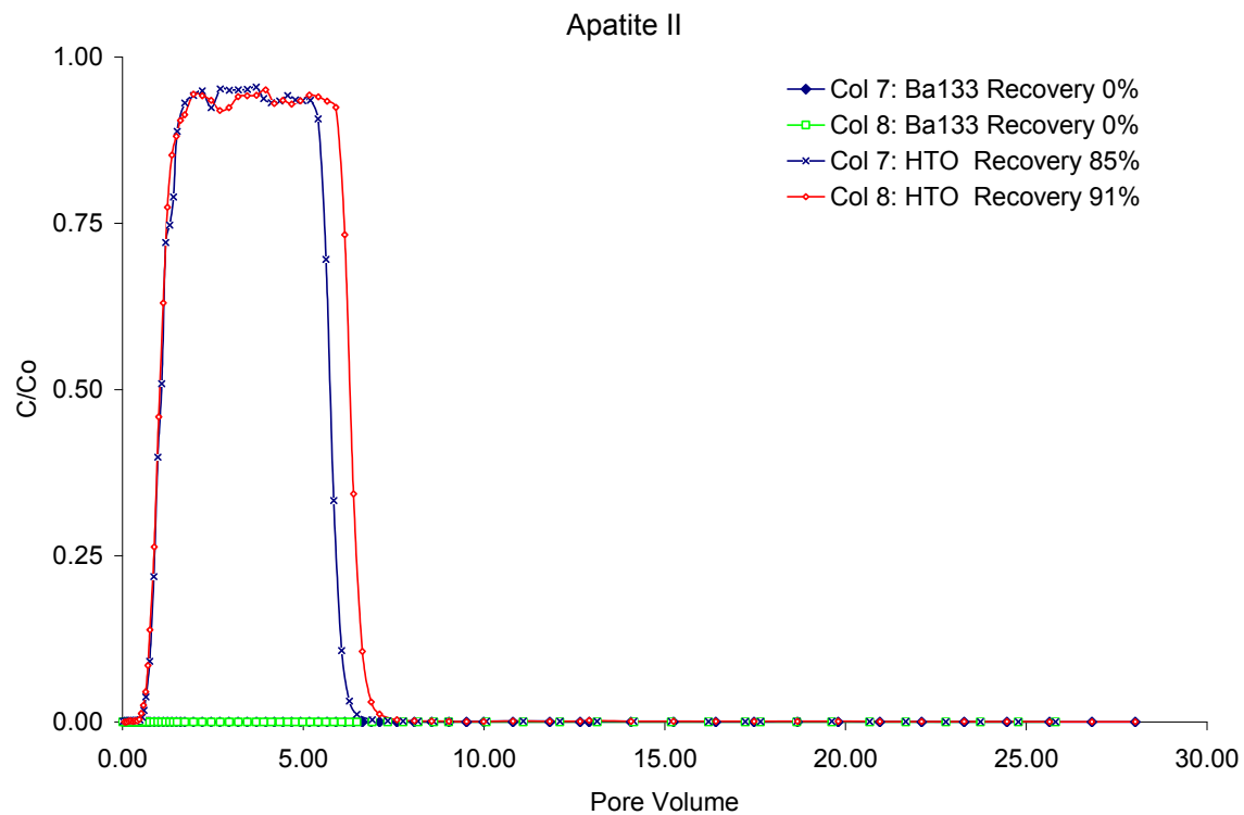
Figure B1-11 Breakthrough curves for apatite II columns
