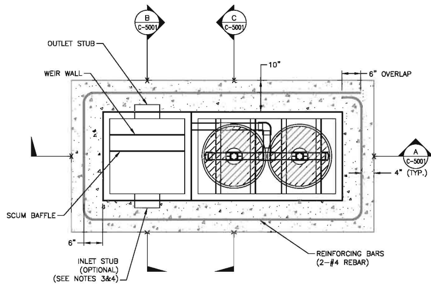
1 DETAIL CATCH BASIN FILTER-PLAN VIEW SCALE: NONE
