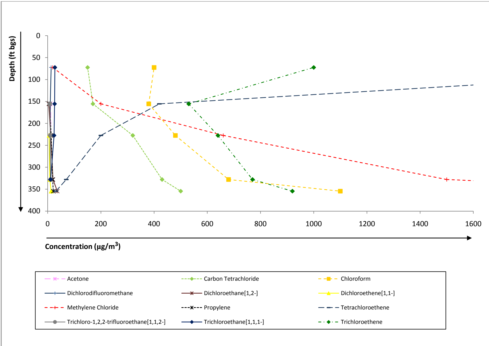
Figure 5.1-12 Vertical profile of detected VOCs in pore gas, monitoring well 21-25264, fourth quarter, September 2008
