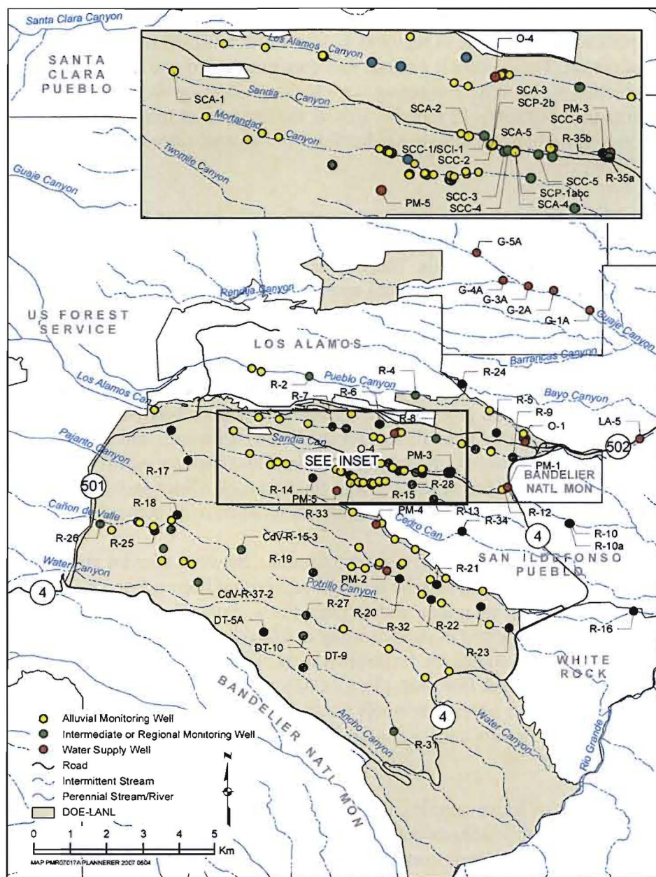
Figure 3-1. Alluvial, intermediate, and regional aquifer characterization wells within LANL and vicinity.
