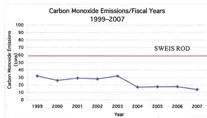
Figure 4-4. Carbon monoxide emissions for FY 1999–2007.
