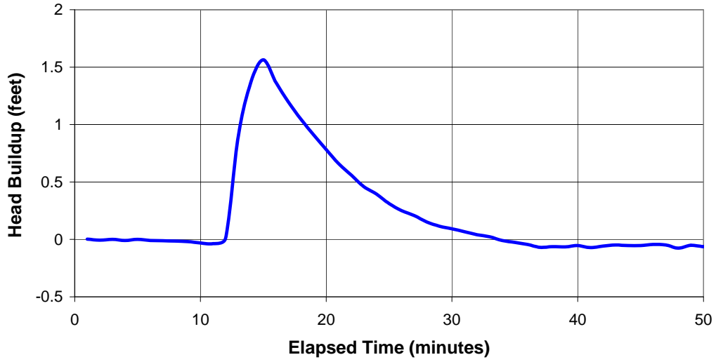
Figure E-4.4-7 Well R-37 screen 1 packer deflation following 24-h test
