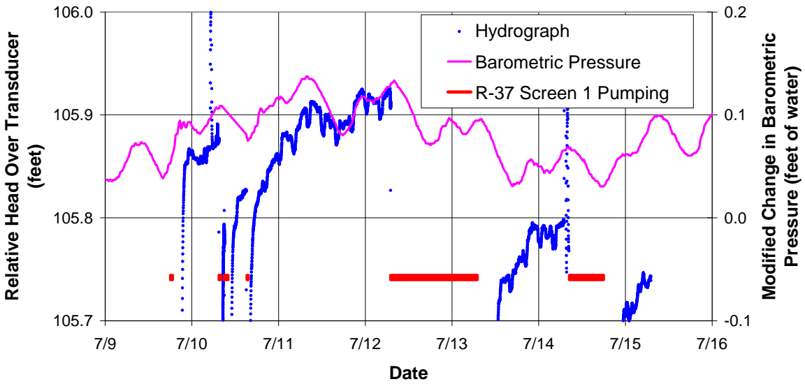
Figure E-4.1-2 R-37 screen 1 rolling average hydrograph and barometric pressure corrected for 62% efficiency
