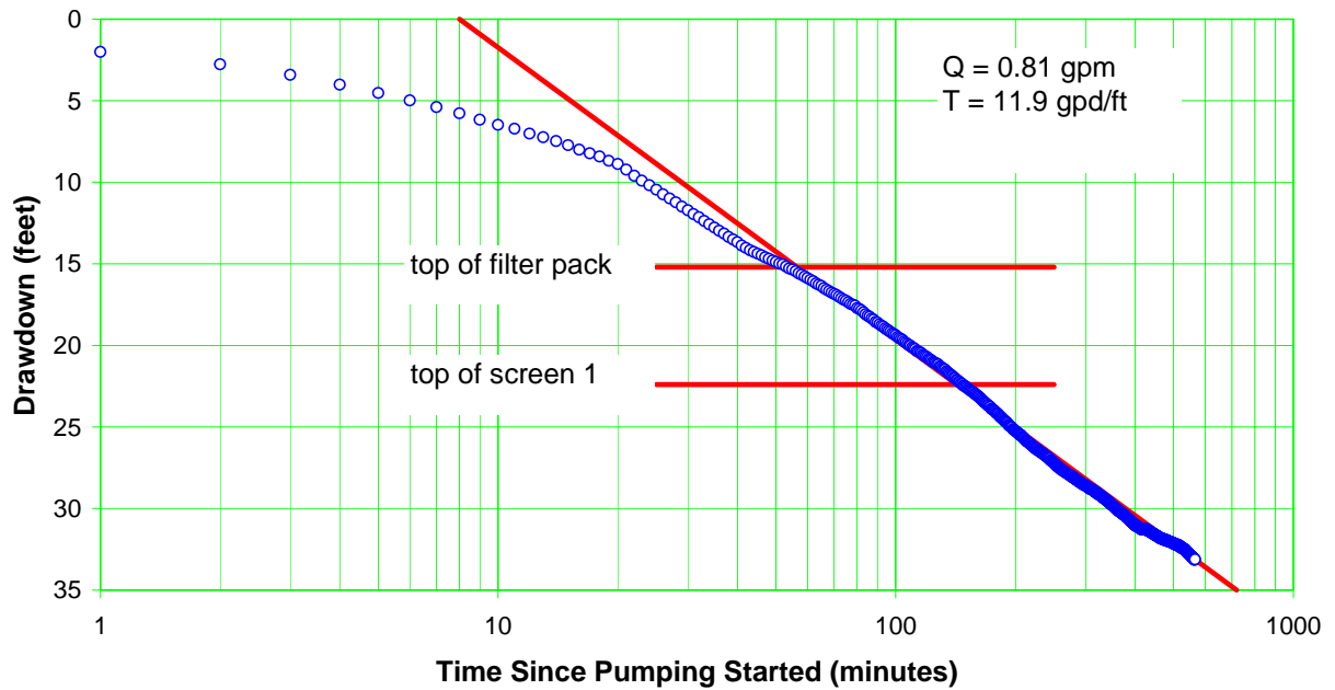
Figure E-4.5-1 Well R-37 screen 1 purge development drawdown
