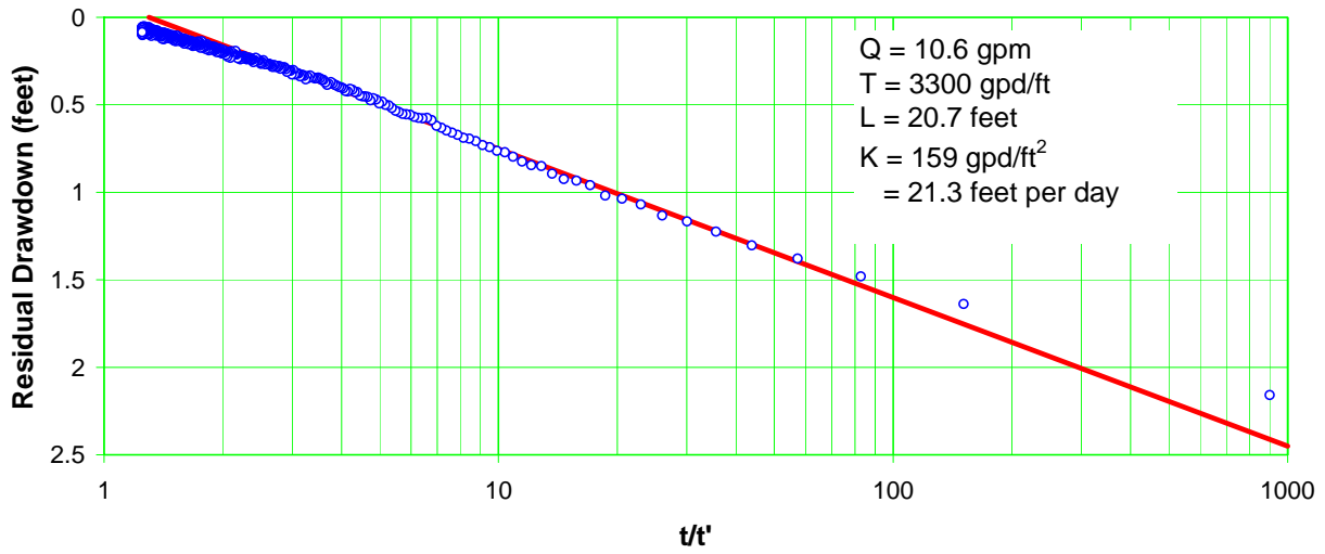
Figure E-5.2-1 Well R-37 screen 2 trial 1 recovery
