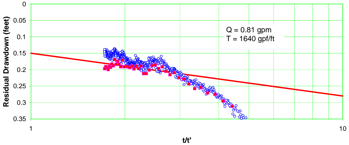
Figure E-4.5-6 Well R-37 screen 1 purge development recovery—corrected data
