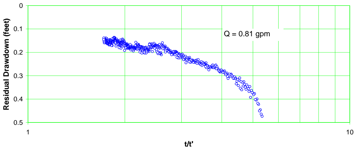
Figure E-4.5-5 Well R-37 screen 1 purge development recovery—expanded scale
