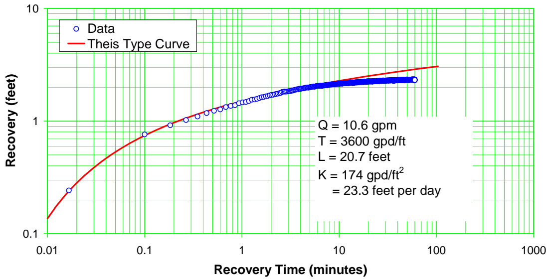
Figure E-5.2-2 Well R-37 screen 2 trial 1 recovery—Theis analysis
