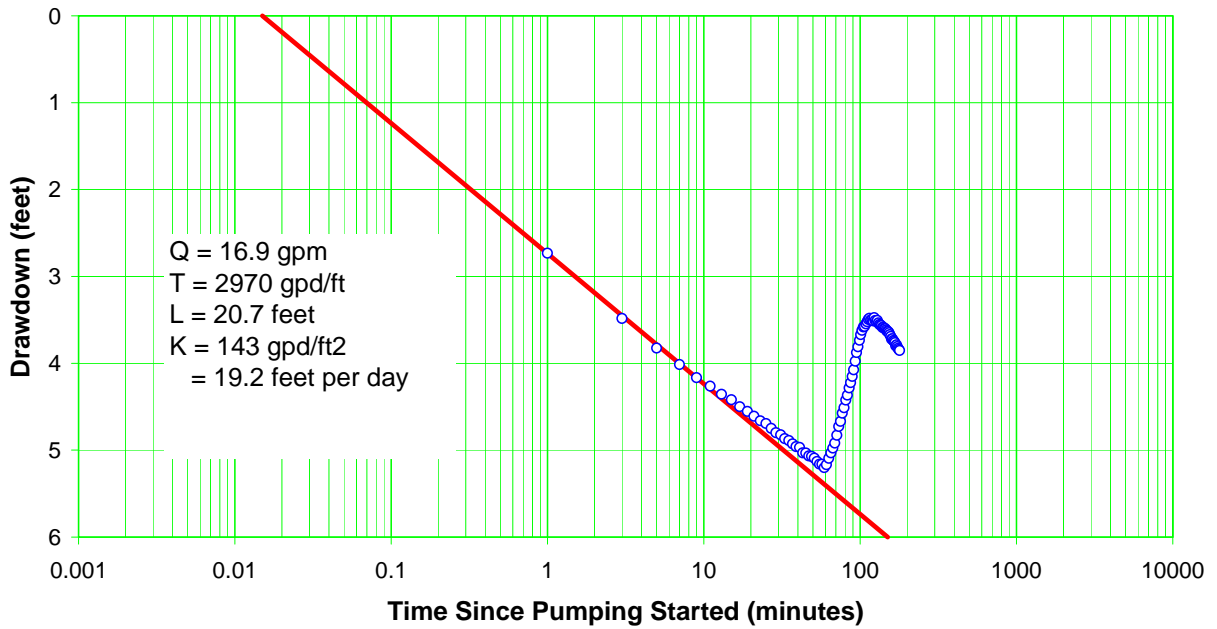
Figure E-5.5-1 Well R-37 screen 2 trial 3 drawdown
