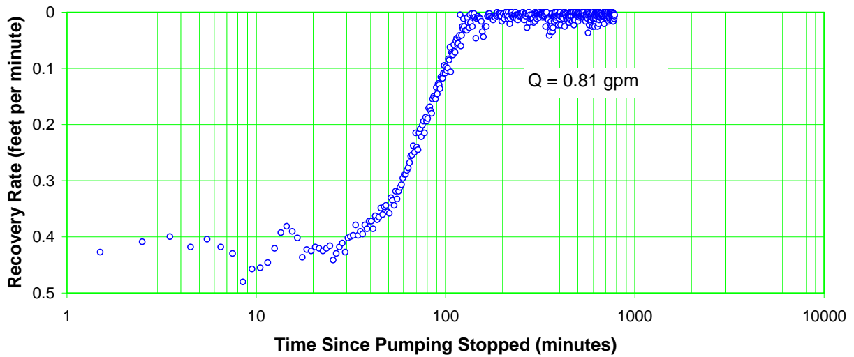
Figure E-4.5-3 Well R-37 screen 1 purge development calculated recovery rate
