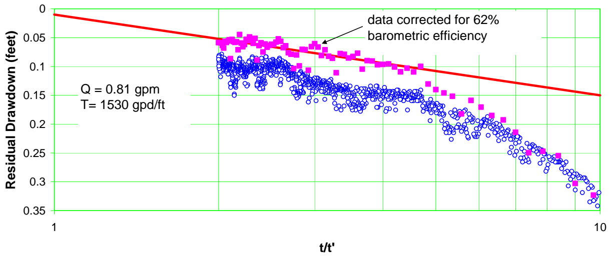
Figure E-4.4-6 Well R-37 screen 1 recovery—corrected data
