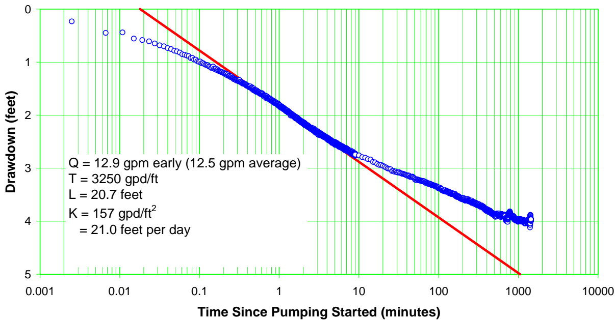
Figure E-5.4-1 Well R-37 screen 2 drawdown
