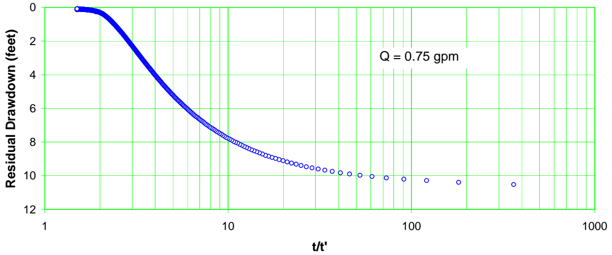
Figure E-4.2-2 Well R-37 screen 1 trial 1 recovery
