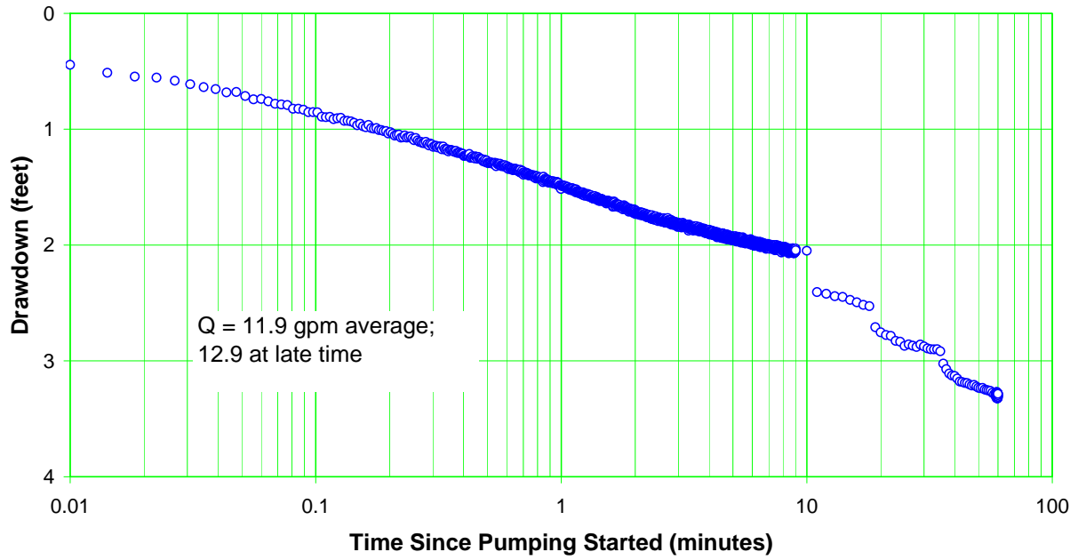
Figure E-5.3-1 Well R-37 screen 2 trial 2 drawdown
