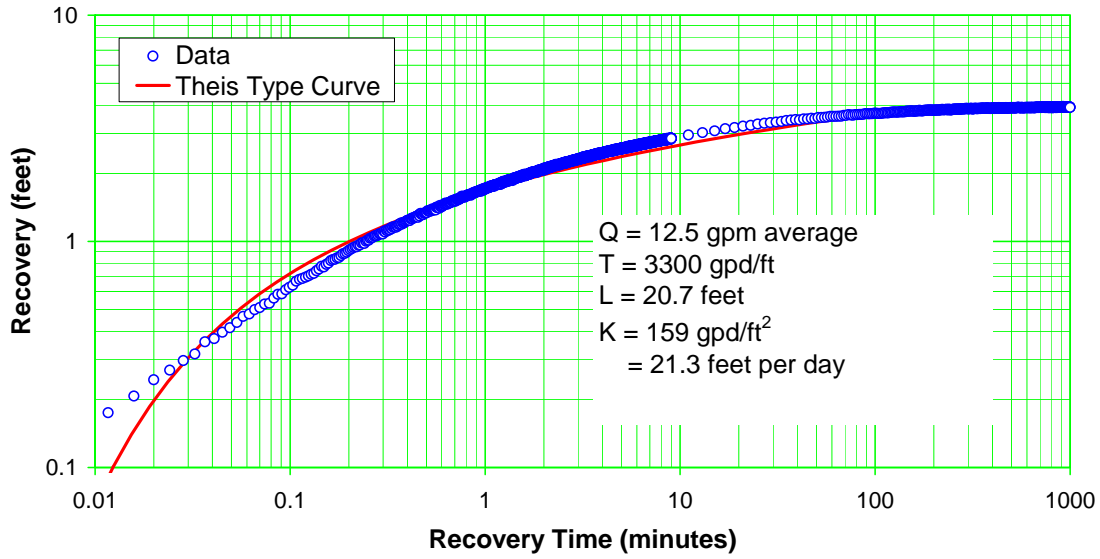
Figure E-5.4-4 Well R-37 screen 2 recovery—Theis analysis
