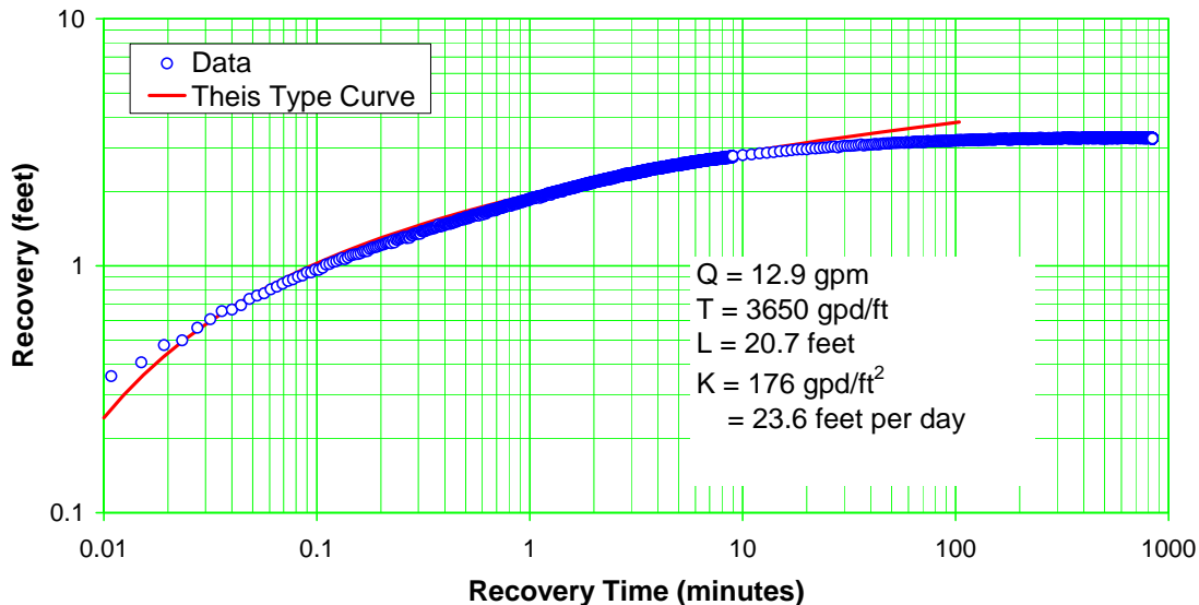
Figure E-5.3-3 Well R-37 screen 2 trial 2 recovery—Theis analysis
