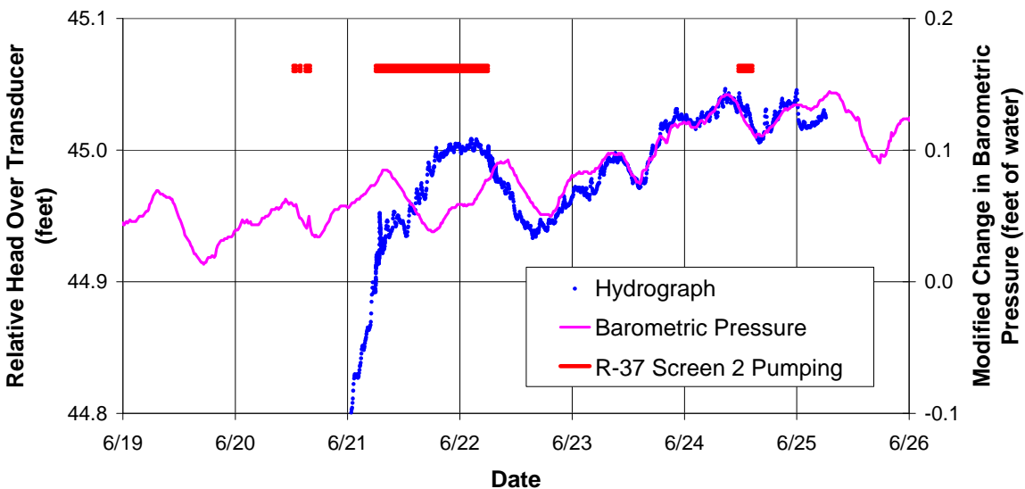
Figure E-4.1-4 R-37 screen 1 rolling average hydrograph during screen 2 pumping test and barometric pressure corrected for 62% efficiency
