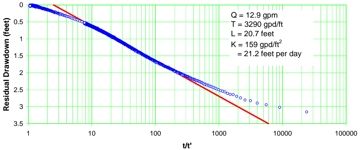
Figure E-5.3-2 Well R-37 screen 2 trial 2 recovery
