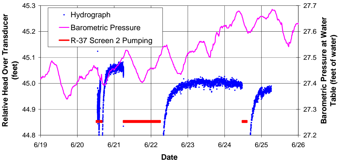
Figure E-5.1-1 Well R-37 screen 2 apparent hydrograph
