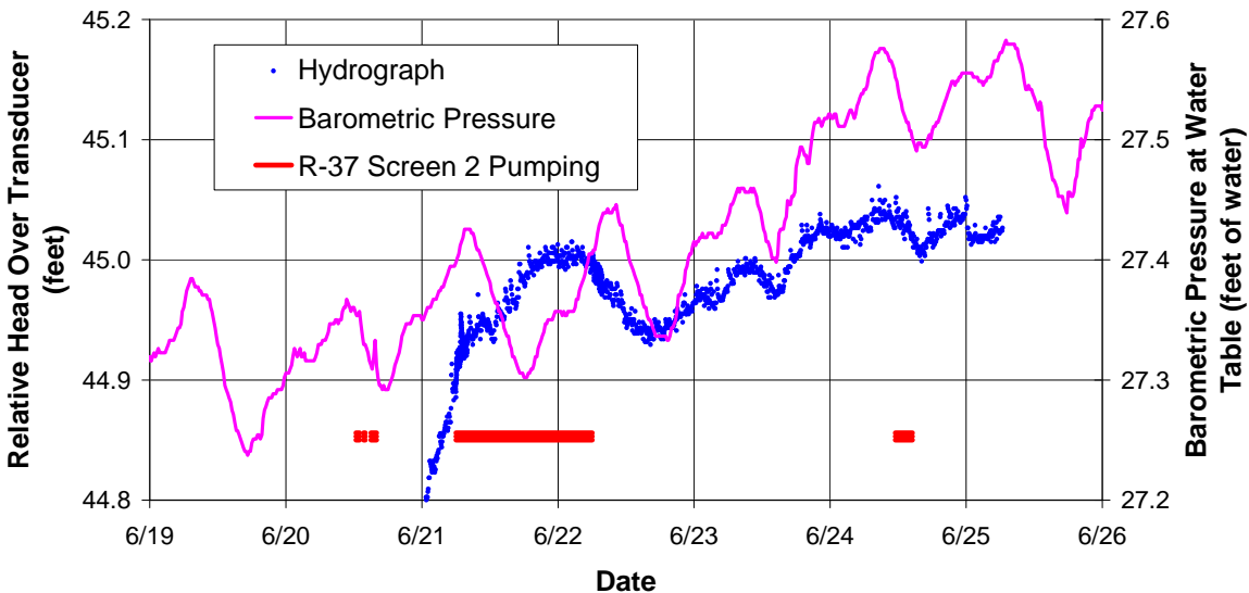
Figure E-4.1-3 R-37 screen 1 apparent hydrograph during screen 2 pumping test
