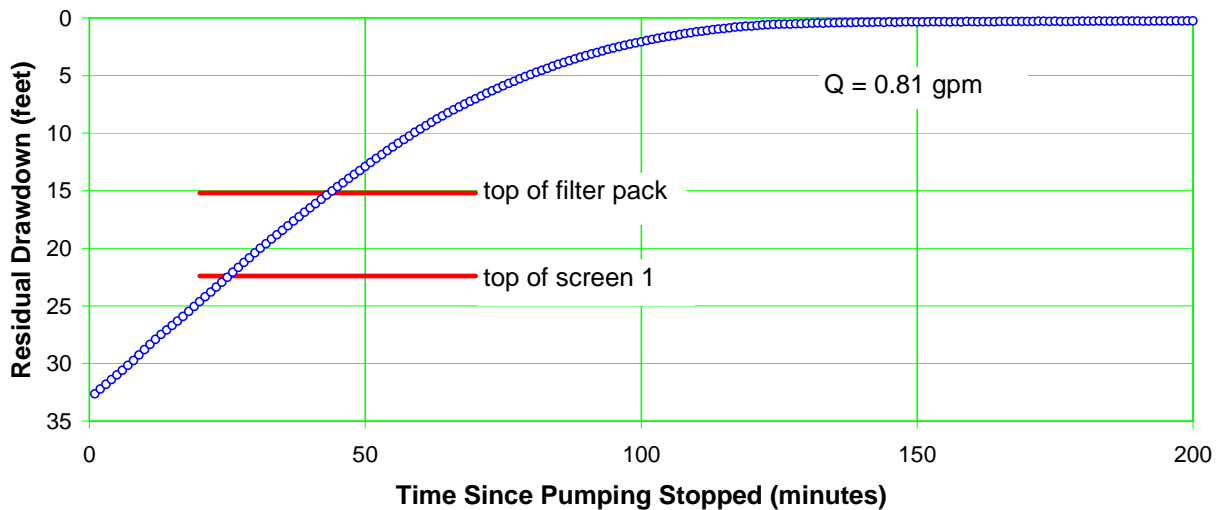
Figure E-4.5-4 Well R-37 screen 1 purge development recovery—linear plot
