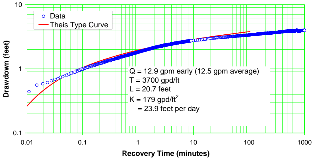
Figure E-5.4-2 Well R-37 screen 2 drawdown—This analysis
