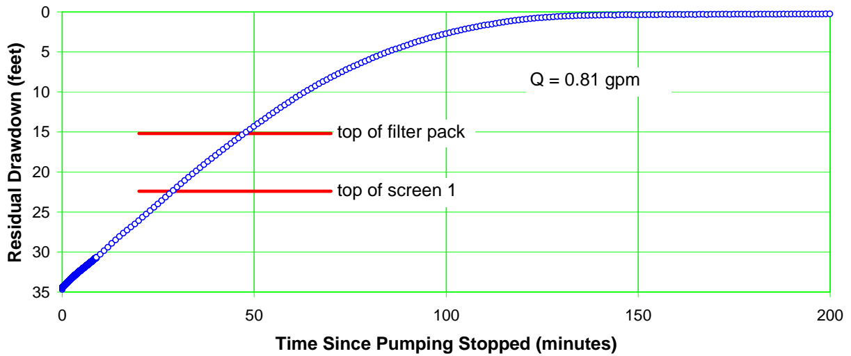
Figure E-4.4-4 Well R-37 screen 1 recovery—linear plot
