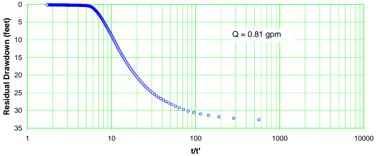
Figure E-4.5-2 Well R-37 screen 1 purge development recovery
