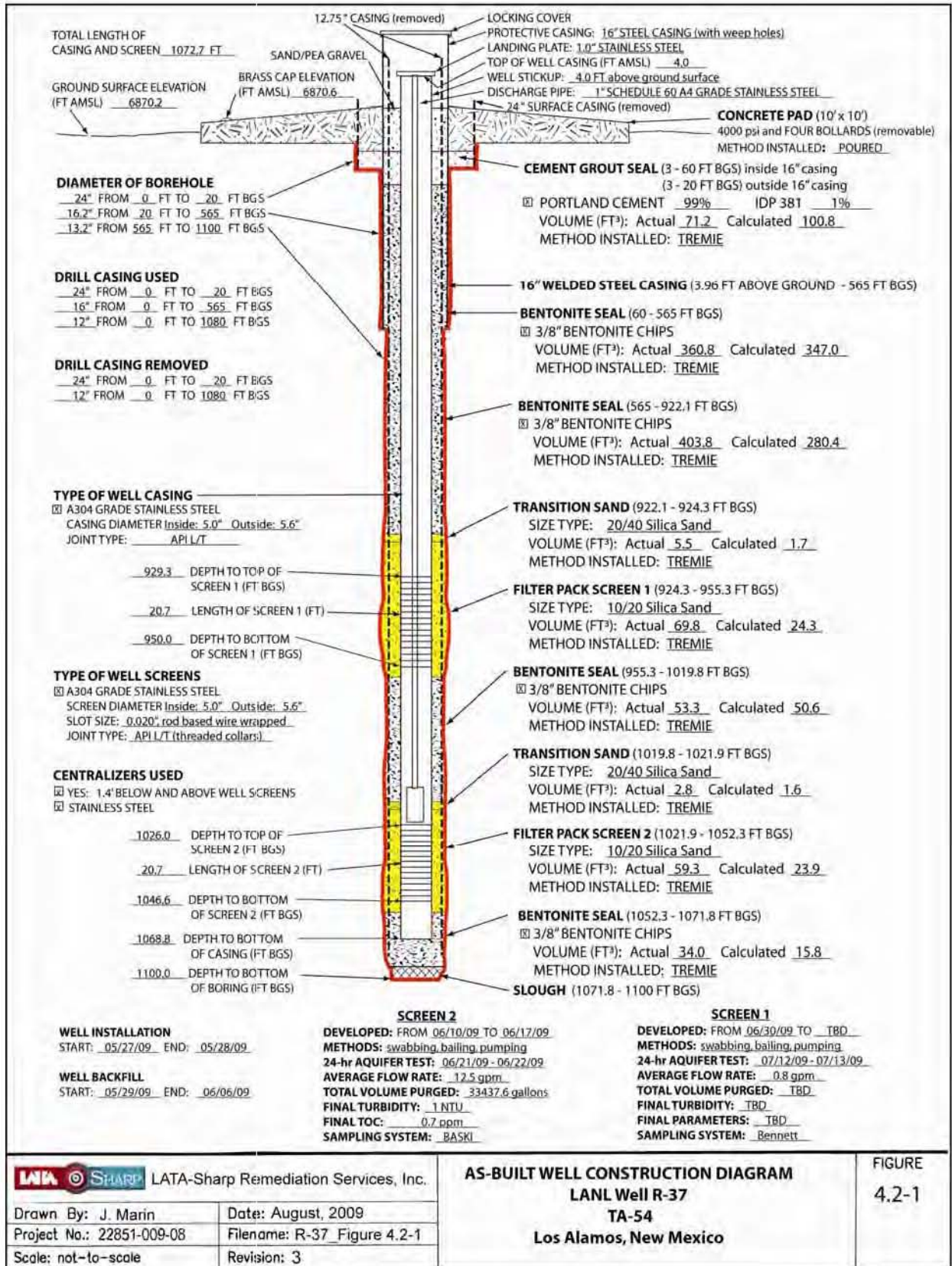
Figure 4.2-1 As-built well construction diagram
