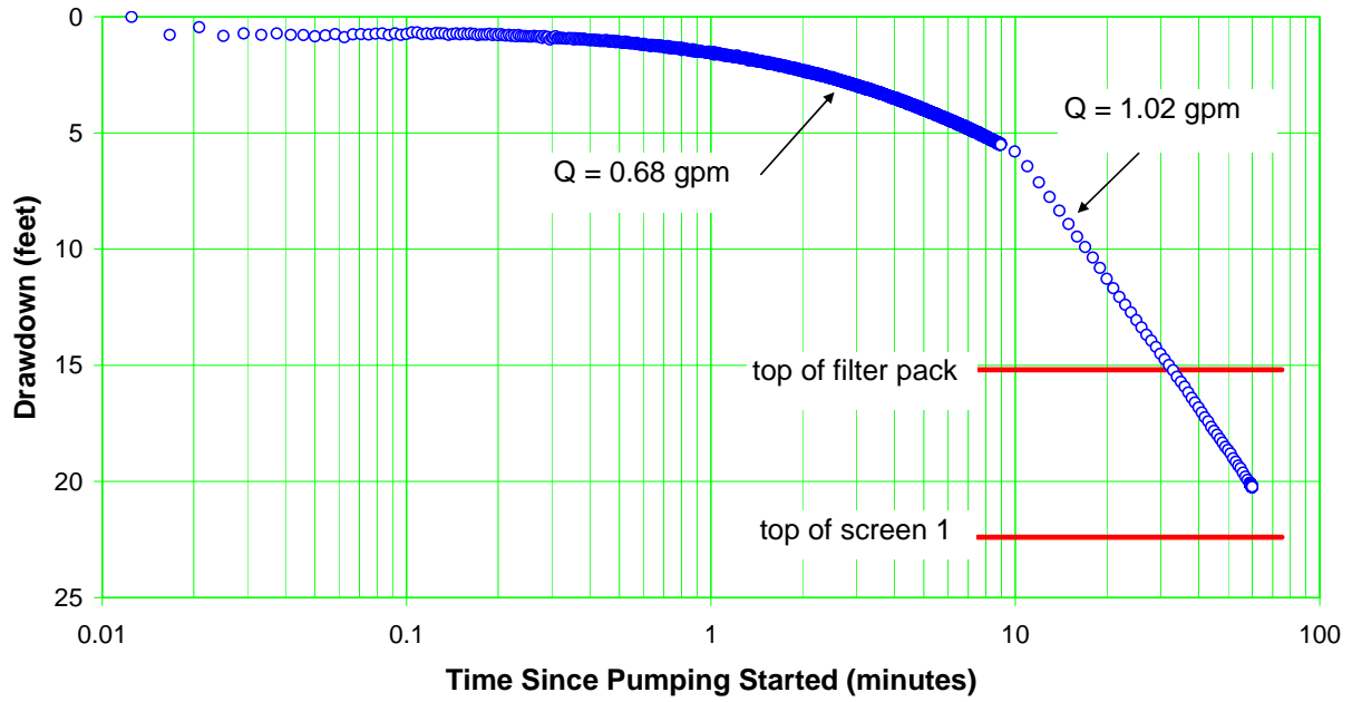
Figure E-4.3-1 Well R-37 screen 1 trial 2 drawdown
