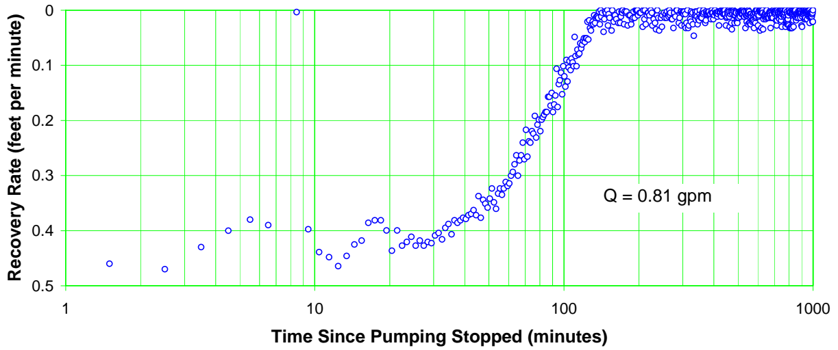
Figure E-4.4-3 Well R-37 screen 1 calculated recovery rate
