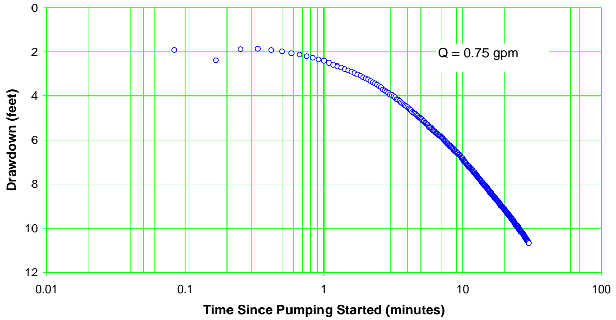
Figure E-4.2-1 Well R-37 screen 1 trial 1 drawdown
