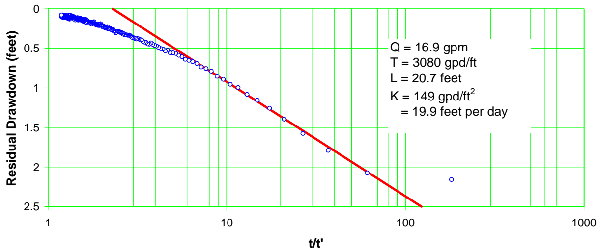
Figure E-5.5-2 Well R-37 screen 2 trial 3 recovery
