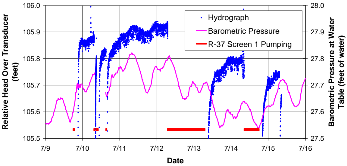
Figure E-4.1-1 R-37 screen 1 apparent hydrograph
