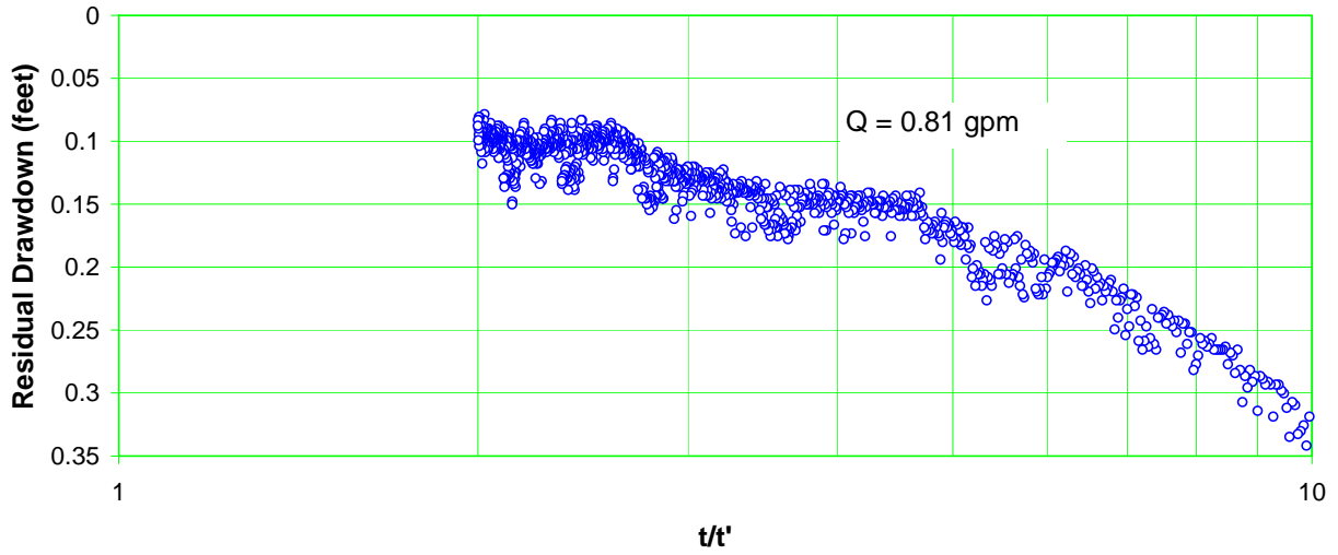
Figure E-4.4-5 Well R-37 screen 1 recovery—expanded scale
