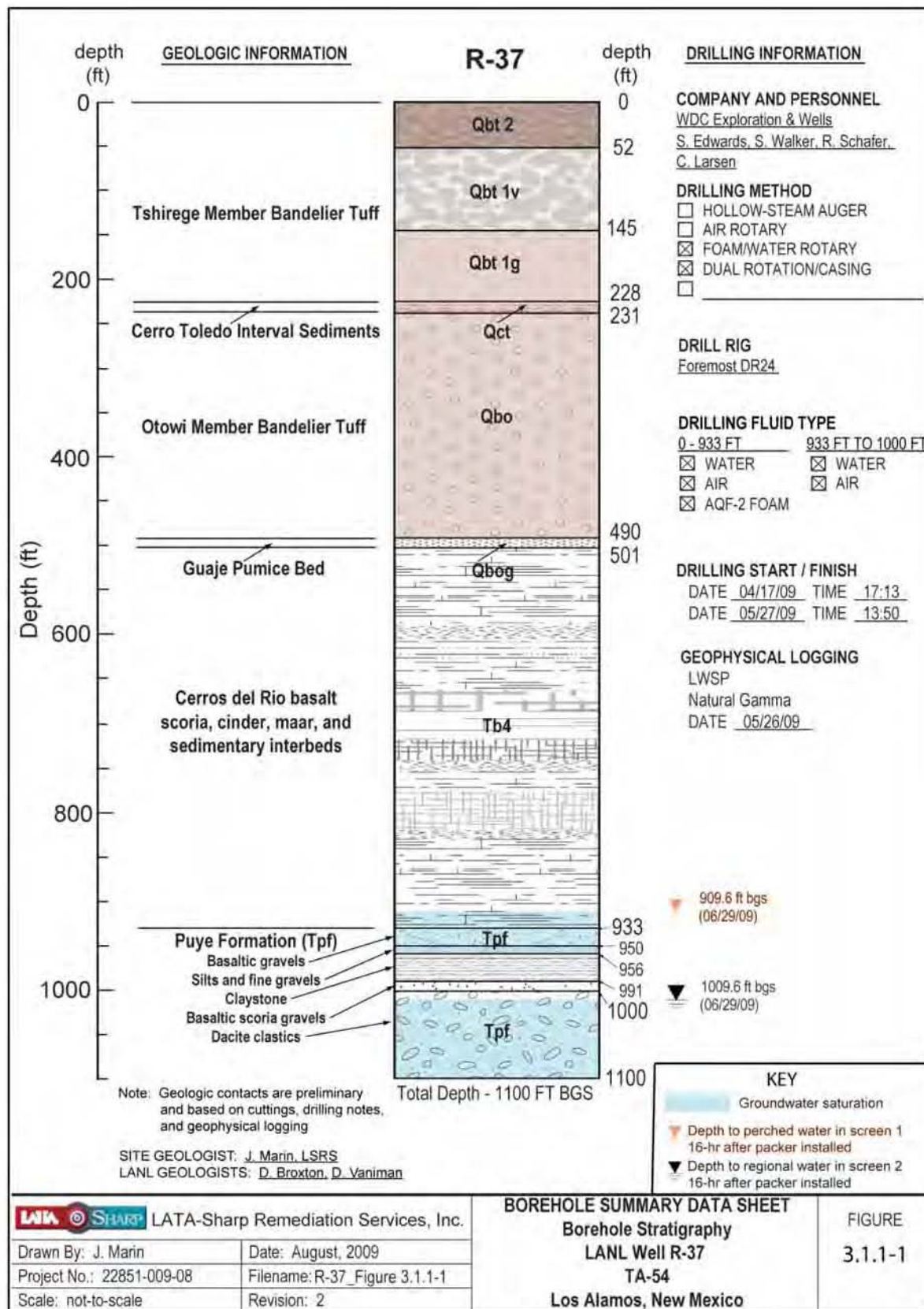
Figure 3.1-1 R-37 borehole summary data sheet
