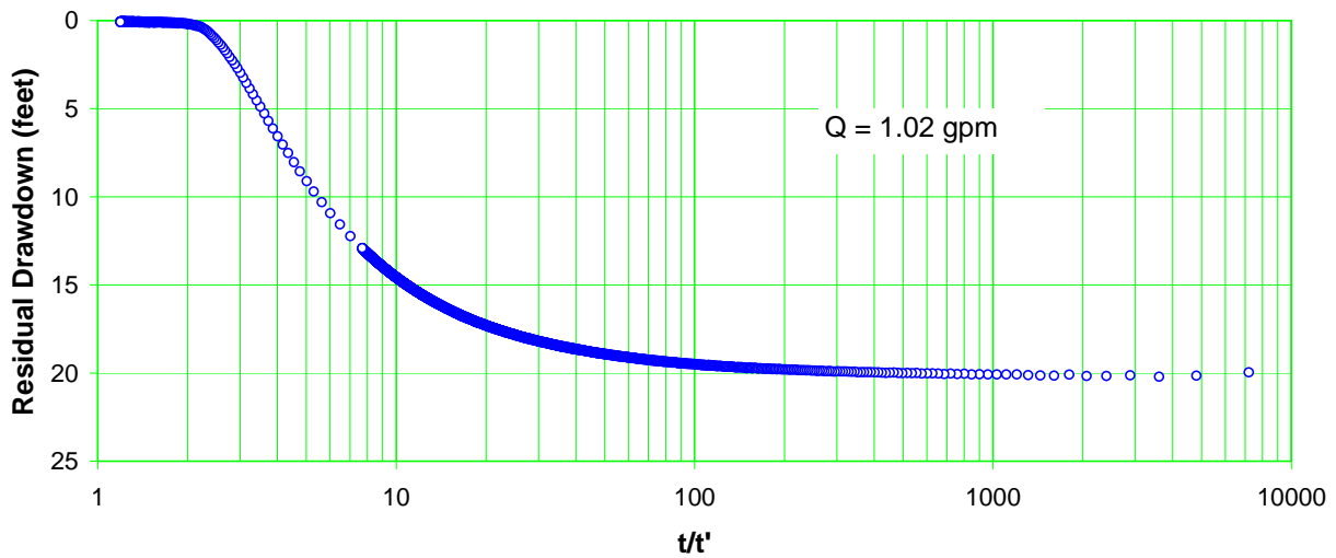
Figure E-4.3-2 Well R-37 screen 1 trial 2 recovery
