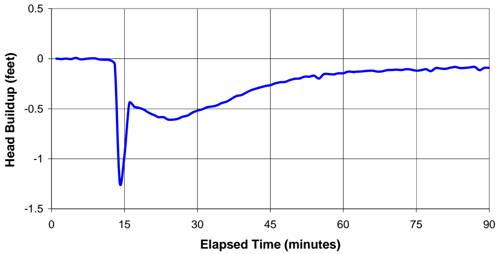
Figure E-4.5-7 Well R-37 screen 1 packer deflation following purge development
