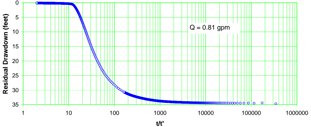
Figure E-4.4-2 Well R-37 screen 1 recovery
