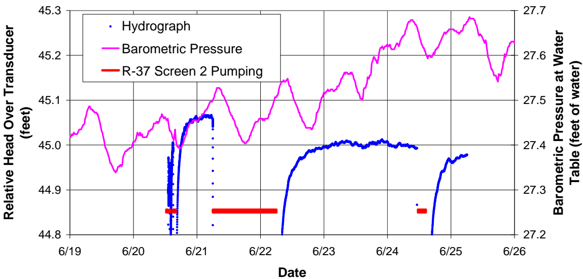
Figure E-5.1-2 Well R-37 screen 2 apparent hydrograph—rolling average
