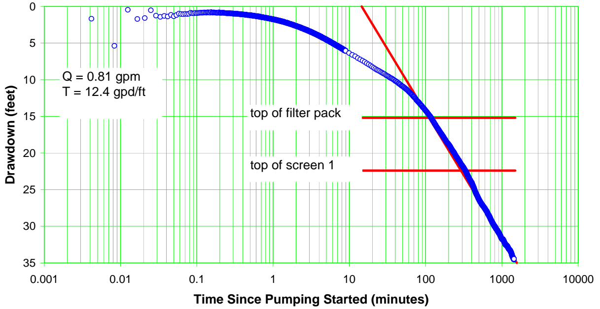
Figure E-4.4-1 Well R-37 screen 1 drawdown
