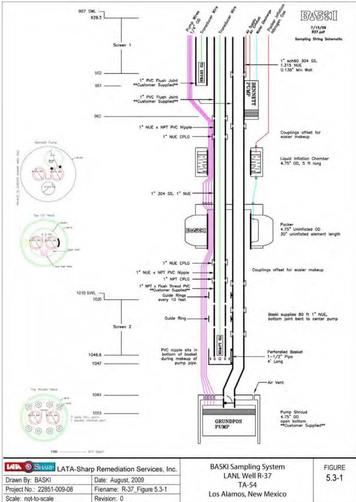
Figure 5.3-1 As-built completion schematic for regional aquifer well R-37
