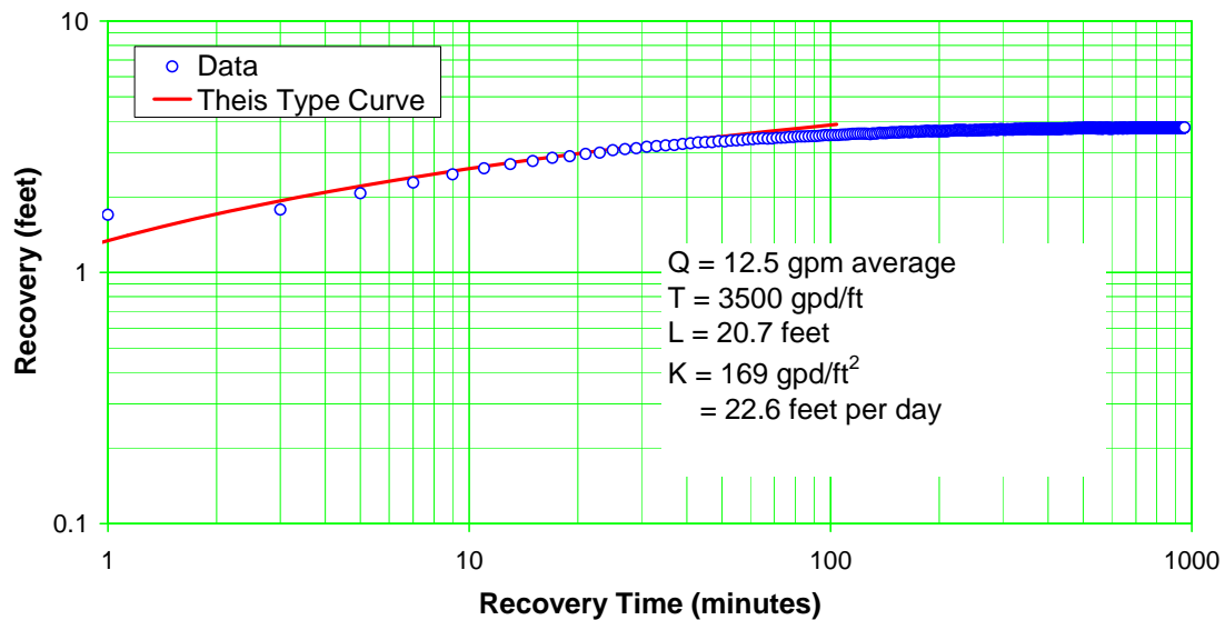
Figure E-5.5-3 Well R-37 screen 2 trial 3 recovery—Theis analysis
