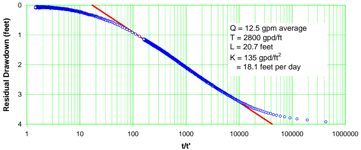
Figure E-5.4-3 Well R-37 screen 2 recovery
