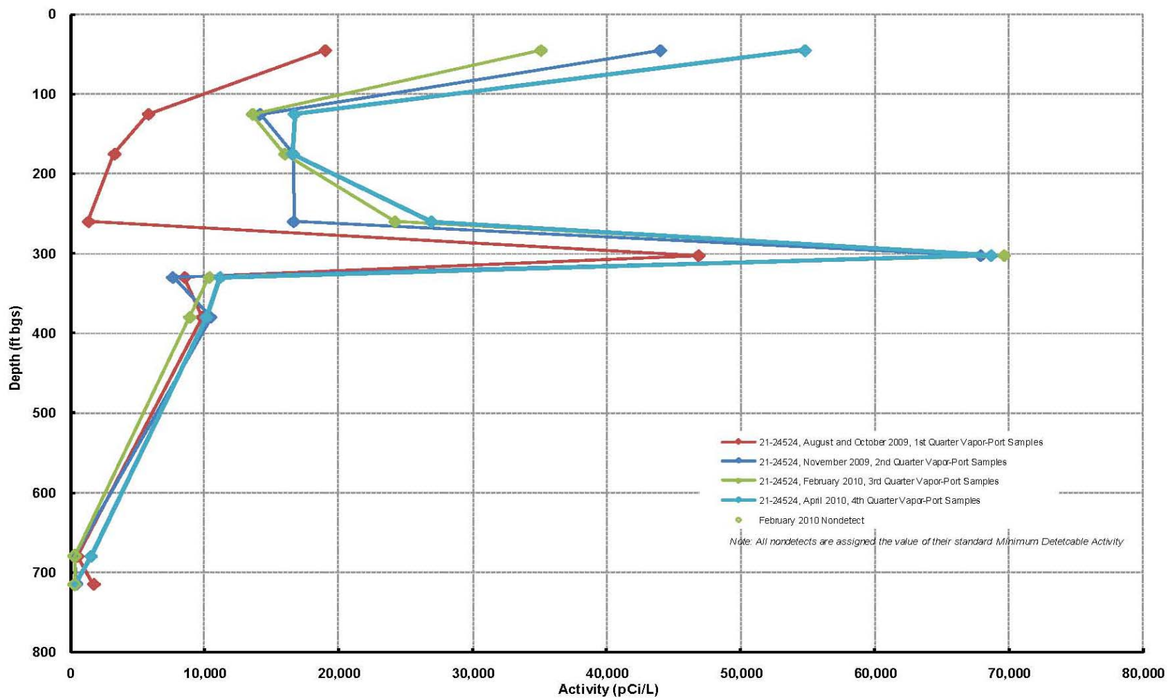
Figure 5.1-1 Vertical profile of tritium vapor-port samples from vapor-monitoring wells 21-24524W and 21-24524S, August 2009–April 2010
